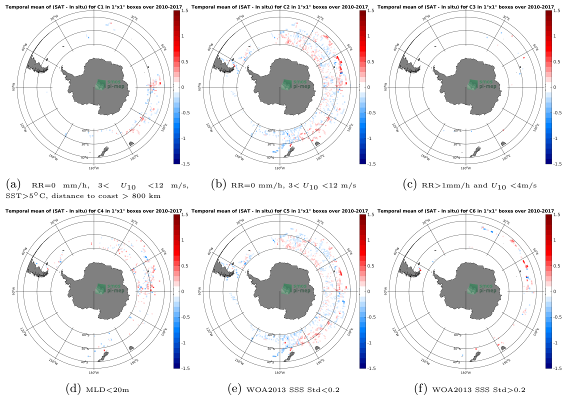
Figure 12: Temporal mean gridded over spatial boxes of size 1^{\circ}\times 1^{\circ} of \Delta\text{SSS} (CCI L4 Merged-OI v1.8 - 7-day running (ESA) - Sea mammals) for 6 different subdatasets corresponding to:RR=0 mm/h, 3 < U_{10} < 12 m/s, SST >5^{\circ}\text{C} , distance to coast > 800 km (a), RR=0 mm/h, 3 < U_{10} < 12 m/s (b), RR >1 mm/h and U_{10} < 4 m/s (c),MLD <20 m (d),WOA2013 SSS Std <0.2 (e),WOA2013 SSS Std >0.2 (f).
