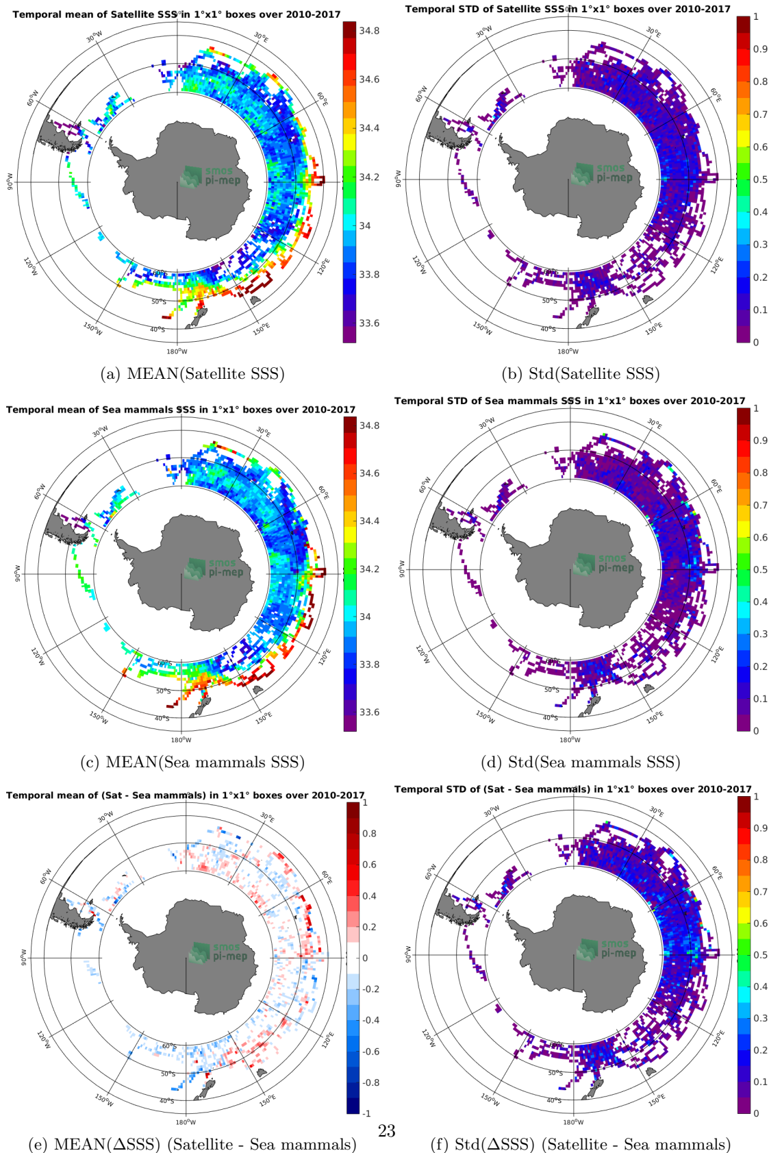
Figure 6: Temporal mean (left) and Std (right) of SSS from CCI L4 Merged-OI v1.8 - 7-day running (ESA) (top), Sea mammals (middle), and of \Delta SSS (Satellite - Sea mammals). Only match-up pairs are used to generate these maps.
