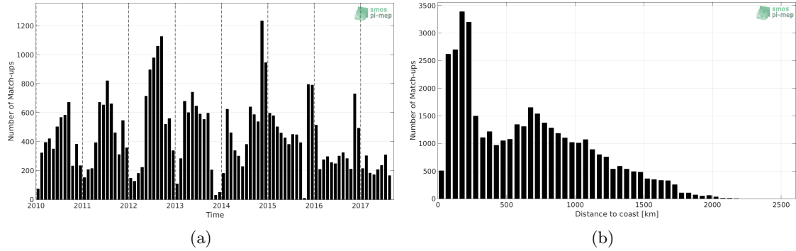
Figure 1: Number of match-ups between Sea mammals and CCI L4 Merged-OI v1.8 - 7-day running (ESA) SSS as a function of time (a) and as function of the distance to coast (b) over the Roaring Forties and Furious Fifties Pi-MEP region and for the full satellite product period.
