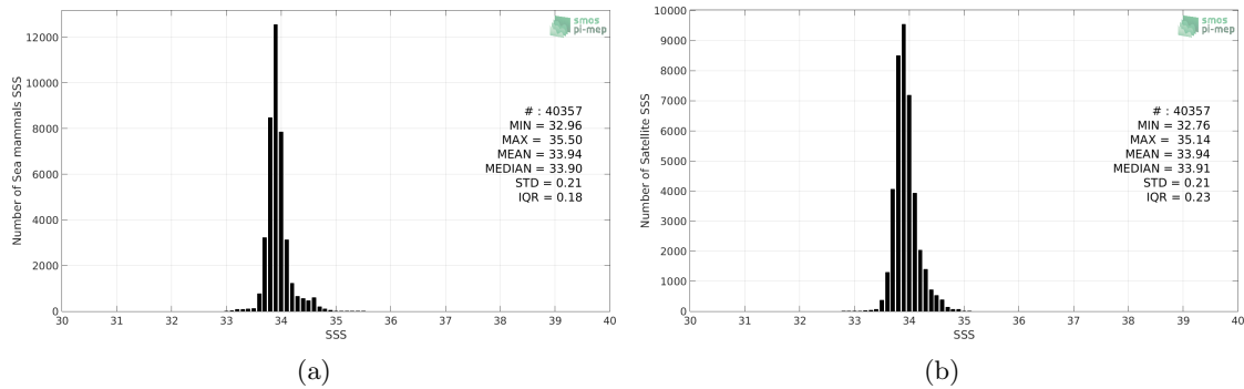
Figure 2: Histograms of SSS from Sea mammals (a) and CCI L4 Merged-OI v1.8 - 7-day running (ESA) (b) considering all match-up pairs per bins of 0.1 over the Roaring Forties and Furious Fifties Pi-MEP region and for the full satellite product period.
