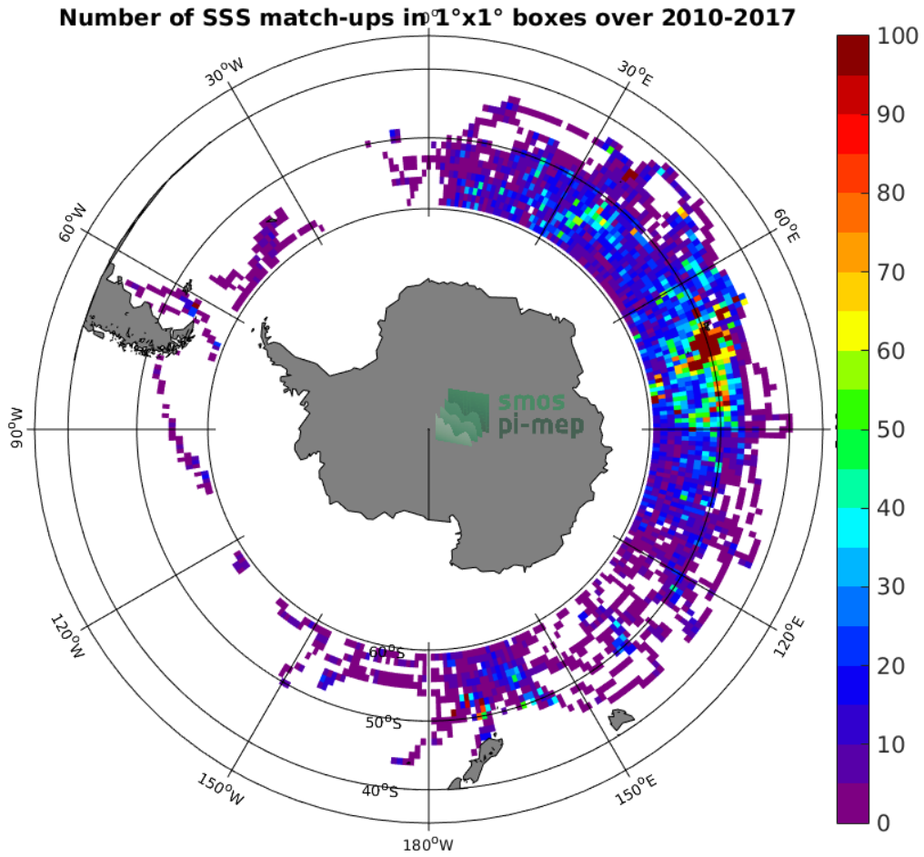
Figure 4: Number of SSS match-ups between Sea mammals SSS and the CCI L4 Merged-OI v1.8 - 7-day running (ESA) SSS product for the Roaring Forties and Furious Fifties Pi-MEP region over 1°x1° boxes and for the full satellite product period.
