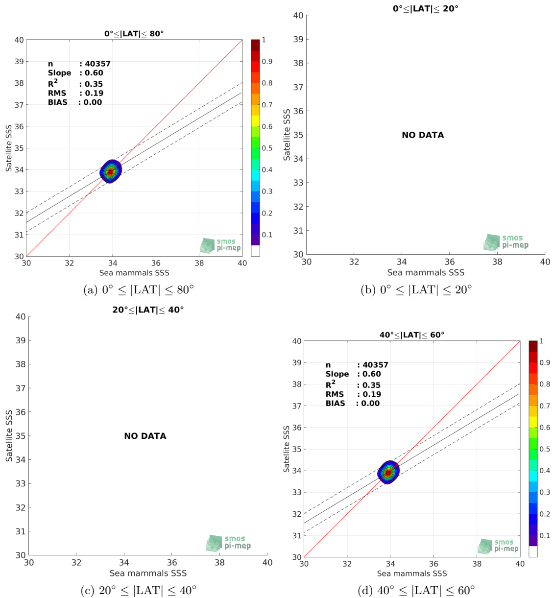
Figure 9: Contour maps of the concentration of CCI L4 Merged-OI v1.8 - 7-day running (ESA) SSS (y-axis) versus Sea mammals SSS (x-axis) at match-up pairs for different latitude bands. For each plot, the red line shows x=y . The black thin and dashed lines indicate a linear fit through the data cloud and the \pm 95\% confidence levels, respectively. The number match-up pairs n , the slope and R^2 coefficient of the linear fit, the root mean square (RMS) and the mean bias between satellite and in situ data are indicated for each latitude band in each plots.
