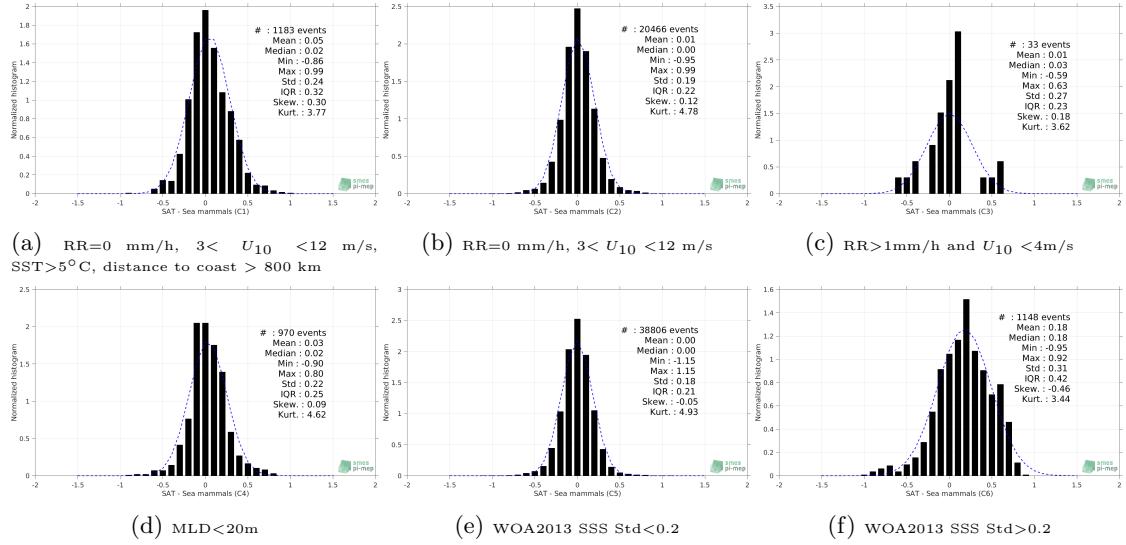
Figure 13: Normalized histogram of \Delta SSS (CCI L4 Merged-OI v1.8 - 7-day running (ESA) - Sea mammals) for 6 different subdatasets corresponding to: RR=0 mm/h, 3 < U_{10} < 12 m/s, SST>5°C, distance to coast > 800 km (a), RR=0 mm/h, 3 < U_{10} < 12 m/s (b), RR>1mm/h and U_{10} < 4 m/s (c), MLD<20m (d), WOA2013 SSS Std<0.2 (e), WOA2013 SSS Std>0.2 (f).
