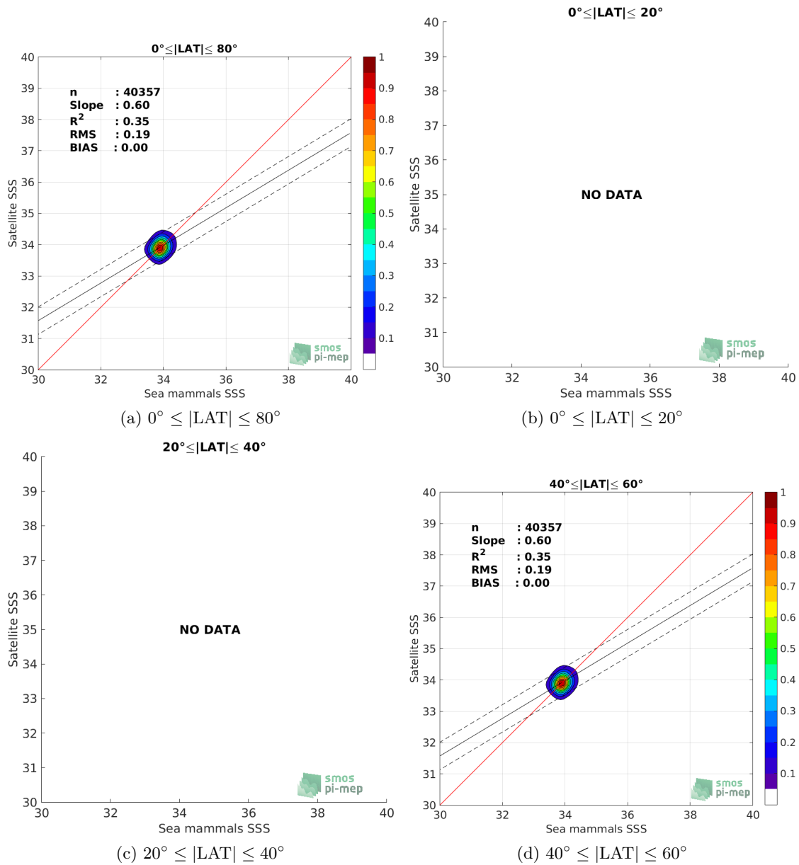
Figure 9: Contour maps of the concentration of CCI-L4-ESA-MERGED-OI-V1.8-7DAY-RUNNING SSS (y-axis) versus Sea mammals SSS (x-axis) at match-up pairs for different latitude bands. For each plot, the red line shows x=y . The black thin and dashed lines indicate a linear fit through the data cloud and the \pm 95\% confidence levels, respectively. The number match-up pairs n , the slope and R^2 coefficient of the linear fit, the root mean square (RMS) and the mean bias between satellite and in situ data are indicated for each latitude band in each plots.
