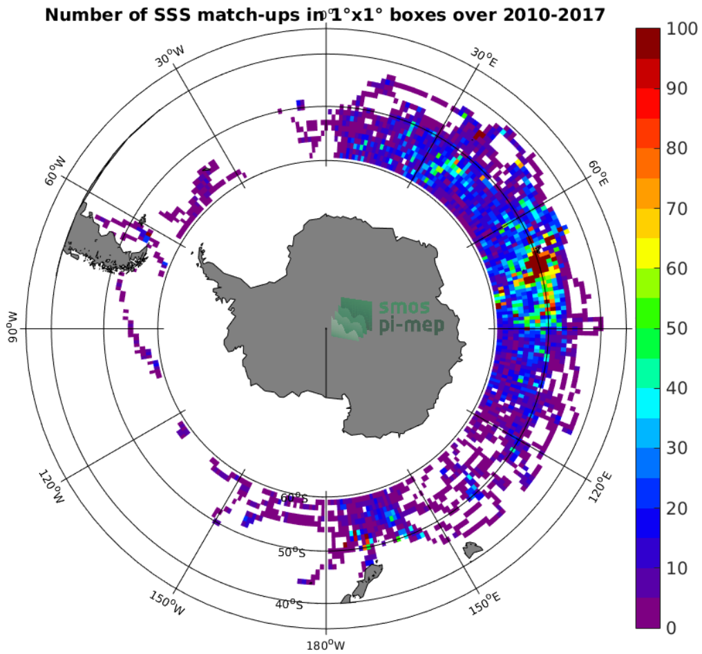
Figure 4: Number of SSS match-ups between Sea mammals SSS and the CCI-L4-ESA-MERGED-OI-V1.8-7DAY-RUNNING SSS product for the Roaring Forties and Furious Fifties Pi-MEP region over 1°x1° boxes and for the full satellite product period.
