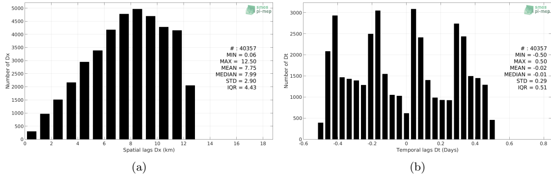
Figure 5: Histograms of the spatial (a) and temporal (b) lags between the time of the Sea mammals measurements and the date of the corresponding CCI-L4-ESA-MERGED-OI-V1.8-7DAY-RUNNING SSS product.
