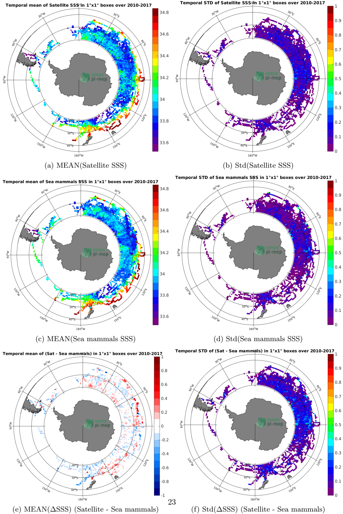
Figure 6: Temporal mean (left) and Std (right) of SSS from CCI-L4-ESA-MERGED-OI-V1.8-7DAY-RUNNING (top), Sea mammals (middle), and of \Delta SSS (Satellite - Sea mammals). Only match-up pairs are used to generate these maps.
