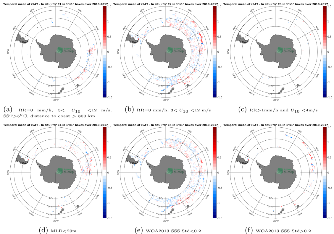
Figure 12: Temporal mean gridded over spatial boxes of size 1^\circ \times 1^\circ of \Delta SSS (CCI-L4-ESAMERGED-OI-V1.8-7DAY-RUNNING - Sea mammals) for 6 different subdatasets corresponding to:RR=0 mm/h, 3 < U_{10} < 12 m/s, SST >5^\circ C, distance to coast > 800 km (a), RR=0 mm/h, 3 < U_{10} < 12 m/s (b), RR >1 mm/h and U_{10} < 4 m/s (c),MLD <20 m (d),WOA2013 SSS Std <0.2 (e),WOA2013 SSS Std >0.2 (f).
