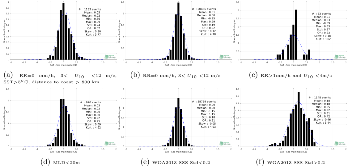
Figure 13: Normalized histogram of \Delta SSS (CCI-L4-ESA-MERGED-OI-V1.8-7DAY-RUNNING - Sea mammals) for 6 different subdatasets corresponding to: RR=0 mm/h, 3 < U_{10} < 12 m/s, SST>5°C, distance to coast > 800 km (a), RR=0 mm/h, 3 < U_{10} < 12 m/s (b), RR>1mm/h and U_{10} < 4 m/s (c), MLD<20m (d), WOA2013 SSS Std<0.2 (e), WOA2013 SSS Std>0.2 (f).
