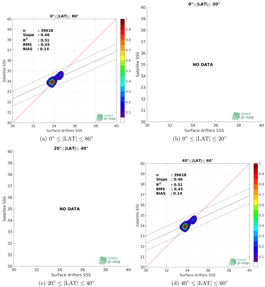
Figure 8: Contour maps of the concentration of CCI-L4-ESA-MERGED-OI-V1.8-7DAY-RUNNING SSS (y-axis) versus Surface drifters SSS (x-axis) at match-up pairs for different latitude bands. For each plot, the red line shows x=y . The black thin and dashed lines indicate a linear fit through the data cloud and the \pm 95\% confidence levels, respectively. The number match-up pairs n , the slope and R^2 coefficient of the linear fit, the root mean square (RMS) and the mean bias between satellite and in situ data are indicated for each latitude band in each plots.
