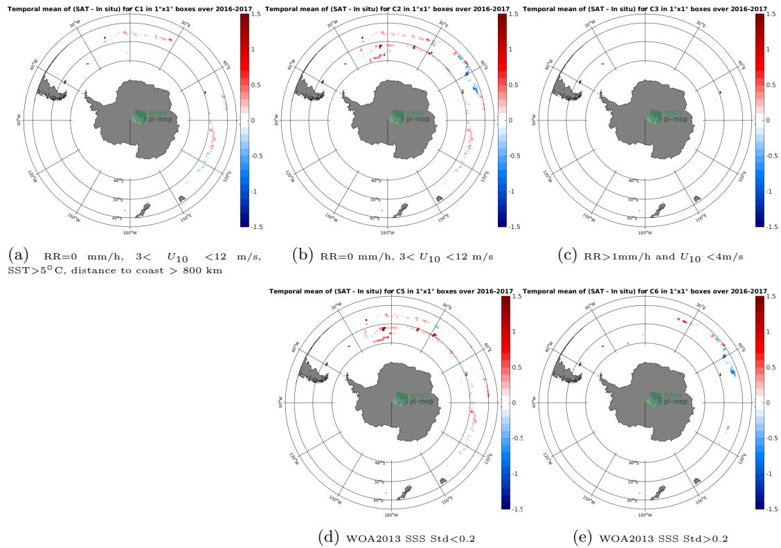
Figure 11: Temporal mean gridded over spatial boxes of size 1°x1° of \Delta SSS (CCI-L4-ESAMERGED-OI-V1.8-7DAY-RUNNING - Surface drifters) for 5 different subdatasets corresponding to:RR=0 mm/h, 3 < U_{10} < 12 m/s, SST>5°C, distance to coast > 800 km (a), RR=0 mm/h, 3 < U_{10} < 12 m/s (b), RR>1mm/h and U_{10} < 4 m/s (c), WOA2013 SSS Std<0.2 (d), WOA2013 SSS Std>0.2 (e).
