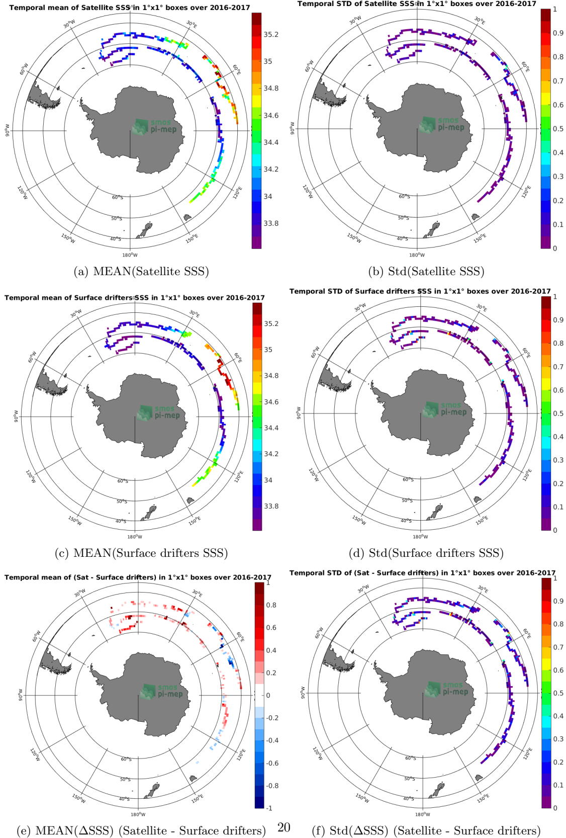
Figure 5: Temporal mean (left) and Std (right) of SSS from CCI-L4-ESA-MERGED-OI-V1.8-7DAY-RUNNING (top), Surface drifters (middle), and of \Delta SSS (Satellite - Surface drifters). Only match-up pairs are used to generate these maps.
