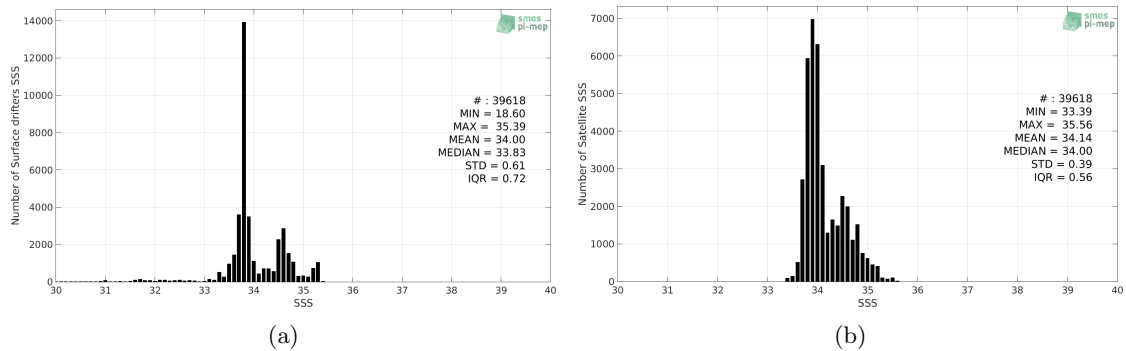
Figure 2: Histograms of SSS from Surface drifters (a) and CCI-L4-ESA-MERGED-OI-V1.8-7DAY-RUNNING (b) considering all match-up pairs per bins of 0.1 over the Roaring Forties and Furious Fifties Pi-MEP region and for the full satellite product period.
