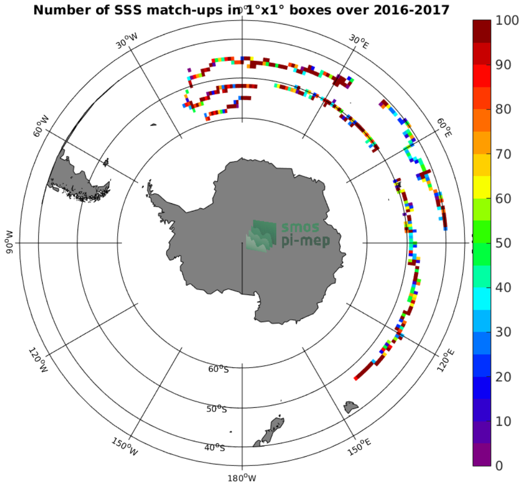
Figure 3: Number of SSS match-ups between Surface drifters SSS and the CCI-L4-ESA-MERGED-OI-V1.8-7DAY-RUNNING SSS product for the Roaring Forties and Furious Fifties Pi-MEP region over 1°x1° boxes and for the full satellite product period.
