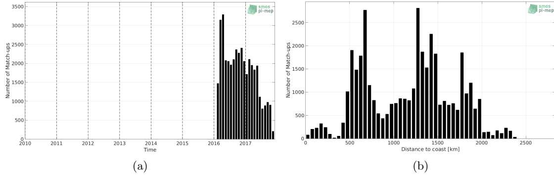
Figure 1: Number of match-ups between Surface drifters and CCI-L4-ESA-MERGED-OI-V1.8-7DAY-RUNNING SSS as a function of time (a) and as function of the distance to coast (b) over the Roaring Forties and Furious Fifties Pi-MEP region and for the full satellite product period.
