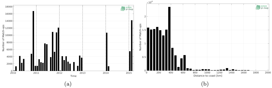
Figure 1: Number of match-ups between TSG-SAMOS and CCI L4 Merged-OI v1.8 - 30-day running (ESA) SSS as a function of time (a) and as function of the distance to coast (b) over the Roaring Forties and Furious Fifties Pi-MEP region and for the full satellite product period.
