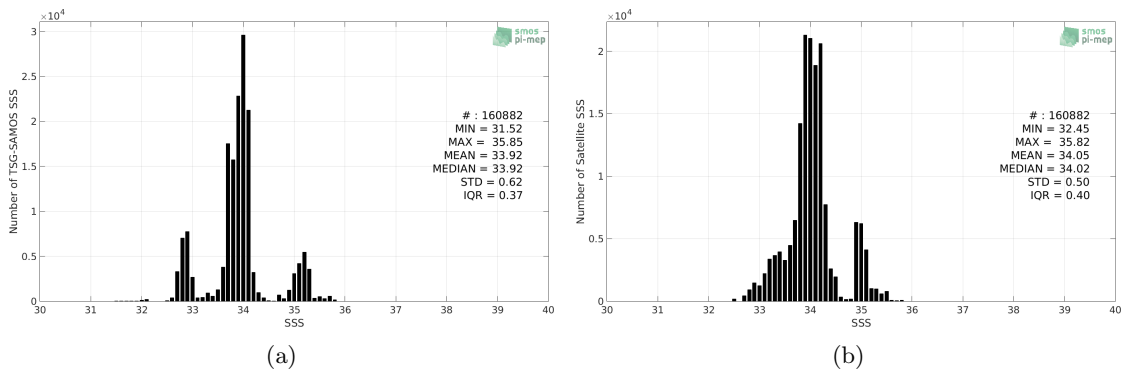
Figure 2: Histograms of SSS from TSG-SAMOS (a) and CCI L4 Merged-OI v1.8 - 30-day running (ESA) (b) considering all match-up pairs per bins of 0.1 over the Roaring Forties and Furious Fifties Pi-MEP region and for the full satellite product period.
