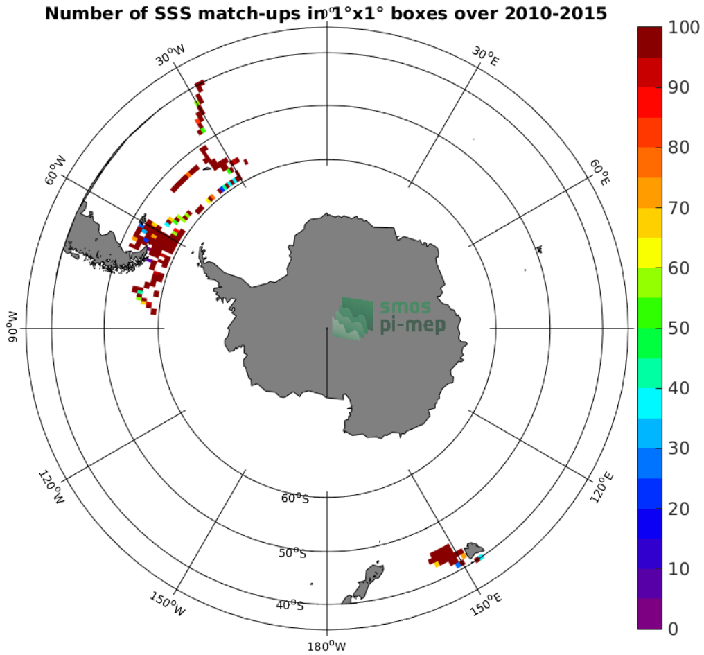
Figure 4: Number of SSS match-ups between TSG-SAMOS SSS and the CCI L4 Merged-OI v1.8 - 30-day running (ESA) SSS product for the Roaring Forties and Furious Fifties Pi-MEP region over 1°x1° boxes and for the full satellite product period.
