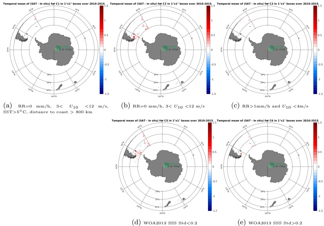
Figure 12: Temporal mean gridded over spatial boxes of size 1^\circ \times 1^\circ of \Delta SSS (CCI-L4-ESA-MERGED-OI-V1.8-30DAY-RUNNING - TSG-SAMOS) for 5 different subdatasets corresponding to:RR=0 mm/h, 3 < U_{10} < 12 m/s, SST >5^\circ\text{C} , distance to coast > 800 km (a), RR=0 mm/h, 3 < U_{10} < 12 m/s (b), RR >1 mm/h and U_{10} < 4 m/s (c), WOA2013 SSS Std <0.2 (d), WOA2013 SSS Std >0.2 (e).
