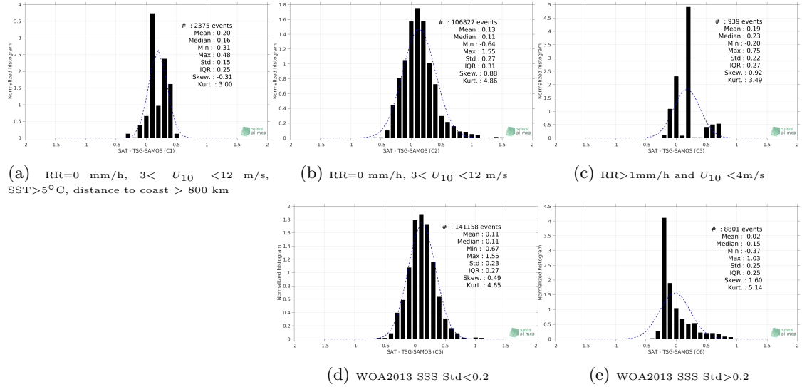
Figure 13: Normalized histogram of \Delta SSS (CCI-L4-ESA-MERGED-OI-V1.8-30DAY-RUNNING - TSG-SAMOS) for 5 different subdatasets corresponding to: RR=0 mm/h, 3 < U_{10} < 12 m/s, SST>5°C, distance to coast > 800 km (a), RR=0 mm/h, 3 < U_{10} < 12 m/s (b), RR>1mm/h and U_{10} < 4 m/s (c), WOA2013 SSS Std<0.2 (d), WOA2013 SSS Std>0.2 (e).
