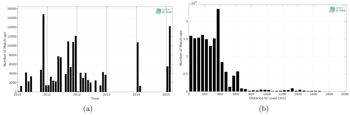
Figure 1: Number of match-ups between TSG-SAMOS and CCI-L4-ESA-MERGED-OI-V1.8-30DAY-RUNNING SSS as a function of time (a) and as function of the distance to coast (b) over the Roaring Forties and Furious Fifties Pi-MEP region and for the full satellite product period.
