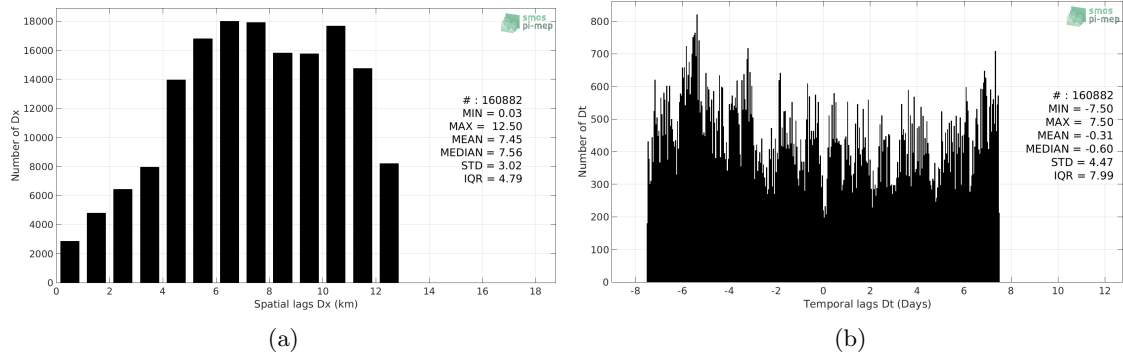
Figure 5: Histograms of the spatial (a) and temporal (b) lags between the time of the TSG-SAMOS measurements and the date of the corresponding CCI-L4-ESA-MERGED-OI-V1.8-30DAY-RUNNING SSS product.
