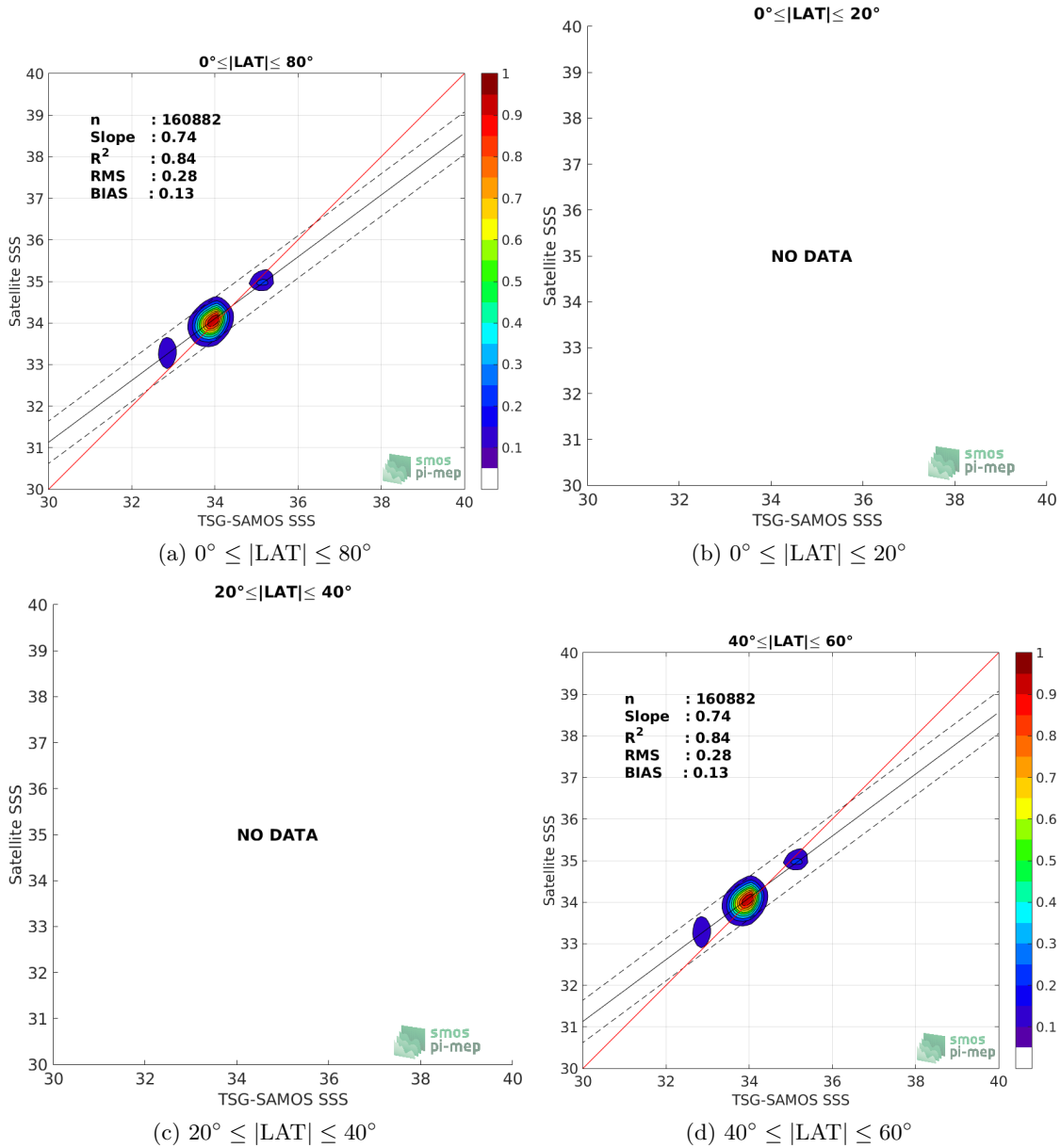
Figure 9: Contour maps of the concentration of CCI-L4-ESA-MERGED-OI-V1.8-30DAY-RUNNING SSS (y-axis) versus TSG-SAMOS SSS (x-axis) at match-up pairs for different latitude bands. For each plot, the red line shows x=y . The black thin and dashed lines indicate a linear fit through the data cloud and the \pm 95\% confidence levels, respectively. The number match-up pairs n , the slope and R^2 coefficient of the linear fit, the root mean square (RMS) and the mean bias between satellite and in situ data are indicated for each latitude band in each plots.
