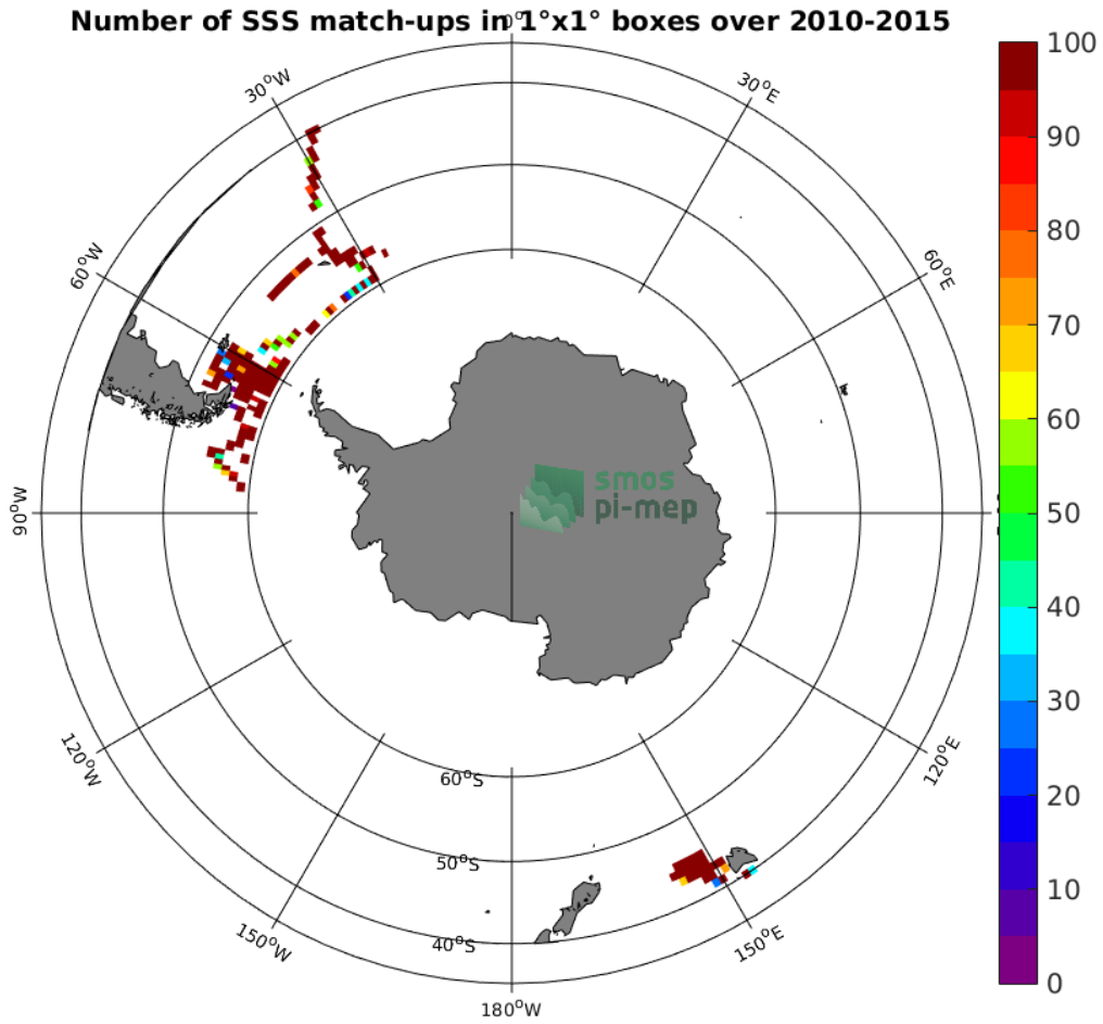
Figure 4: Number of SSS match-ups between TSG-SAMOS SSS and the CCI-L4-ESA-MERGED-OI-V1.8-30DAY-RUNNING SSS product for the Roaring Forties and Furious Fifties Pi-MEP region over 1°x1° boxes and for the full satellite product period.
