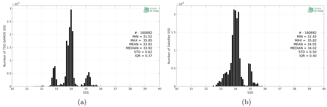
Figure 2: Histograms of SSS from TSG-SAMOS (a) and CCI-L4-ESA-MERGED-OI-V1.8-30DAY-RUNNING (b) considering all match-up pairs per bins of 0.1 over the Roaring Forties and Furious Fifties Pi-MEP region and for the full satellite product period.
