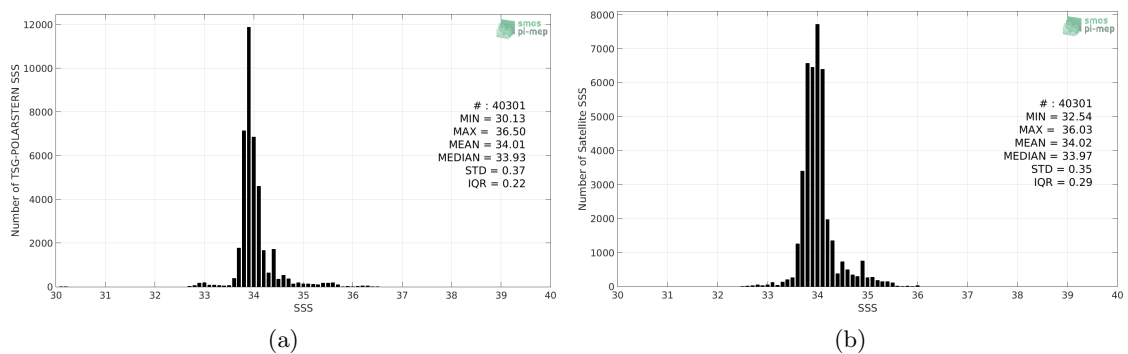
Figure 2: Histograms of SSS from TSG-POLARSTERN (a) and CCI L4 Merged-OI v1.8 - 30-day running (ESA) (b) considering all match-up pairs per bins of 0.1 over the Roaring Forties and Furious Fifties Pi-MEP region and for the full satellite product period.
