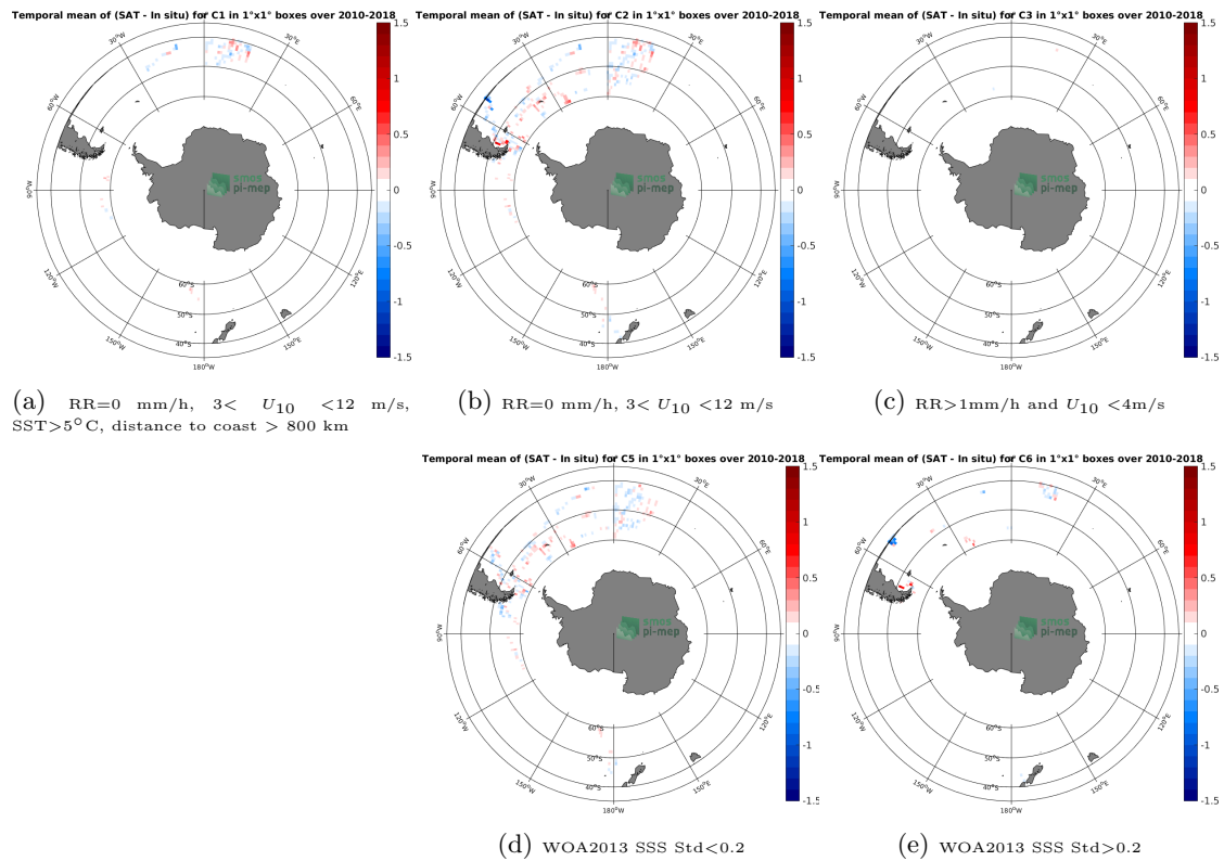
Figure 12: Temporal mean gridded over spatial boxes of size 1^{\circ}\times 1^{\circ} of \Delta\text{SSS} (CCI L4 Merged-OI v1.8 - 30-day running (ESA) - TSG-POLARSTERN) for 5 different subdatasets corresponding to:RR=0 mm/h, 3 < U_{10} < 12 m/s, SST >5^{\circ}\text{C} , distance to coast > 800 km (a), RR=0 mm/h, 3 < U_{10} < 12 m/s (b), RR >1 mm/h and U_{10} < 4 m/s (c), WOA2013 SSS Std <0.2 (d), WOA2013 SSS Std >0.2 (e).
