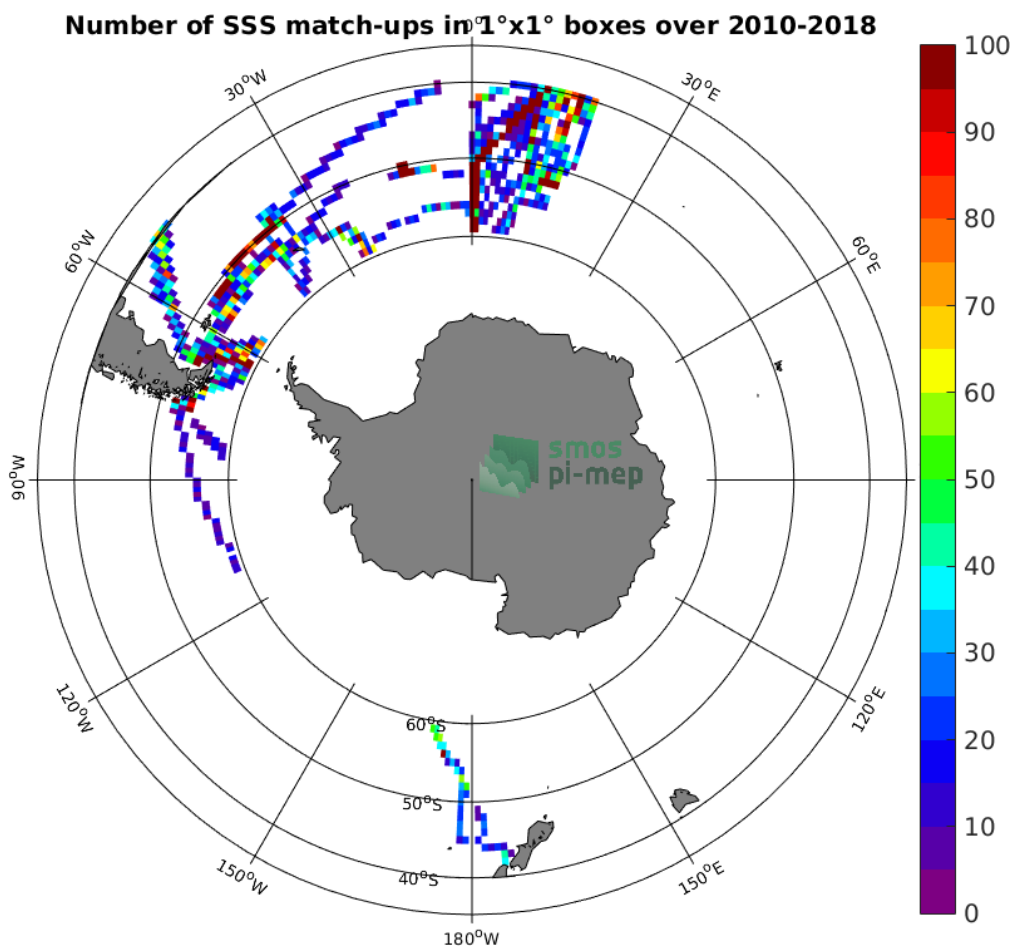
Figure 4: Number of SSS match-ups between TSG-POLARSTERN SSS and the CCI L4 Merged-OI v1.8 - 30-day running (ESA) SSS product for the Roaring Forties and Furious Fifties Pi-MEP region over 1^\circ \times 1^\circ boxes and for the full satellite product period.
