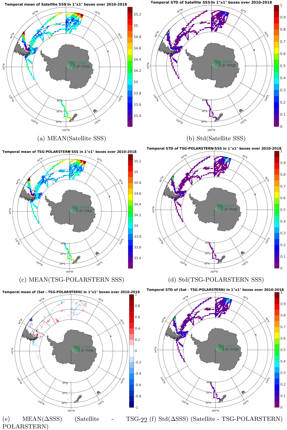
Figure 6: Temporal mean (left) and Std (right) of SSS from CCI L4 Merged-OI v1.8 - 30-day running (ESA) (top), TSG-POLARSTERN (middle), and of \Delta SSS (Satellite - TSG-POLARSTERN). Only match-up pairs are used to generate these maps.
