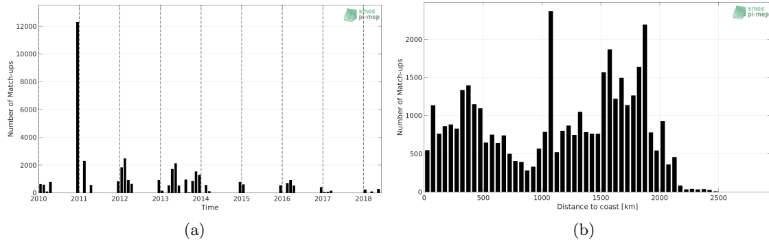
Figure 1: Number of match-ups between TSG-POLARSTERN and CCI L4 Merged-OI v1.8 - 30-day running (ESA) SSS as a function of time (a) and as function of the distance to coast (b) over the Roaring Forties and Furious Fifties Pi-MEP region and for the full satellite product period.
