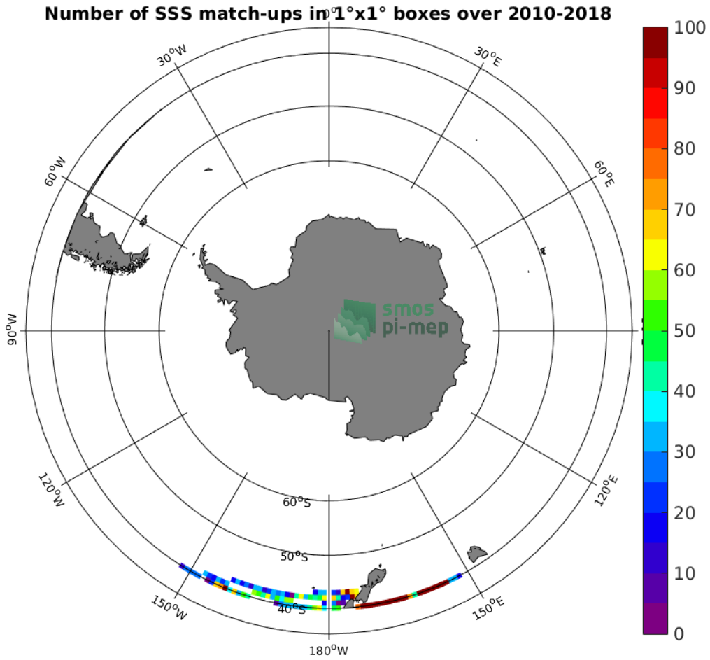
Figure 4: Number of SSS match-ups between TSG-LEGOS-DM SSS and the CCI L4 Merged-OI v1.8 - 30-day running (ESA) SSS product for the Roaring Forties and Furious Fifties Pi-MEP region over 1°x1° boxes and for the full satellite product period.
