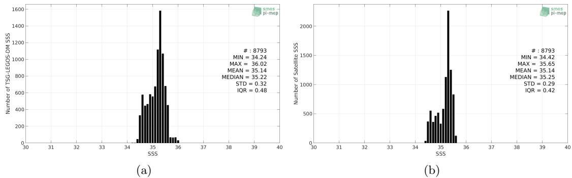
Figure 2: Histograms of SSS from TSG-LEGOS-DM (a) and CCI L4 Merged-OI v1.8 - 30-day running (ESA) (b) considering all match-up pairs per bins of 0.1 over the Roaring Forties and Furious Fifties Pi-MEP region and for the full satellite product period.
