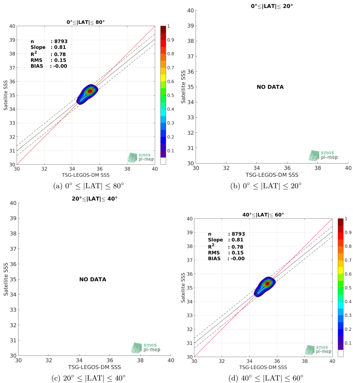
Figure 9: Contour maps of the concentration of CCI L4 Merged-OI v1.8 - 30-day running (ESA) SSS (y-axis) versus TSG-LEGOS-DM SSS (x-axis) at match-up pairs for different latitude bands. For each plot, the red line shows x=y . The black thin and dashed lines indicate a linear fit through the data cloud and the \pm 95\% confidence levels, respectively. The number match-up pairs n , the slope and R^2 coefficient of the linear fit, the root mean square (RMS) and the mean bias between satellite and in situ data are indicated for each latitude band in each plots.
