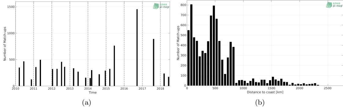
Figure 1: Number of match-ups between TSG-LEGOS-DM and CCI L4 Merged-OI v1.8 - 30-day running (ESA) SSS as a function of time (a) and as function of the distance to coast (b) over the Roaring Forties and Furious Fifties Pi-MEP region and for the full satellite product period.
