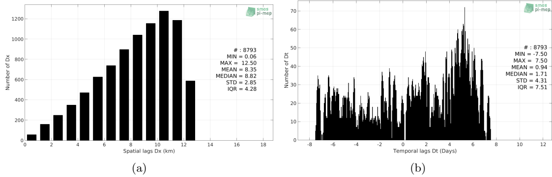
Figure 5: Histograms of the spatial (a) and temporal (b) lags between the time of the TSG-LEGOS-DM measurements and the date of the corresponding CCI L4 Merged-OI v1.8 - 30-day running (ESA) SSS product.
