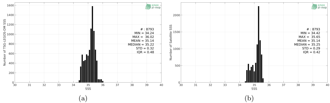
Figure 2: Histograms of SSS from TSG-LEGOS-DM (a) and CCI-L4-ESA-MERGED-OI-V1.8-30DAY-RUNNING (b) considering all match-up pairs per bins of 0.1 over the Roaring Forties and Furious Fifties Pi-MEP region and for the full satellite product period.
