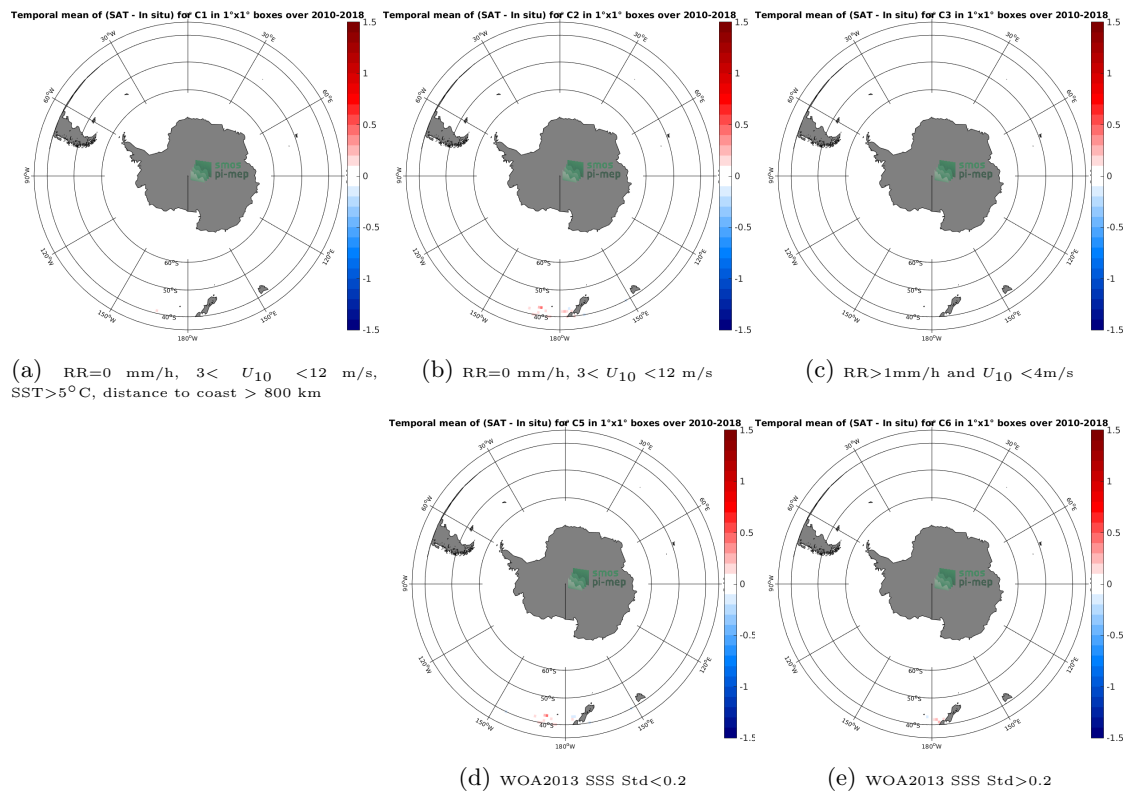
Figure 12: Temporal mean gridded over spatial boxes of size 1^\circ \times 1^\circ of \Delta SSS (CCI-L4-ESA-MERGED-OI-V1.8-30DAY-RUNNING - TSG-LEGOS-DM) for 5 different subdatasets corresponding to: RR=0 mm/h, 3 < U_{10} < 12 m/s, SST > 5^\circ\text{C} , distance to coast > 800 km (a), RR=0 mm/h, 3 < U_{10} < 12 m/s (b), RR > 1 mm/h and U_{10} < 4 m/s (c), WOA2013 SSS Std < 0.2 (d), WOA2013 SSS Std > 0.2 (e).
