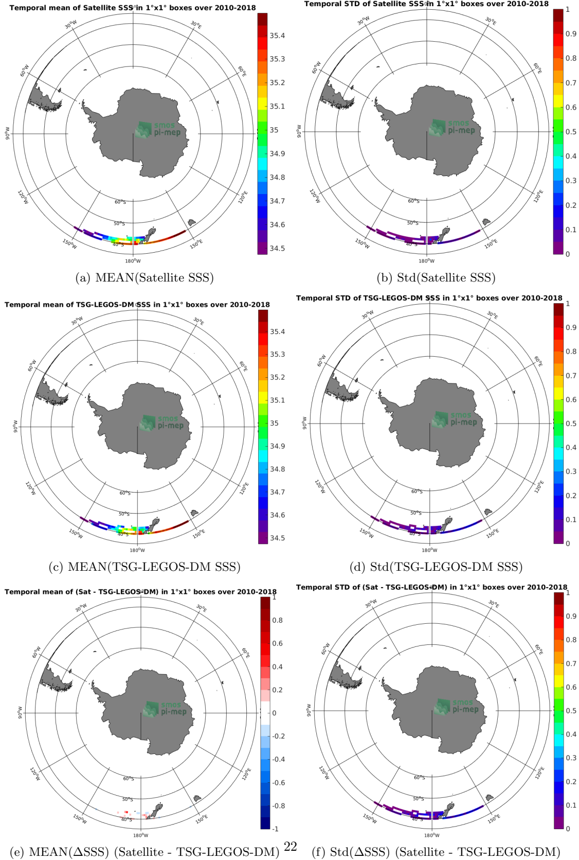
Figure 6: Temporal mean (left) and Std (right) of SSS from CCI-L4-ESA-MERGED-OI-V1.8-30DAY-RUNNING (top), TSG-LEGOS-DM (middle), and of \Delta SSS (Satellite - TSG-LEGOS-DM). Only match-up pairs are used to generate these maps.
