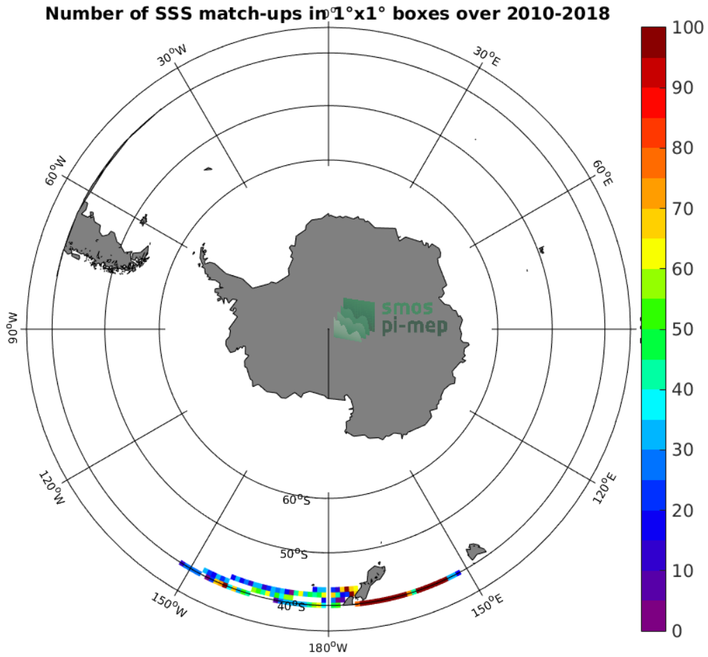
Figure 4: Number of SSS match-ups between TSG-LEGOS-DM SSS and the CCI-L4-ESA-MERGED-OI-V1.8-30DAY-RUNNING SSS product for the Roaring Forties and Furious Fifties Pi-MEP region over 1°x1° boxes and for the full satellite product period.
