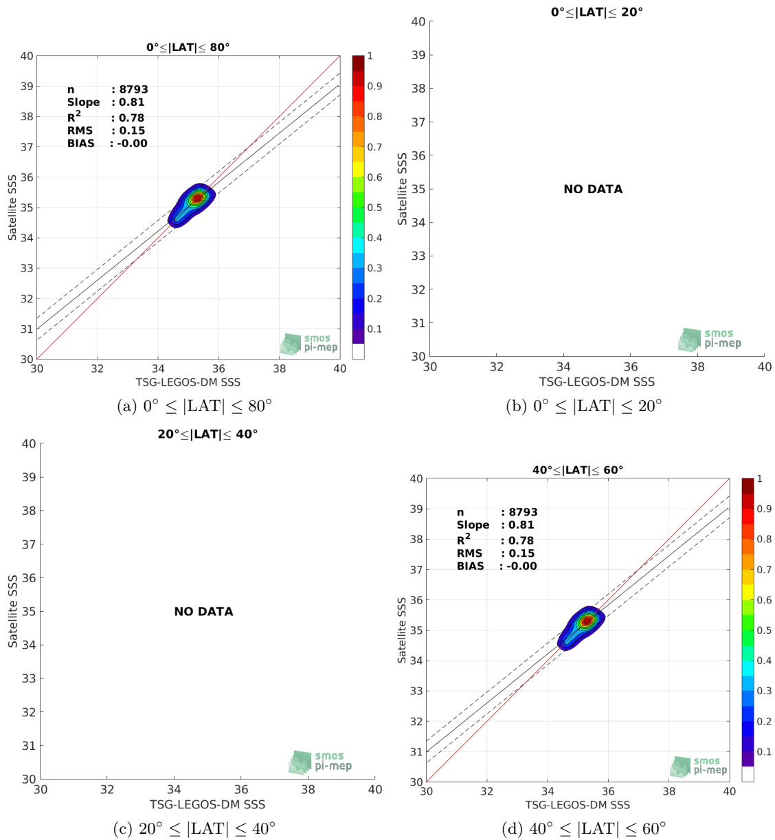
Figure 9: Contour maps of the concentration of CCI-L4-ESA-MERGED-OI-V1.8-30DAY-RUNNING SSS (y-axis) versus TSG-LEGOS-DM SSS (x-axis) at match-up pairs for different latitude bands. For each plot, the red line shows x=y . The black thin and dashed lines indicate a linear fit through the data cloud and the \pm 95\% confidence levels, respectively. The number match-up pairs n , the slope and R^2 coefficient of the linear fit, the root mean square (RMS) and the mean bias between satellite and in situ data are indicated for each latitude band in each plots.
