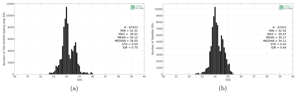
Figure 2: Histograms of SSS from TSG-GOSUD-Sailing-ship (a) and CCI-L4-ESA-MERGED-OI-V1.8-30DAY-RUNNING (b) considering all match-up pairs per bins of 0.1 over the Roaring Forties and Furious Fifties Pi-MEP region and for the full satellite product period.
