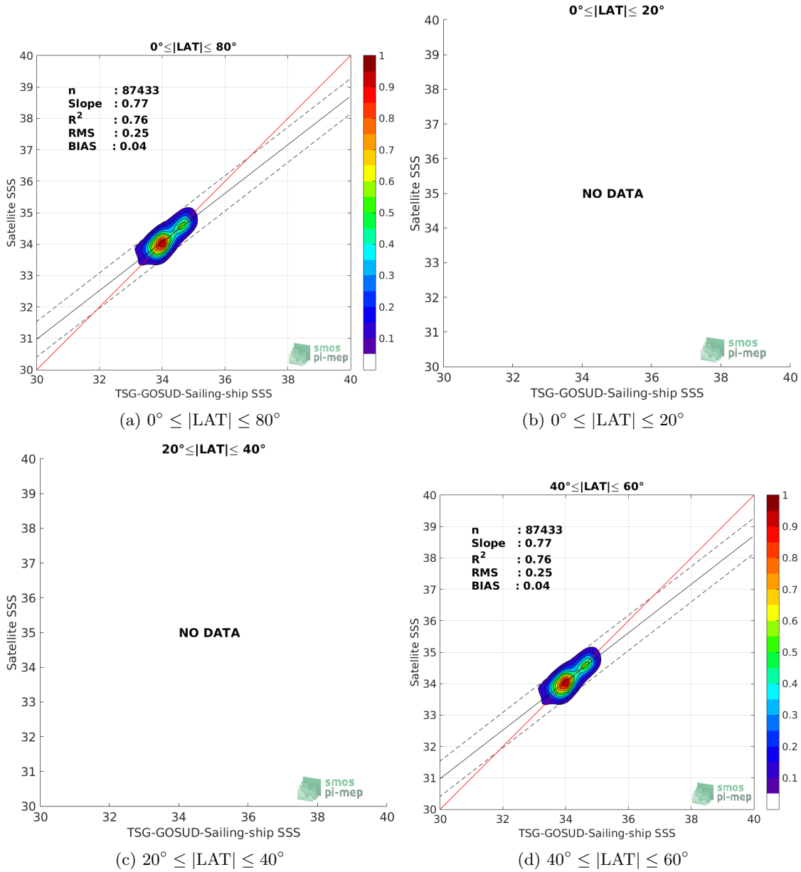
Figure 9: Contour maps of the concentration of CCI-L4-ESA-MERGED-OI-V1.8-30DAY-RUNNING SSS (y-axis) versus TSG-GOSUD-Sailing-ship SSS (x-axis) at match-up pairs for different latitude bands. For each plot, the red line shows x=y . The black thin and dashed lines indicate a linear fit through the data cloud and the \pm 95\% confidence levels, respectively. The number match-up pairs n , the slope and R^2 coefficient of the linear fit, the root mean square (RMS) and the mean bias between satellite and in situ data are indicated for each latitude band in each plots.
