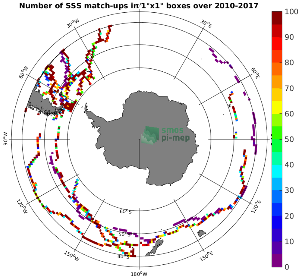
Figure 4: Number of SSS match-ups between TSG-GOSUD-Sailing-ship SSS and the CCI-L4-ESA-MERGED-OI-V1.8-30DAY-RUNNING SSS product for the Roaring Forties and Furious Fifties Pi-MEP region over 1°x1° boxes and for the full satellite product period.
