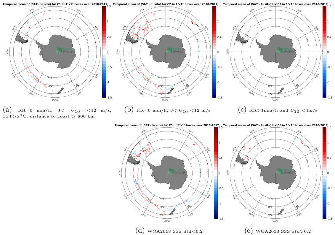
Figure 12: Temporal mean gridded over spatial boxes of size 1^\circ \times 1^\circ of \Delta SSS (CCI-L4-ESA-MERGED-OI-V1.8-30DAY-RUNNING - TSG-GOSUD-Sailing-ship) for 5 different subdatasets corresponding to: RR=0 mm/h, 3 < U_{10} < 12 m/s, SST > 5°C, distance to coast > 800 km (a), RR=0 mm/h, 3 < U_{10} < 12 m/s (b), RR > 1 mm/h and U_{10} < 4 m/s (c), WOA2013 SSS Std < 0.2 (d), WOA2013 SSS Std > 0.2 (e).
