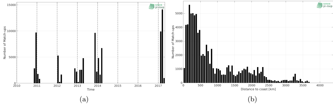
Figure 1: Number of match-ups between TSG-GOSUD-Sailing-ship and CCI-L4-ESA-MERGED-OI-V1.8-30DAY-RUNNING SSS as a function of time (a) and as function of the distance to coast (b) over the Roaring Forties and Furious Fifties Pi-MEP region and for the full satellite product period.
