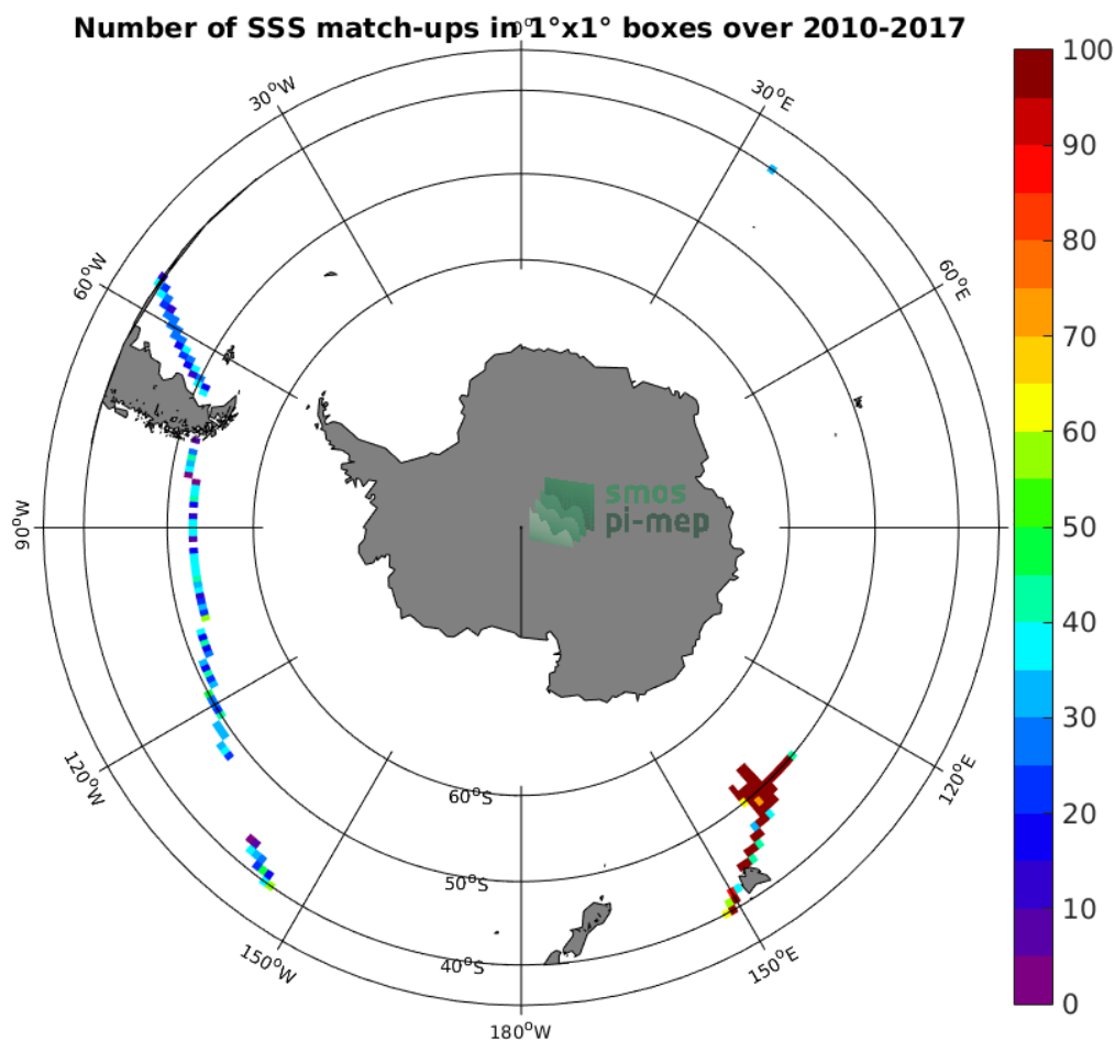
Figure 4: Number of SSS match-ups between TSG-GOSUD-Research-vessel SSS and the CCI L4 Merged-OI v1.8 - 30-day running (ESA) SSS product for the Roaring Forties and Furious Fifties Pi-MEP region over 1°x1° boxes and for the full satellite product period.
