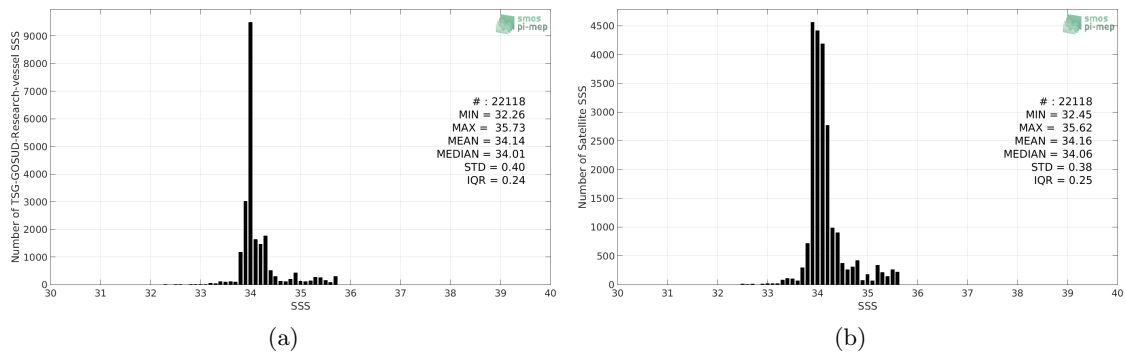
Figure 2: Histograms of SSS from TSG-GOSUD-Research-vessel (a) and CCI L4 Merged-OI v1.8 - 30-day running (ESA) (b) considering all match-up pairs per bins of 0.1 over the Roaring Forties and Furious Fifties Pi-MEP region and for the full satellite product period.
