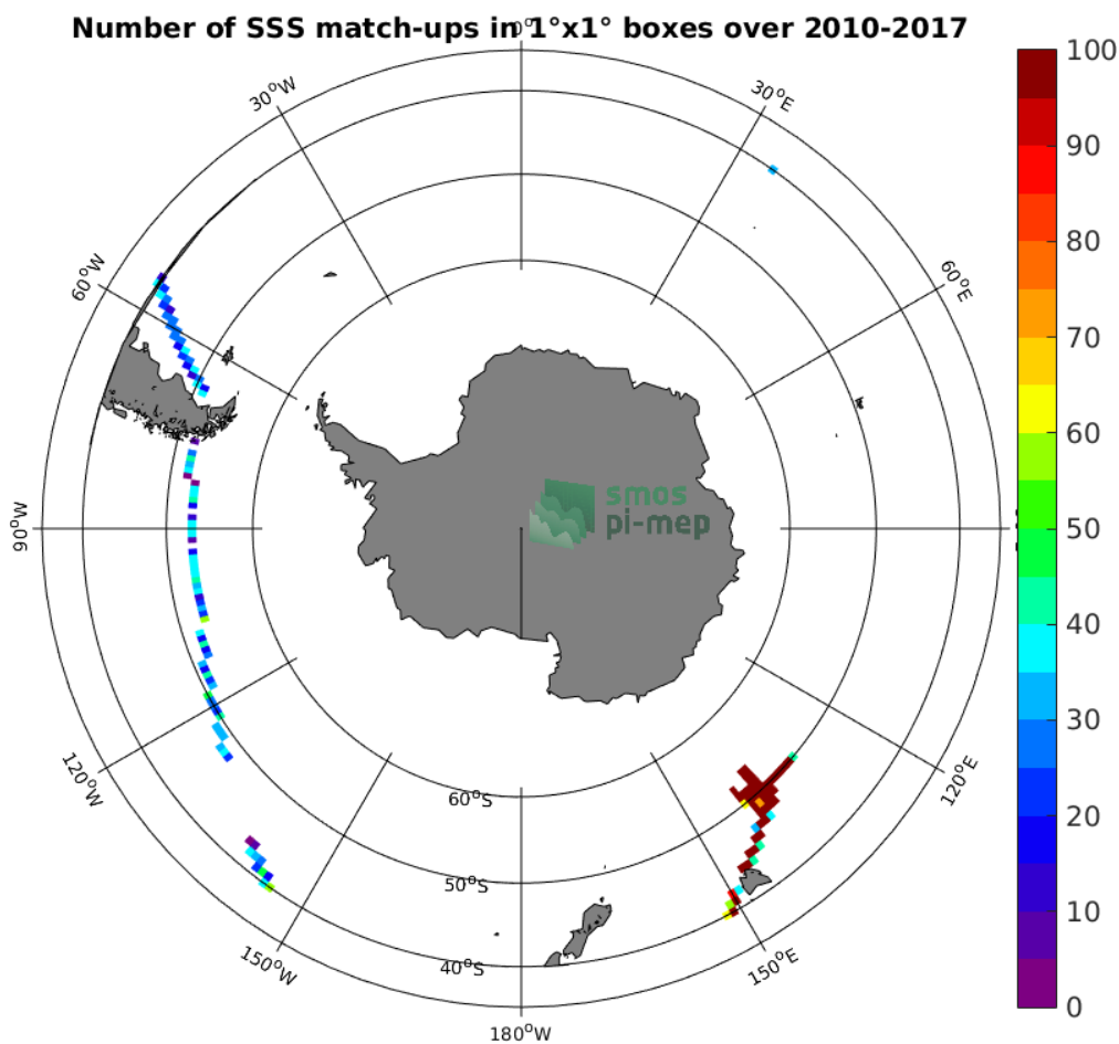
Figure 4: Number of SSS match-ups between TSG-GOSUD-Research-vessel SSS and the CCI-L4-ESA-MERGED-OI-V1.8-30DAY-RUNNING SSS product for the Roaring Forties and Furious Fifties Pi-MEP region over 1°x1° boxes and for the full satellite product period.
