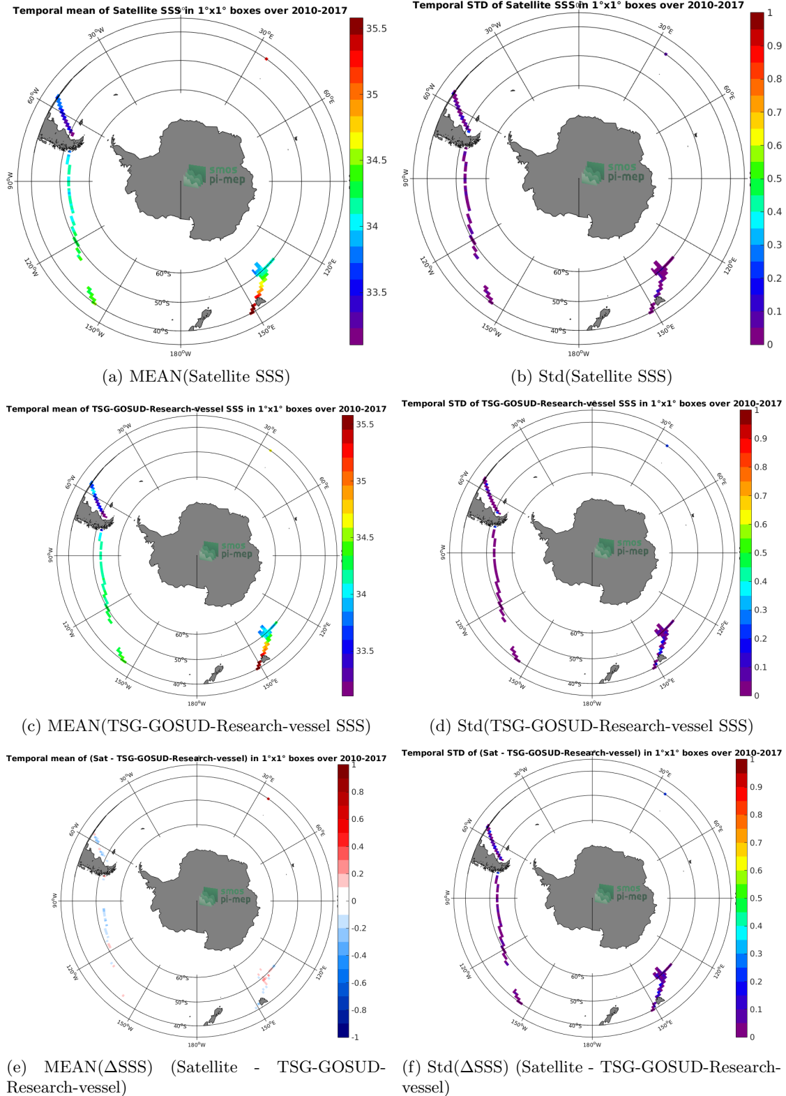
Figure 6: Temporal mean (left) and Std (right) of SSS from CCI-L4-ESA-MERGED-OI-V1.8-30DAY-RUNNING (top), TSG-GOSUD-Research-vessel (middle), and of \Delta SSS (Satellite - TSG-GOSUD-Research-vessel). Only match-up pairs are used to generate these maps.
