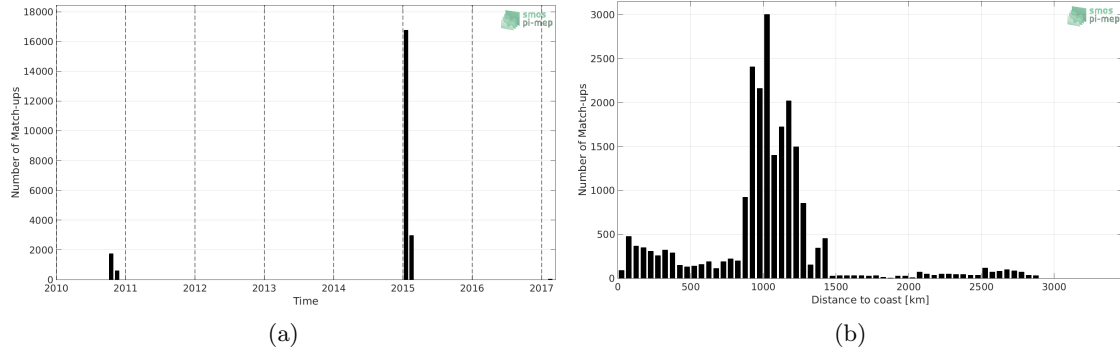
Figure 1: Number of match-ups between TSG-GOSUD-Research-vessel and CCI-L4-ESA-MERGED-OI-V1.8-30DAY-RUNNING SSS as a function of time (a) and as function of the distance to coast (b) over the Roaring Forties and Furious Fifties Pi-MEP region and for the full satellite product period.
