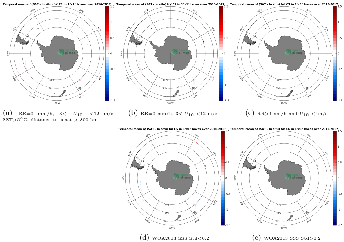
Figure 12: Temporal mean gridded over spatial boxes of size 1^\circ \times 1^\circ of \Delta SSS (CCI-L4-ESA-MERGED-OI-V1.8-30DAY-RUNNING - TSG-GOSUD-Research-vessel) for 5 different sub-datasets corresponding to:RR=0 mm/h, 3 < U_{10} < 12 m/s, SST>5°C, distance to coast > 800 km (a), RR=0 mm/h, 3 < U_{10} < 12 m/s (b), RR>1mm/h and U_{10} < 4 m/s (c), WOA2013 SSS Std<0.2 (d), WOA2013 SSS Std>0.2 (e).
