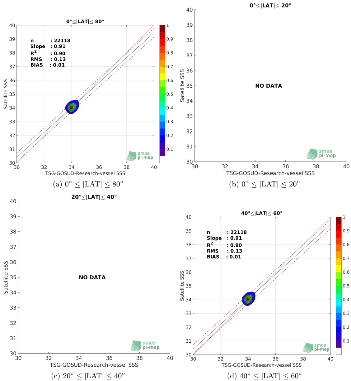
Figure 9: Contour maps of the concentration of CCI-L4-ESA-MERGED-OI-V1.8-30DAY-RUNNING SSS (y-axis) versus TSG-GOSUD-Research-vessel SSS (x-axis) at match-up pairs for different latitude bands. For each plot, the red line shows x=y . The black thin and dashed lines indicate a linear fit through the data cloud and the \pm 95\% confidence levels, respectively. The number match-up pairs n , the slope and R^2 coefficient of the linear fit, the root mean square (RMS) and the mean bias between satellite and in situ data are indicated for each latitude band in each plots.
