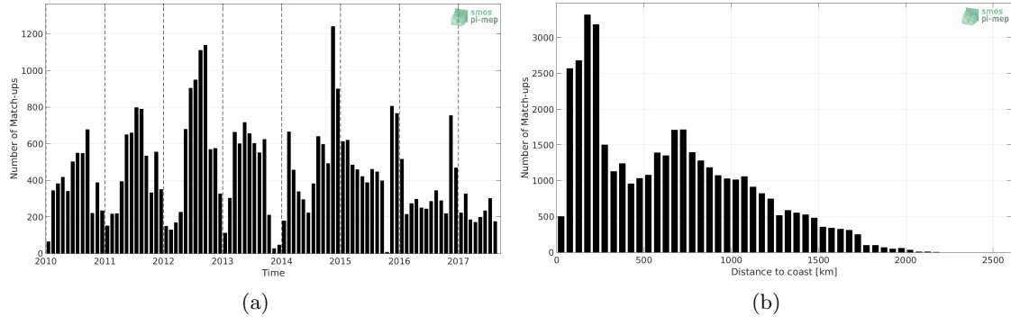
Figure 1: Number of match-ups between Sea mammals and CCI L4 Merged-OI v1.8 - 30-day running (ESA) SSS as a function of time (a) and as function of the distance to coast (b) over the Roaring Forties and Furious Fifties Pi-MEP region and for the full satellite product period.
