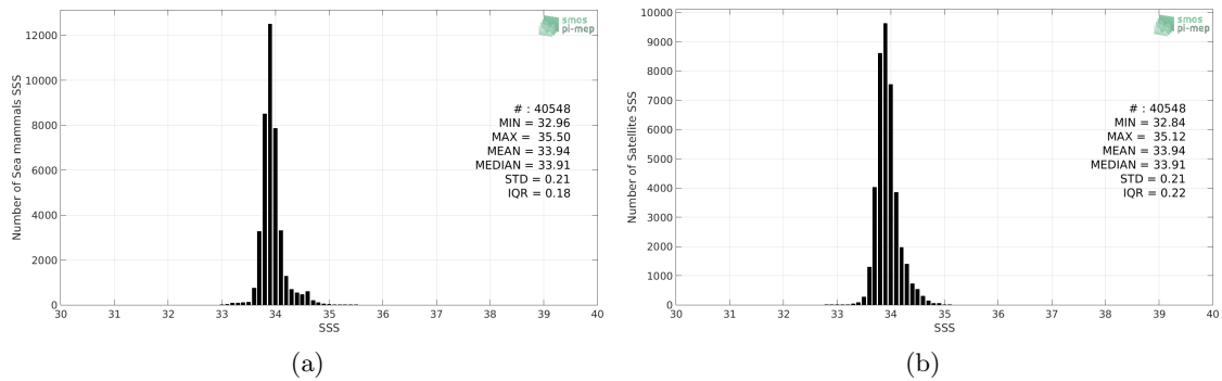
Figure 2: Histograms of SSS from Sea mammals (a) and CCI-L4-ESA-MERGED-OI-V1.8-30DAY-RUNNING (b) considering all match-up pairs per bins of 0.1 over the Roaring Forties and Furious Fifties Pi-MEP region and for the full satellite product period.
