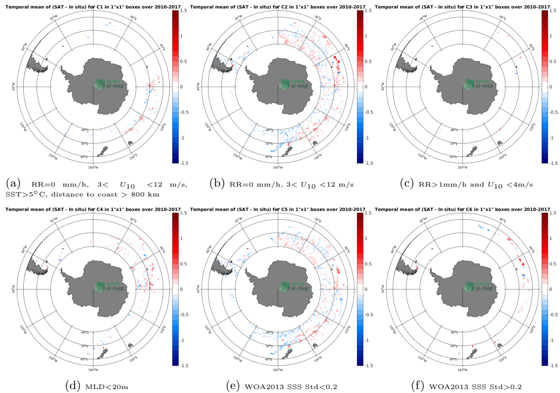
Figure 12: Temporal mean gridded over spatial boxes of size 1^\circ \times 1^\circ of \Delta SSS (CCI-L4-ESAMERGED-OI-V1.8-30DAY-RUNNING - Sea mammals) for 6 different subdatasets corresponding to:RR=0 mm/h, 3 < U_{10} < 12 m/s, SST >5^\circ C, distance to coast > 800 km (a), RR=0 mm/h, 3 < U_{10} < 12 m/s (b), RR >1 mm/h and U_{10} < 4 m/s (c),MLD <20 m (d),WOA2013 SSS Std <0.2 (e),WOA2013 SSS Std >0.2 (f).
