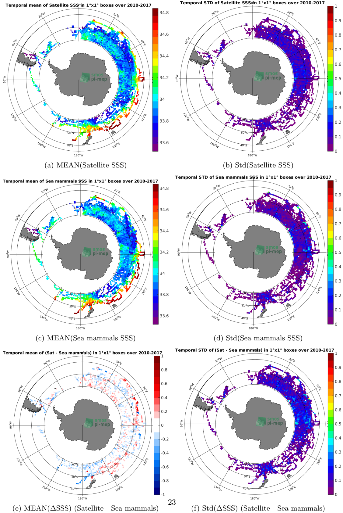
Figure 6: Temporal mean (left) and Std (right) of SSS from CCI-L4-ESA-MERGED-OI-V1.8-30DAY-RUNNING (top), Sea mammals (middle), and of \Delta SSS (Satellite - Sea mammals). Only match-up pairs are used to generate these maps.
