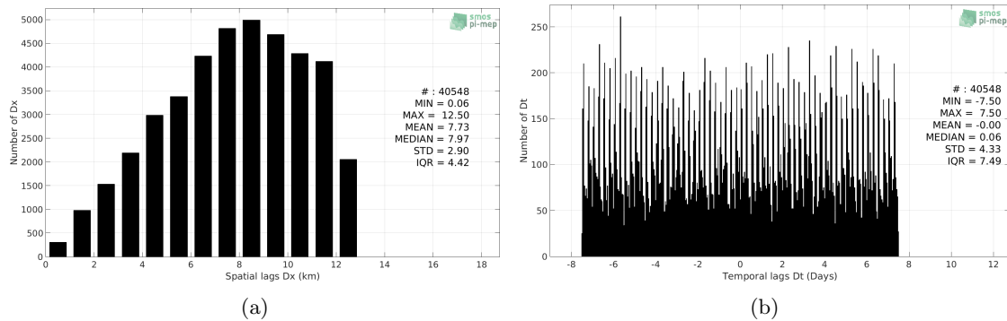
Figure 5: Histograms of the spatial (a) and temporal (b) lags between the time of the Sea mammals measurements and the date of the corresponding CCI-L4-ESA-MERGED-OI-V1.8-30DAY-RUNNING SSS product.
