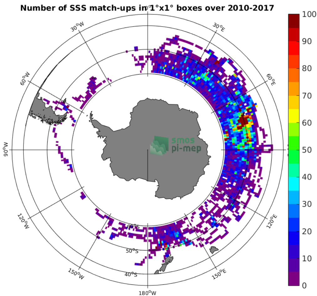
Figure 4: Number of SSS match-ups between Sea mammals SSS and the CCI-L4-ESA-MERGED-OI-V1.8-30DAY-RUNNING SSS product for the Roaring Forties and Furious Fifties Pi-MEP region over 1°x1° boxes and for the full satellite product period.
