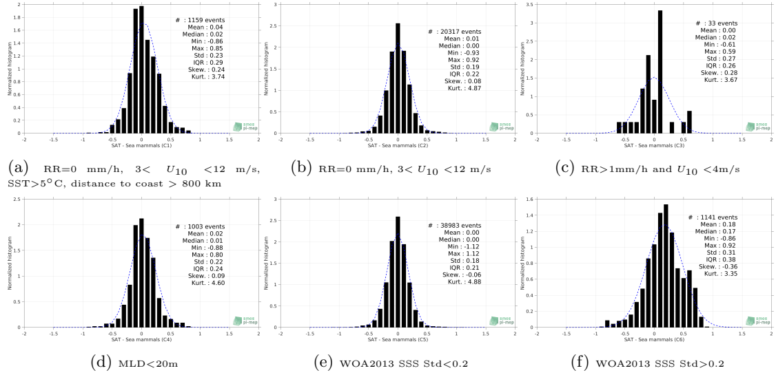
Figure 13: Normalized histogram of \Delta SSS (CCI-L4-ESA-MERGED-OI-V1.8-30DAY-RUNNING - Sea mammals) for 6 different subdatasets corresponding to: RR=0 mm/h, 3 < U_{10} < 12 m/s, SST>5°C, distance to coast > 800 km (a), RR=0 mm/h, 3 < U_{10} < 12 m/s (b), RR>1mm/h and U_{10} < 4 m/s (c), MLD<20m (d), WOA2013 SSS Std<0.2 (e), WOA2013 SSS Std>0.2 (f).
