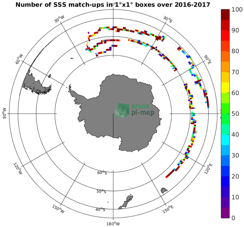
Figure 3: Number of SSS match-ups between Surface drifters SSS and the CCI-L4-ESA-MERGED-OI-V1.8-30DAY-RUNNING SSS product for the Roaring Forties and Furious Fifties Pi-MEP region over 1°x1° boxes and for the full satellite product period.
