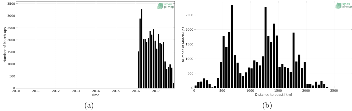
Figure 1: Number of match-ups between Surface drifters and CCI-L4-ESA-MERGED-OI-V1.8-30DAY-RUNNING SSS as a function of time (a) and as function of the distance to coast (b) over the Roaring Forties and Furious Fifties Pi-MEP region and for the full satellite product period.
