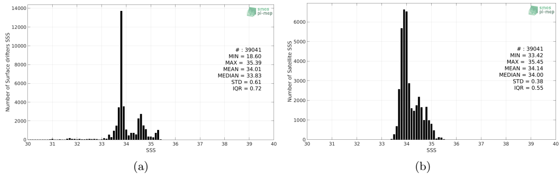
Figure 2: Histograms of SSS from Surface drifters (a) and CCI-L4-ESA-MERGED-OI-V1.8-30DAY-RUNNING (b) considering all match-up pairs per bins of 0.1 over the Roaring Forties and Furious Fifties Pi-MEP region and for the full satellite product period.
