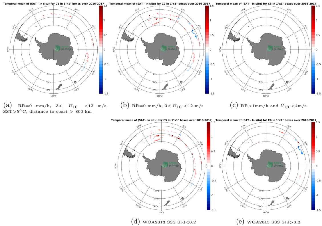
Figure 11: Temporal mean gridded over spatial boxes of size 1^\circ \times 1^\circ of \Delta SSS (CCI-L4-ESAMERGED-OI-V1.8-30DAY-RUNNING - Surface drifters) for 5 different subdatasets corresponding to:RR=0 mm/h, 3 < U_{10} < 12 m/s, SST >5^\circ\text{C} , distance to coast > 800 km (a), RR=0 mm/h, 3 < U_{10} < 12 m/s (b), RR >1 mm/h and U_{10} < 4 m/s (c), WOA2013 SSS Std <0.2 (d), WOA2013 SSS Std >0.2 (e).
