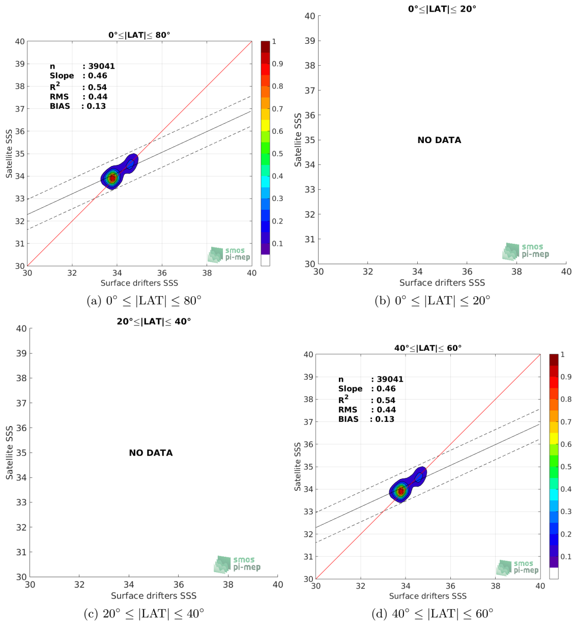
Figure 8: Contour maps of the concentration of CCI-L4-ESA-MERGED-OI-V1.8-30DAY-RUNNING SSS (y-axis) versus Surface drifters SSS (x-axis) at match-up pairs for different latitude bands. For each plot, the red line shows x=y . The black thin and dashed lines indicate a linear fit through the data cloud and the \pm 95\% confidence levels, respectively. The number match-up pairs n , the slope and R^2 coefficient of the linear fit, the root mean square (RMS) and the mean bias between satellite and in situ data are indicated for each latitude band in each plots.
