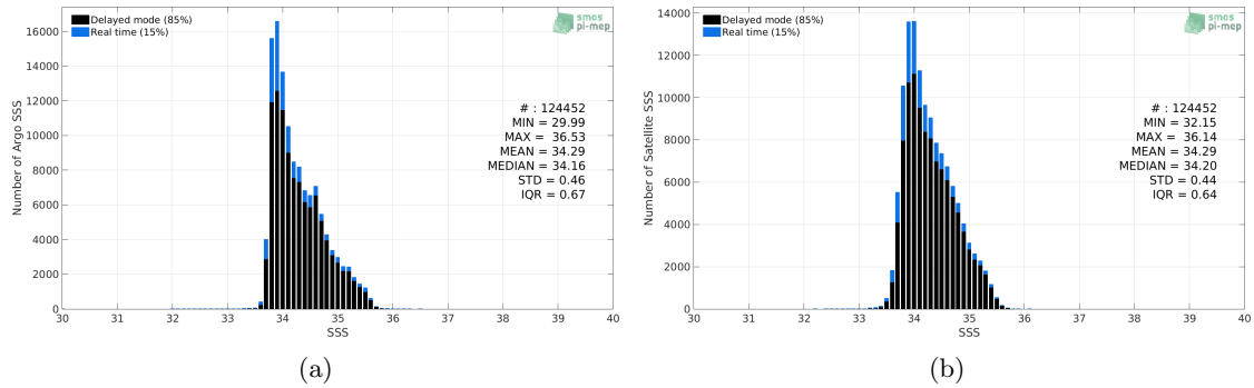
Figure 2: Histograms of SSS from Argo (a) and CCI L4 Merged-OI v1.8 - 30-day running (ESA) (b) considering all match-up pairs per bins of 0.1 over the Roaring Forties and Furious Fifties Pi-MEP region and for the full satellite product period.
