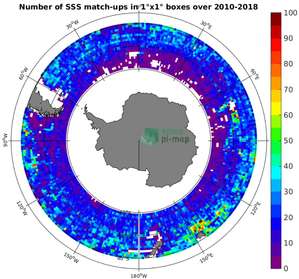
Figure 4: Number of SSS match-ups between Argo SSS and the CCI L4 Merged-OI v1.8 - 30-day running (ESA) SSS product for the Roaring Forties and Furious Fifties Pi-MEP region over 1^\circ \times 1^\circ boxes and for the full satellite product period.
