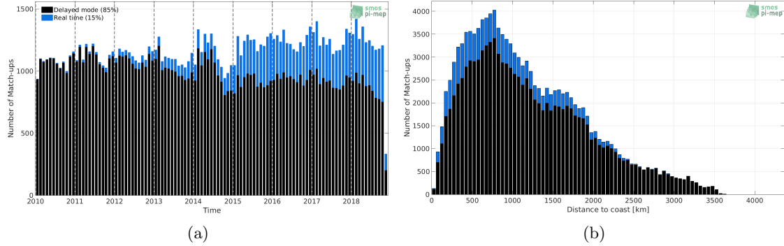
Figure 1: Number of match-ups between Argo and CCI L4 Merged-OI v1.8 - 30-day running (ESA) SSS as a function of time (a) and as function of the distance to coast (b) over the Roaring Forties and Furious Fifties Pi-MEP region and for the full satellite product period.
