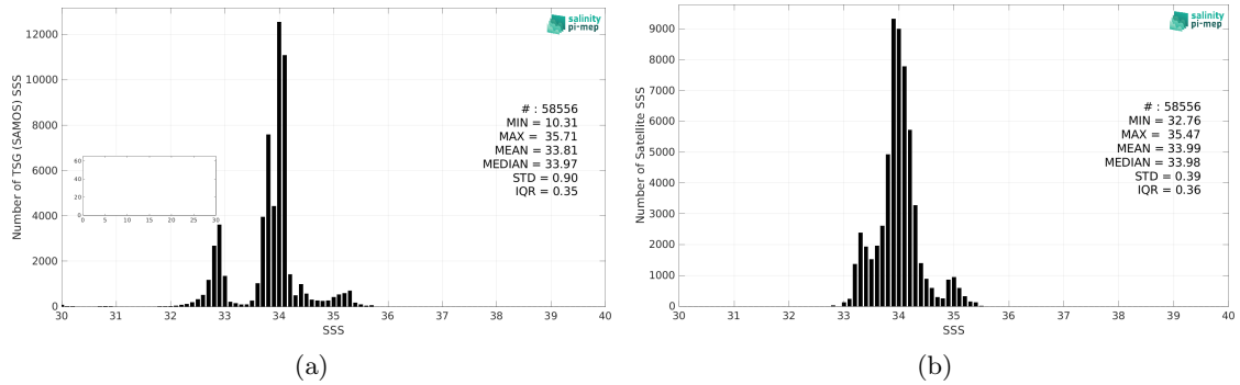
Figure 2: Histograms of SSS from TSG (SAMOS) (a) and Aquarius SSS L4 OI v5 - Weekly (IPRC) (b) considering all match-up pairs per bins of 0.1 over the Roaring Forties and Furious Fifties Pi-MEP region and for the full satellite product period.
