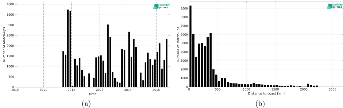
Figure 1: Number of match-ups between TSG (SAMOS) and Aquarius SSS L4 OI v5 - Weekly (IPRC) SSS as a function of time (a) and as function of the distance to coast (b) over the Roaring Forties and Furious Fifties Pi-MEP region and for the full satellite product period.
