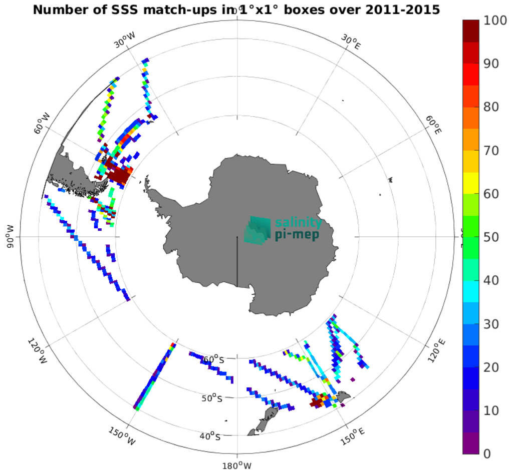
Figure 4: Number of SSS match-ups between TSG (SAMOS) SSS and the Aquarius SSS L4 OI v5 - Weekly (IPRC) SSS product for the Roaring Forties and Furious Fifties Pi-MEP region over 1^\circ \times 1^\circ boxes and for the full satellite product period.
