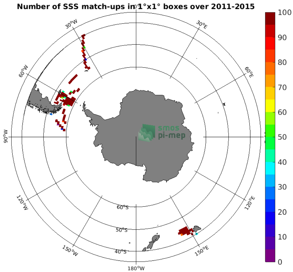
Figure 4: Number of SSS match-ups between TSG (SAMOS) SSS and the Aquarius SSS L4 OI v5 - Weekly (IPRC) SSS product for the Roaring Forties and Furious Fifties Pi-MEP region over 1°x1° boxes and for the full satellite product period.
