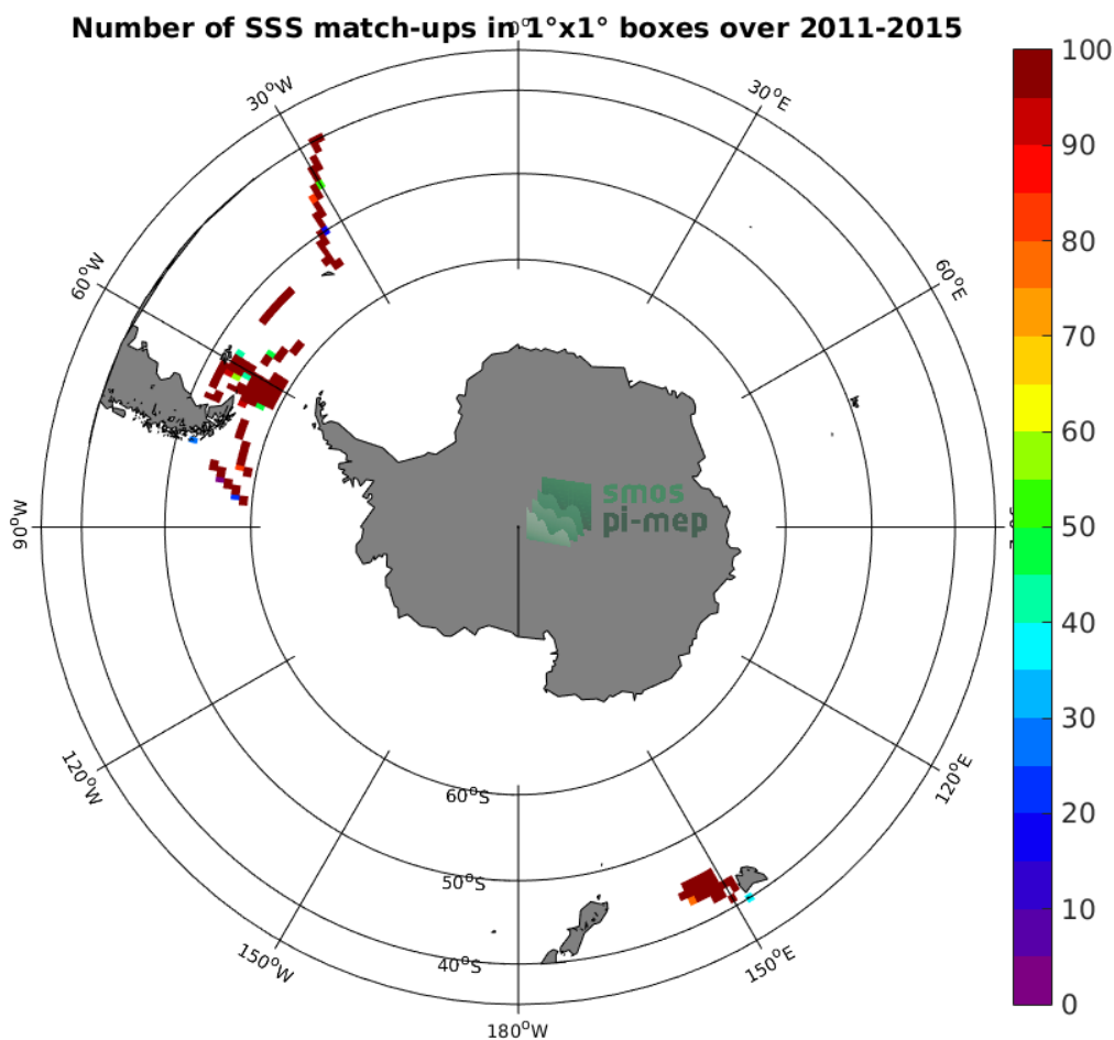
Figure 4: Number of SSS match-ups between TSG-SAMOS SSS and the Aquarius-L4-IPRC-V5-WEEKLY SSS product for the Roaring Forties and Furious Fifties Pi-MEP region over 1°x1° boxes and for the full satellite product period.
