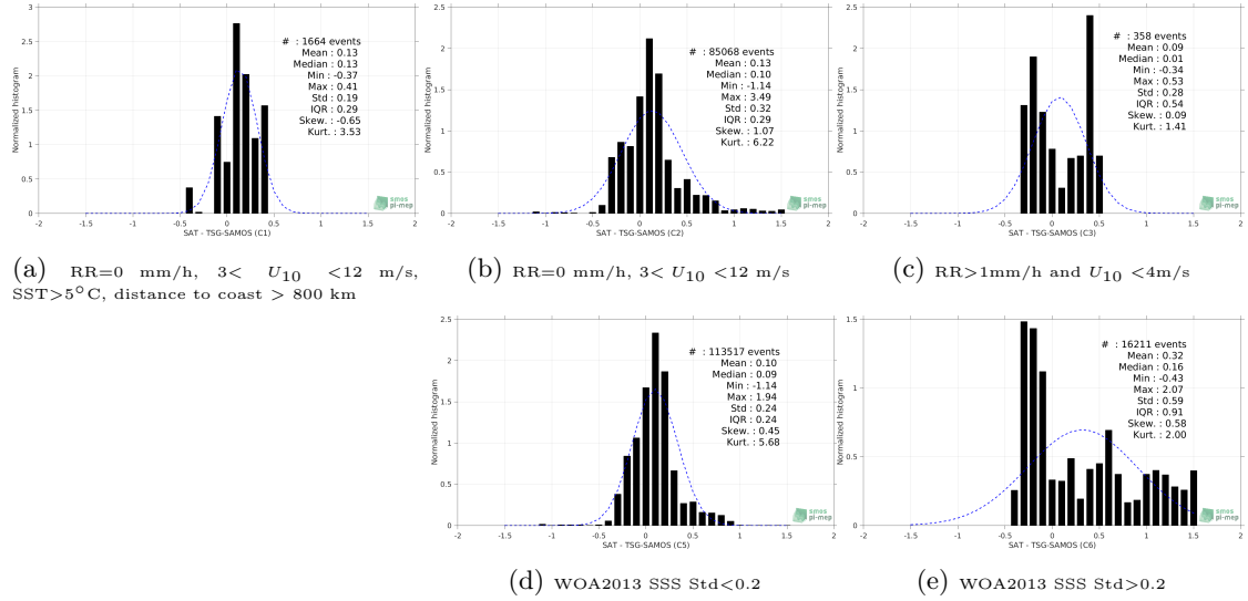
Figure 13: Normalized histogram of \Delta\text{SSS} (Aquarius-L4-IPRC-V5-WEEKLY - TSG-SAMOS) for 5 different subdatasets corresponding to: RR=0 mm/h, 3 < U_{10} < 12 m/s, SST>5°C, distance to coast > 800 km (a), RR=0 mm/h, 3 < U_{10} < 12 m/s (b), RR>1mm/h and U_{10} < 4 m/s (c), WOA2013 SSS Std<0.2 (d), WOA2013 SSS Std>0.2 (e).
