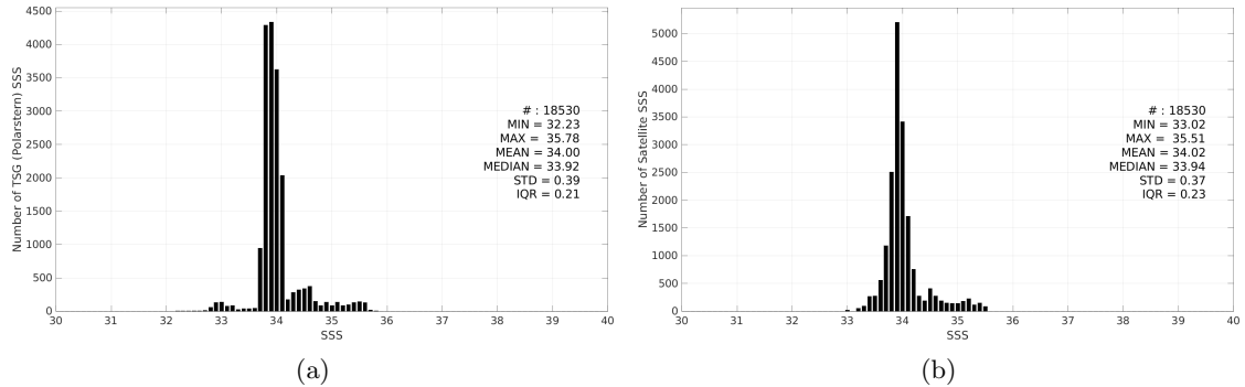
Figure 3: Histograms of SSS from TSG (Polarstern) (a) and Aquarius SSS L4 OI v5 - Weekly (IPRC) (b) considering all match-up pairs per bins of 0.1 over the Roaring Forties and Furious Fifties Pi-MEP region and for the full satellite product period.
