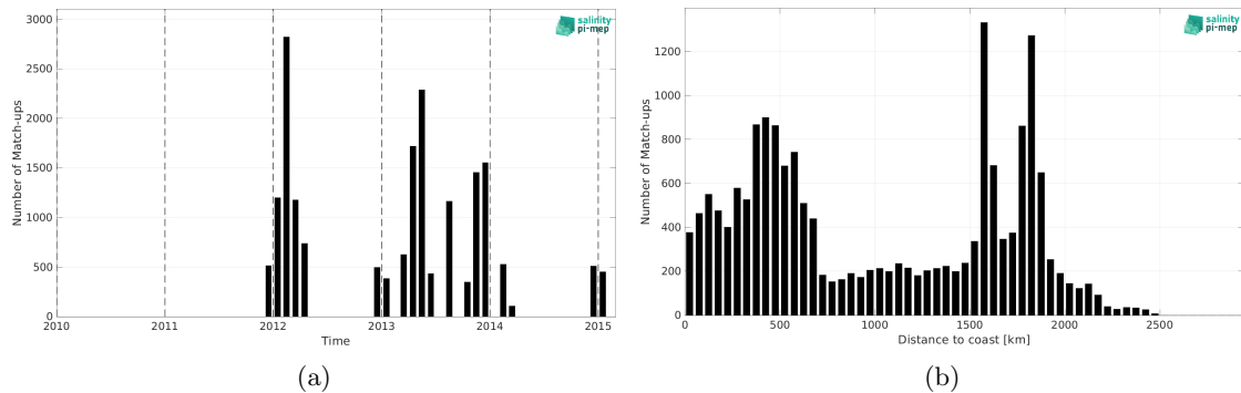
Figure 2: Number of match-ups between TSG (Polarstern) and Aquarius SSS L4 OI v5 - Weekly (IPRC) SSS as a function of time (a) and as function of the distance to coast (b) over the Roaring Forties and Furious Fifties Pi-MEP region and for the full satellite product period.
