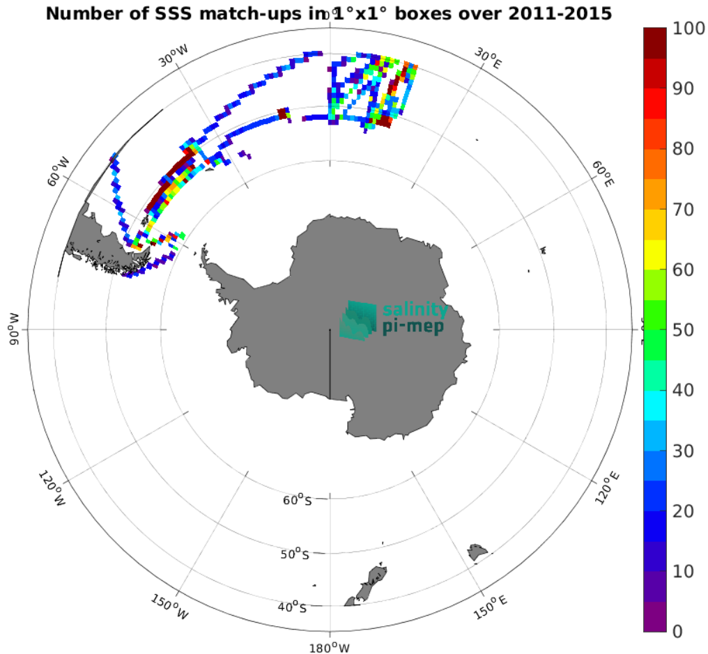
Figure 5: Number of SSS match-ups between TSG (Polarstern) SSS and the Aquarius SSS L4 OI v5 - Weekly (IPRC) SSS product for the Roaring Forties and Furious Fifties Pi-MEP region over 1^\circ \times 1^\circ boxes and for the full satellite product period.
