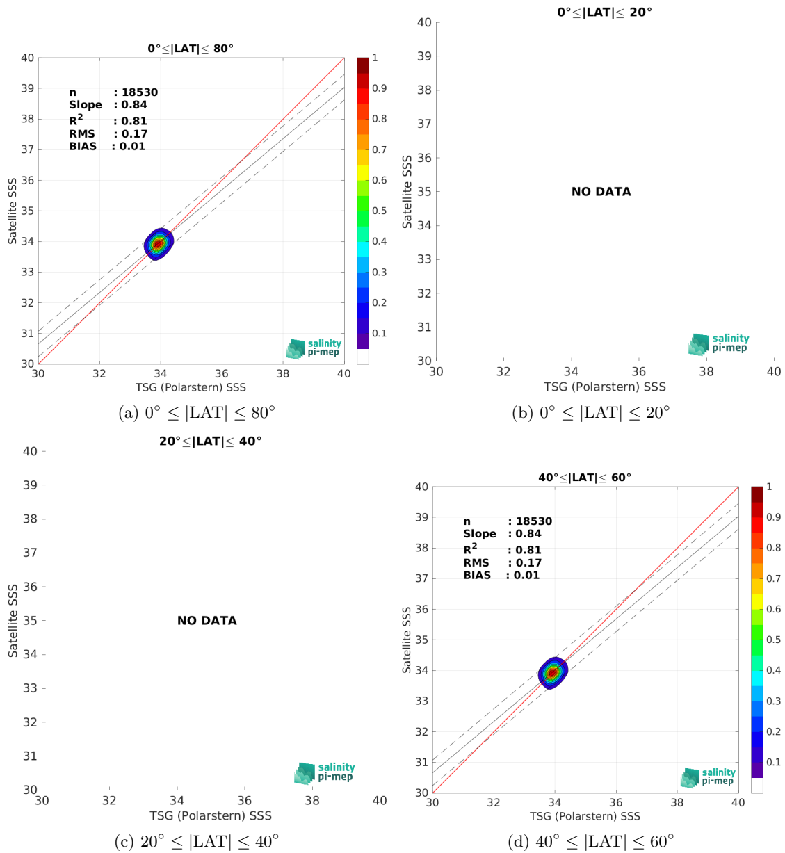
Figure 10: Contour maps of the concentration of Aquarius SSS L4 OI v5 - Weekly (IPRC) SSS (y-axis) versus TSG (Polarstern) SSS (x-axis) at match-up pairs for different latitude bands. For each plot, the red line shows x=y . The black thin and dashed lines indicate a linear fit through the data cloud and the \pm 95\% confidence levels, respectively. The number match-up pairs n , the slope and R^2 coefficient of the linear fit, the root mean square (RMS) and the mean bias between satellite and in situ data are indicated for each latitude band in each plots.
