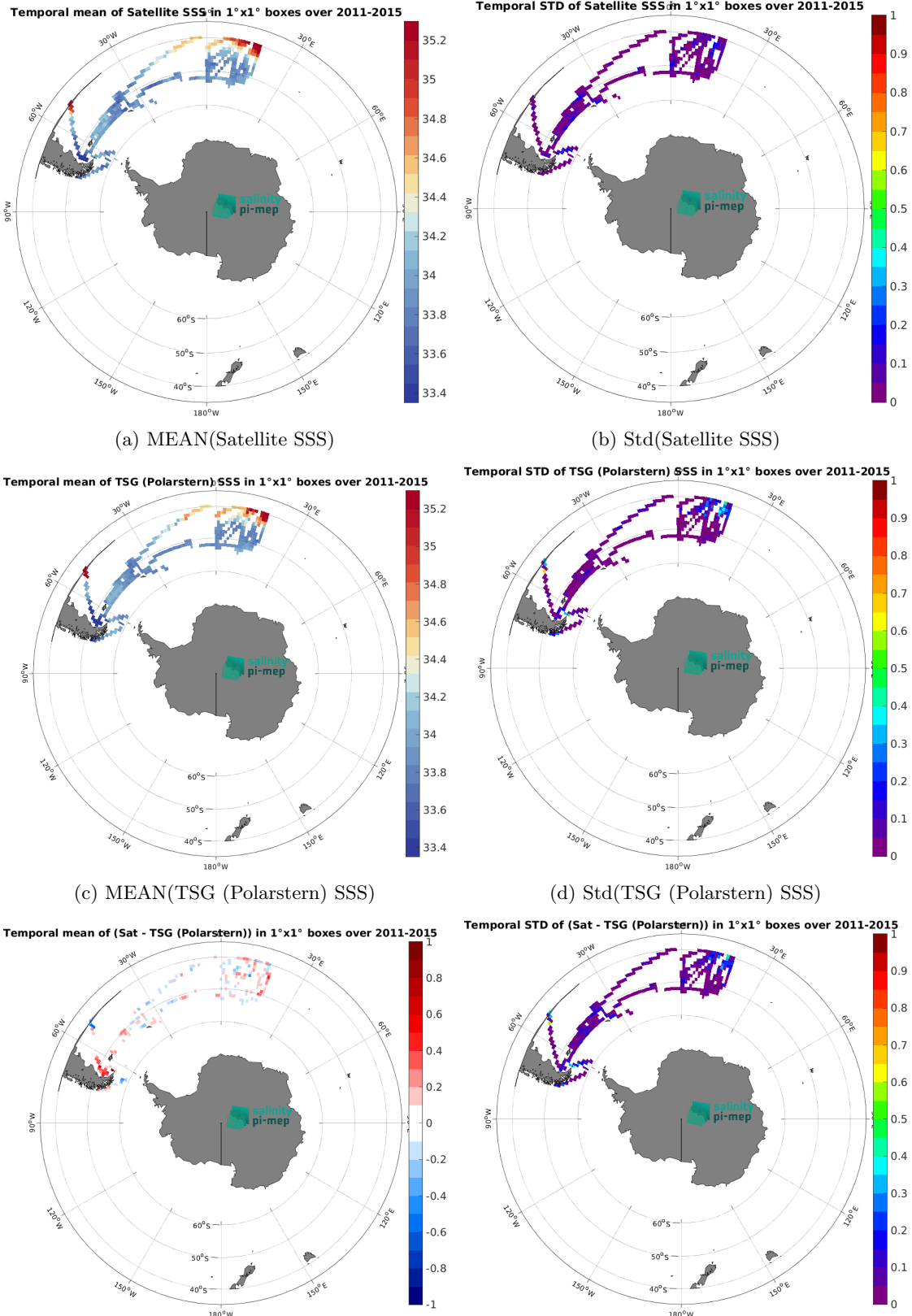
Figure 7: Temporal mean (left) and Std (right) of SSS from Aquarius SSS L4 OI v5 - Weekly (IPRC) (top), TSG (Polarstern) (middle), and of \Delta SSS (Satellite - TSG (Polarstern)). Only match-up pairs are used to generate these maps.
