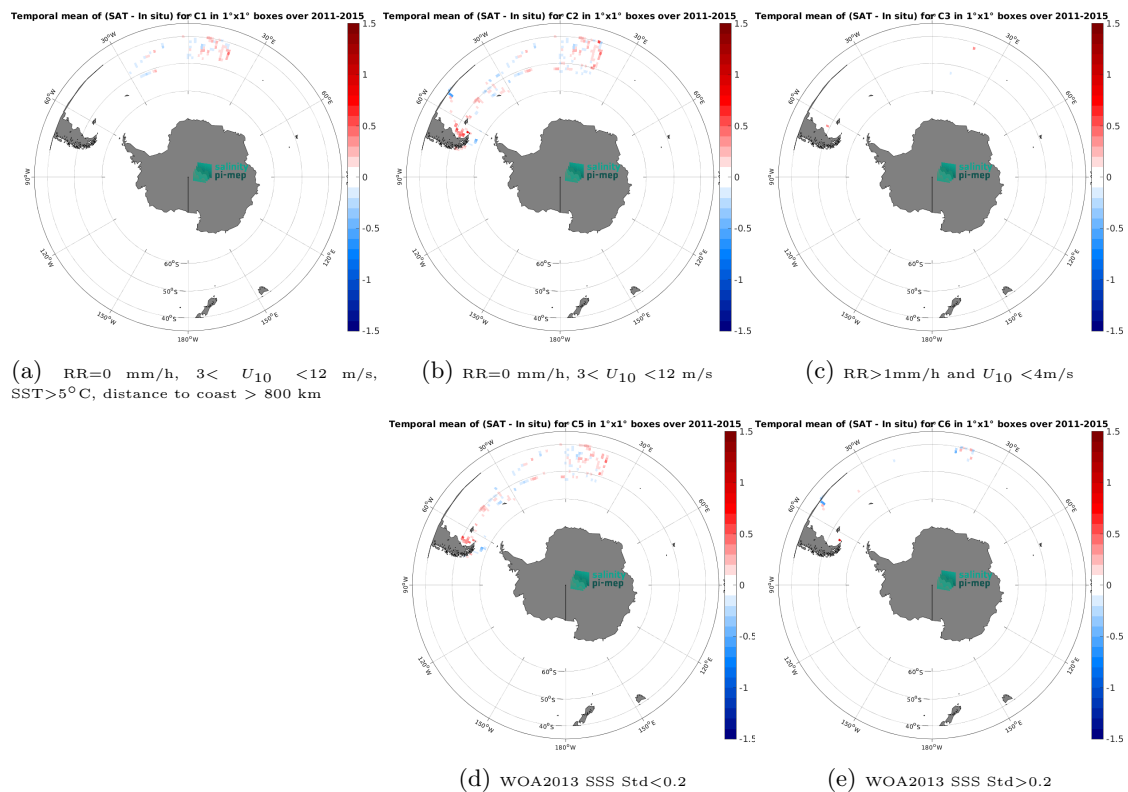
Figure 14: Temporal mean gridded over spatial boxes of size 1^\circ \times 1^\circ of \Delta SSS (Aquarius SSS L4 OI v5 - Weekly (IPRC) - TSG (Polarstern)) for 5 different subdatasets corresponding to:RR=0 mm/h, 3 < U_{10} < 12 m/s, SST >5^\circ C, distance to coast > 800 km (a), RR=0 mm/h, 3 < U_{10} < 12 m/s (b), RR >1 mm/h and U_{10} < 4 m/s (c), WOA2013 SSS Std <0.2 (d), WOA2013 SSS Std >0.2 (e).
