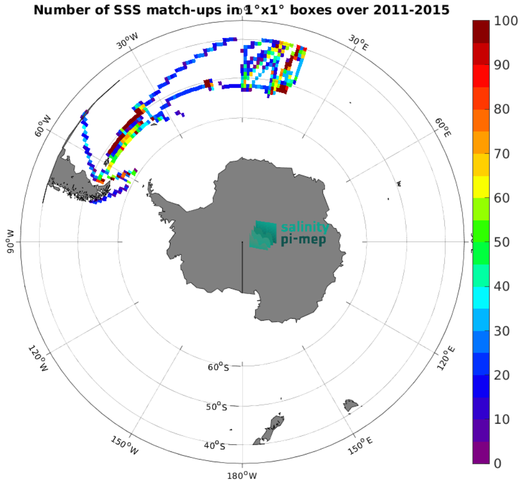
Figure 4: Number of SSS match-ups between TSG (Polarstern) SSS and the Aquarius SSS L4 OI v5 - Weekly (IPRC) SSS product for the Roaring Forties and Furious Fifties Pi-MEP region over 1^\circ \times 1^\circ boxes and for the full satellite product period.
