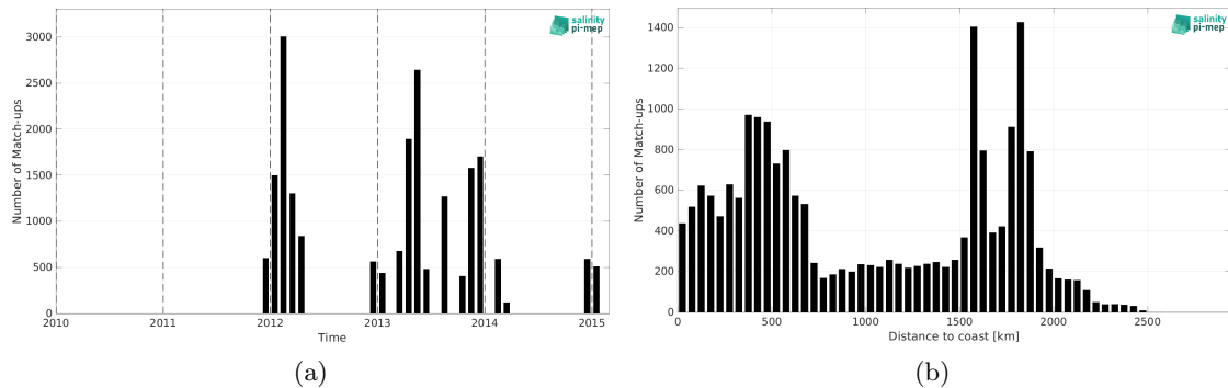
Figure 1: Number of match-ups between TSG (Polarstern) and Aquarius SSS L4 OI v5 - Weekly (IPRC) SSS as a function of time (a) and as function of the distance to coast (b) over the Roaring Forties and Furious Fifties Pi-MEP region and for the full satellite product period.
