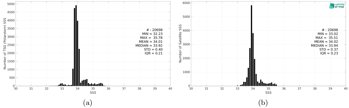
Figure 2: Histograms of SSS from TSG (Polarstern) (a) and Aquarius SSS L4 OI v5 - Weekly (IPRC) (b) considering all match-up pairs per bins of 0.1 over the Roaring Forties and Furious Fifties Pi-MEP region and for the full satellite product period.
