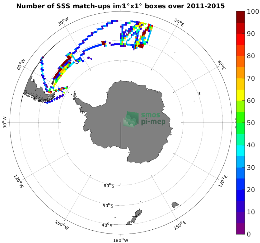
Figure 4: Number of SSS match-ups between TSG (Polarstern) SSS and the Aquarius SSS L4 OI v5 - Weekly (IPRC) SSS product for the Roaring Forties and Furious Fifties Pi-MEP region over 1^\circ \times 1^\circ boxes and for the full satellite product period.
