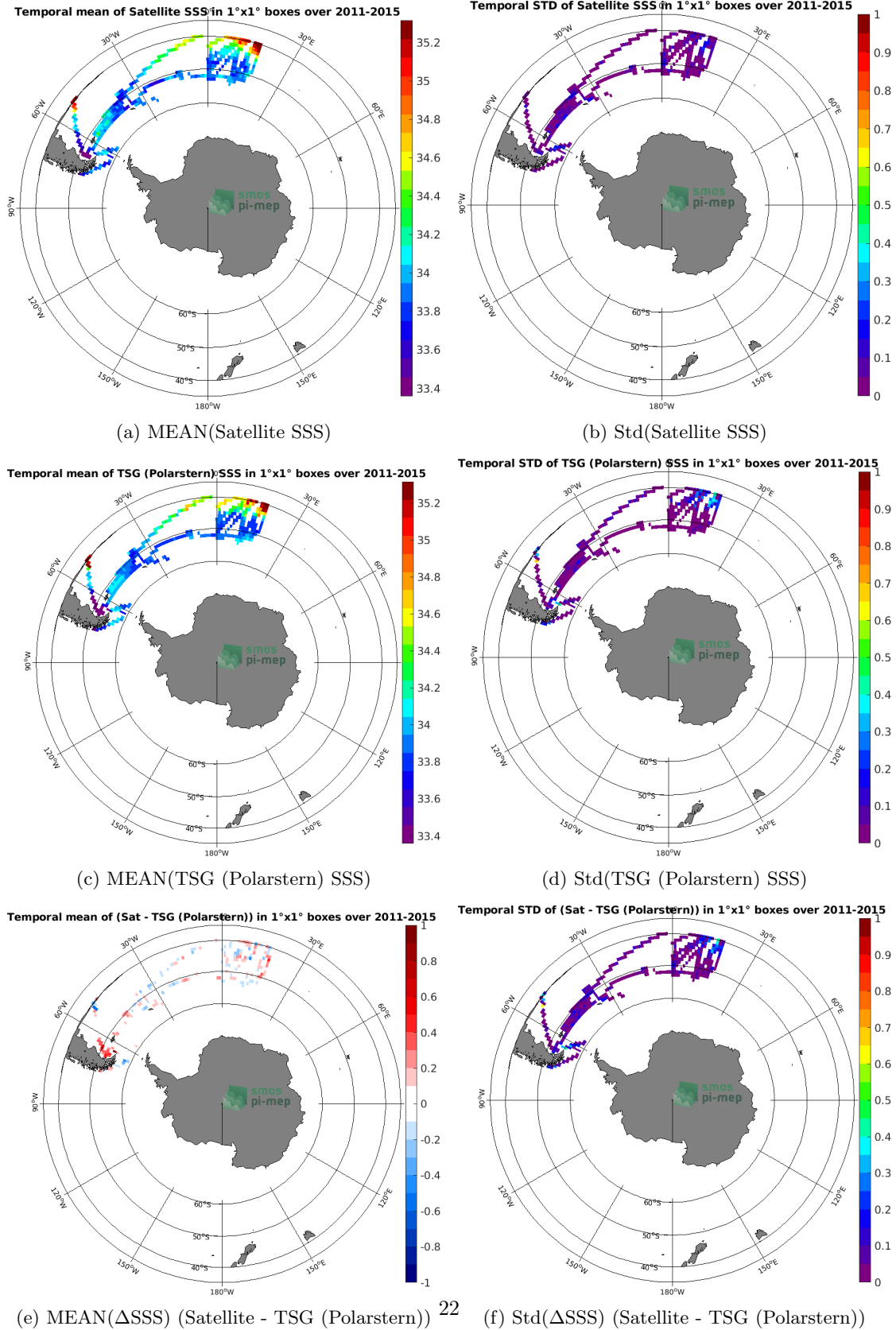
Figure 6: Temporal mean (left) and Std (right) of SSS from Aquarius SSS L4 OI v5 - Weekly (IPRC) (top), TSG (Polarstern) (middle), and of \Delta SSS (Satellite - TSG (Polarstern)). Only match-up pairs are used to generate these maps.
