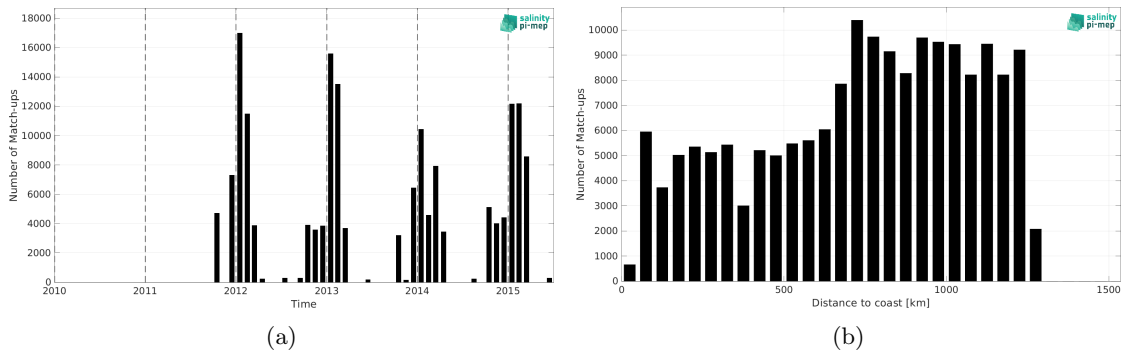
Figure 2: Number of match-ups between TSG (LEGOS-DM) and Aquarius SSS L4 OI v5 - Weekly (IPRC) SSS as a function of time (a) and as function of the distance to coast (b) over the Roaring Forties and Furious Fifties Pi-MEP region and for the full satellite product period.
