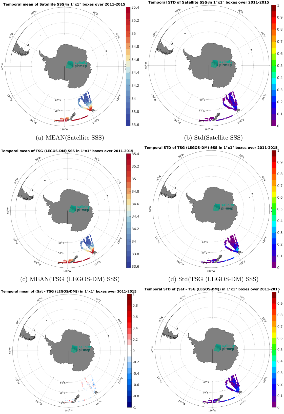
Figure 7: Temporal mean (left) and Std (right) of SSS from Aquarius SSS L4 OI v5 - Weekly (IPRC) (top), TSG (LEGOS-DM) (middle), and of \Delta SSS (Satellite - TSG (LEGOS-DM)). Only match-up pairs are used to generate these maps.
