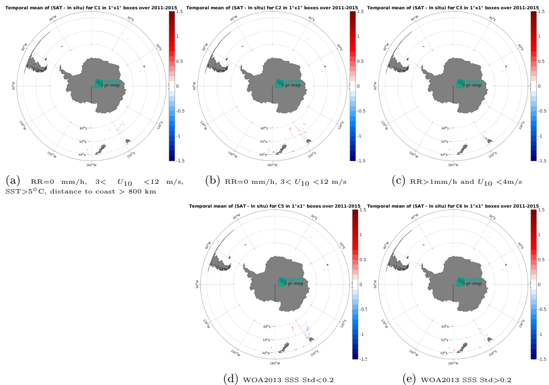
Figure 14: Temporal mean gridded over spatial boxes of size 1^\circ \times 1^\circ of \Delta SSS (Aquarius SSS L4 OI v5 - Weekly (IPRC) - TSG (LEGOS-DM)) for 5 different subdatasets corresponding to:RR=0 mm/h, 3 < U_{10} < 12 m/s, SST > 5^\circ\text{C} , distance to coast > 800 km (a), RR=0 mm/h, 3 < U_{10} < 12 m/s (b), RR > 1 mm/h and U_{10} < 4 m/s (c), WOA2013 SSS Std < 0.2 (d), WOA2013 SSS Std > 0.2 (e).
