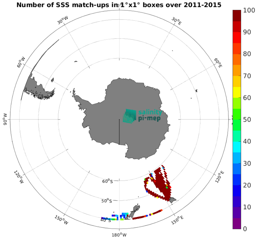
Figure 5: Number of SSS match-ups between TSG (LEGOS-DM) SSS and the Aquarius SSS L4 OI v5 - Weekly (IPRC) SSS product for the Roaring Forties and Furious Fifties Pi-MEP region over 1^\circ \times 1^\circ boxes and for the full satellite product period.
