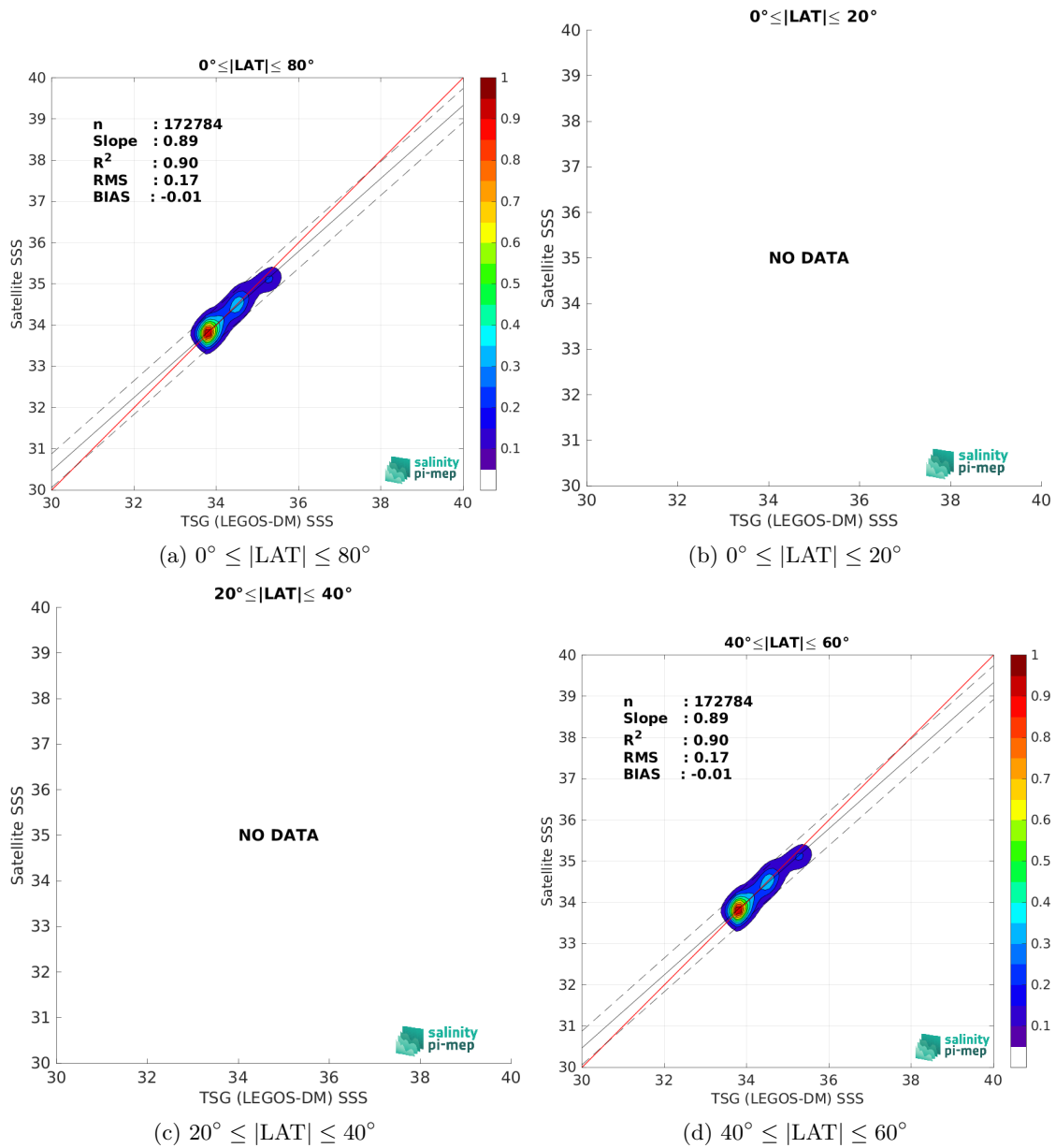
Figure 10: Contour maps of the concentration of Aquarius SSS L4 OI v5 - Weekly (IPRC) SSS (y-axis) versus TSG (LEGOS-DM) SSS (x-axis) at match-up pairs for different latitude bands. For each plot, the red line shows x=y . The black thin and dashed lines indicate a linear fit through the data cloud and the \pm 95\% confidence levels, respectively. The number match-up pairs n , the slope and R^2 coefficient of the linear fit, the root mean square (RMS) and the mean bias between satellite and in situ data are indicated for each latitude band in each plots.
