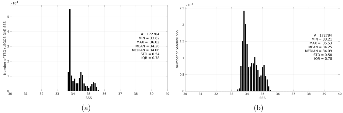
Figure 3: Histograms of SSS from TSG (LEGOS-DM) (a) and Aquarius SSS L4 OI v5 - Weekly (IPRC) (b) considering all match-up pairs per bins of 0.1 over the Roaring Forties and Furious Fifties Pi-MEP region and for the full satellite product period.
