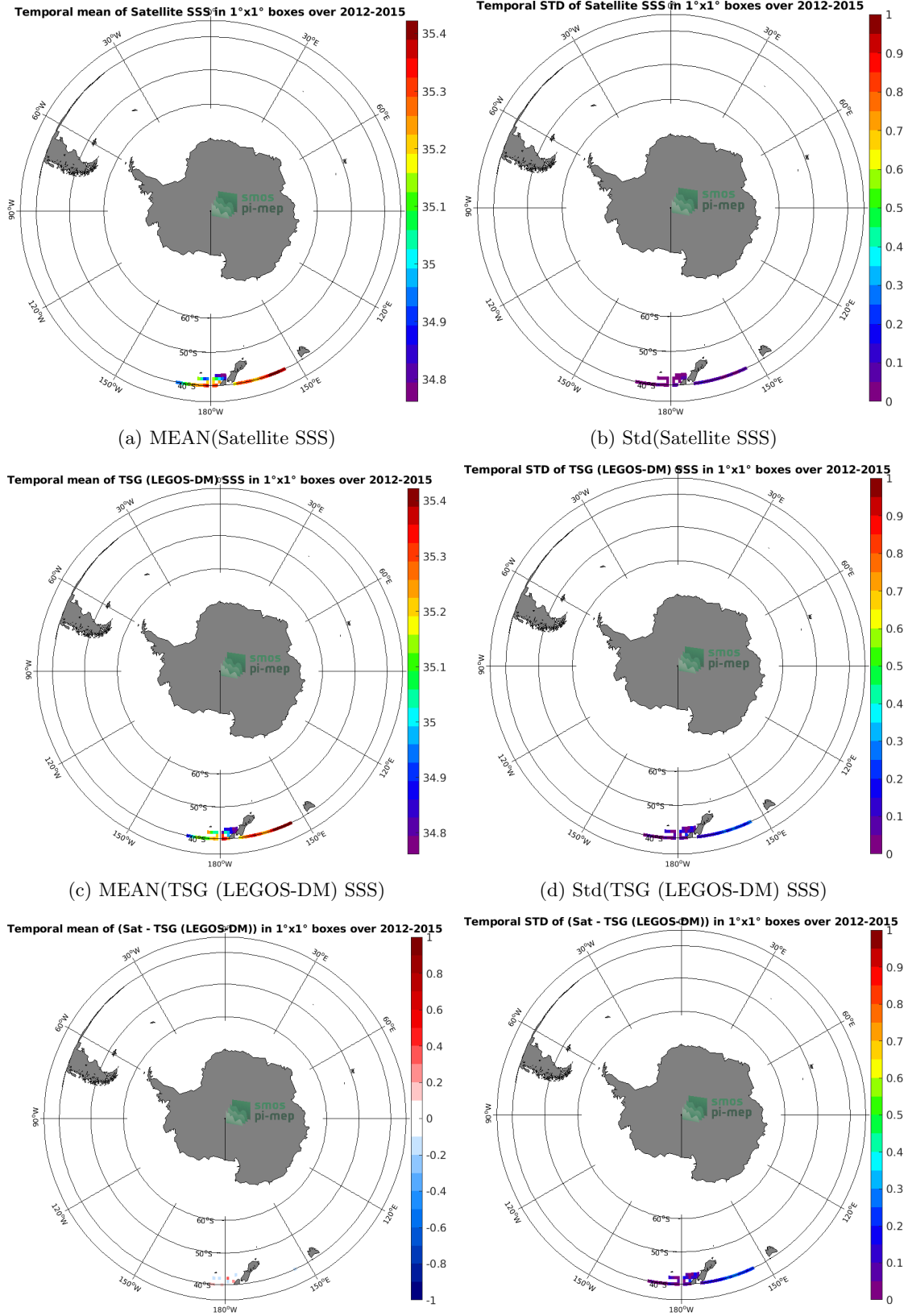
Figure 6: Temporal mean (left) and Std (right) of SSS from Aquarius SSS L4 OI v5 - Weekly (IPRC) (top), TSG (LEGOS-DM) (middle), and of \Delta SSS (Satellite - TSG (LEGOS-DM)). Only match-up pairs are used to generate these maps.
