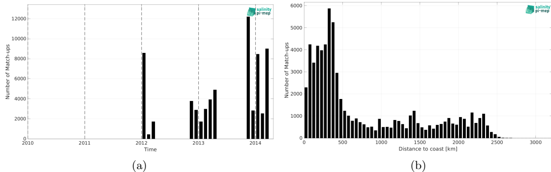
Figure 2: Number of match-ups between TSG (GOSUD-Sailing-ship) and Aquarius SSS L4 OI v5 - Weekly (IPRC) SSS as a function of time (a) and as function of the distance to coast (b) over the Roaring Forties and Furious Fifties Pi-MEP region and for the full satellite product period.
