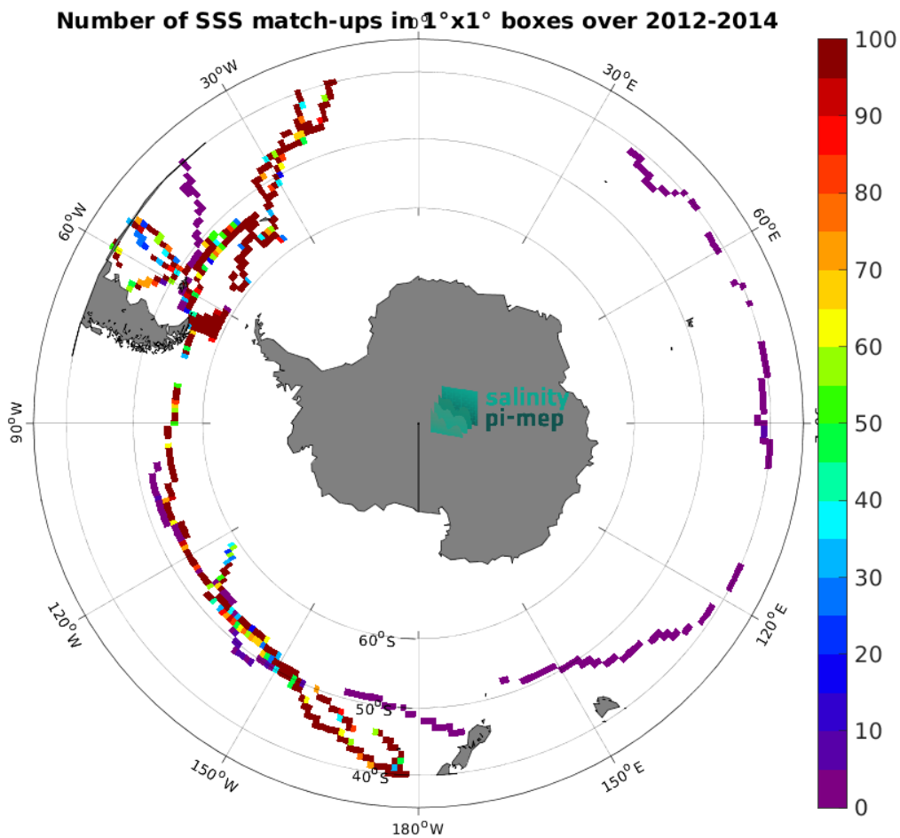
Figure 5: Number of SSS match-ups between TSG (GOSUD-Sailing-ship) SSS and the Aquarius SSS L4 OI v5 - Weekly (IPRC) SSS product for the Roaring Forties and Furious Fifties Pi-MEP region over 1^\circ \times 1^\circ boxes and for the full satellite product period.
