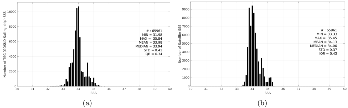
Figure 3: Histograms of SSS from TSG (GOSUD-Sailing-ship) (a) and Aquarius SSS L4 OI v5 - Weekly (IPRC) (b) considering all match-up pairs per bins of 0.1 over the Roaring Forties and Furious Fifties Pi-MEP region and for the full satellite product period.
