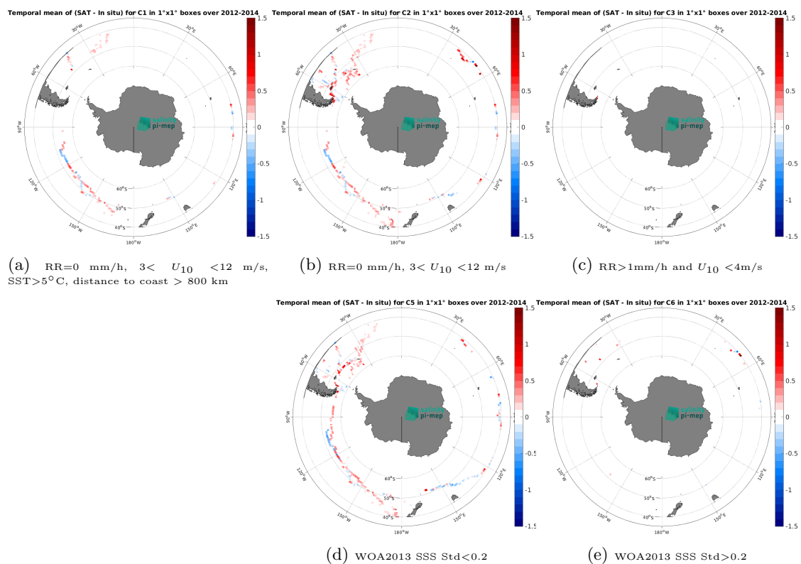
Figure 14: Temporal mean gridded over spatial boxes of size 1^\circ \times 1^\circ of \Delta\text{SSS} (Aquarius SSS L4 OI v5 - Weekly (IPRC) - TSG (GOSUD-Sailing-ship)) for 5 different subdatasets corresponding to: RR=0 mm/h, 3 < U_{10} < 12 m/s, SST > 5°C, distance to coast > 800 km (a), RR=0 mm/h, 3 < U_{10} < 12 m/s (b), RR > 1mm/h and U_{10} < 4 m/s (c), WOA2013 SSS Std < 0.2 (d), WOA2013 SSS Std > 0.2 (e).
