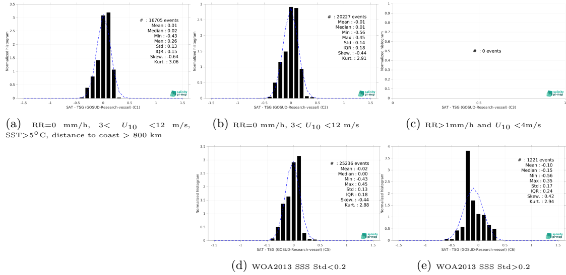
Figure 15: Normalized histogram of \Delta SSS (Aquarius SSS L4 OI v5 - Weekly (IPRC) - TSG (GOSUD-Research-vessel)) for 5 different subdatasets corresponding to: RR=0 mm/h, 3 < U_{10} < 12 m/s, SST > 5°C, distance to coast > 800 km (a), RR=0 mm/h, 3 < U_{10} < 12 m/s (b), RR > 1mm/h and U_{10} < 4 m/s (c), WOA2013 SSS Std < 0.2 (d), WOA2013 SSS Std > 0.2 (e).
