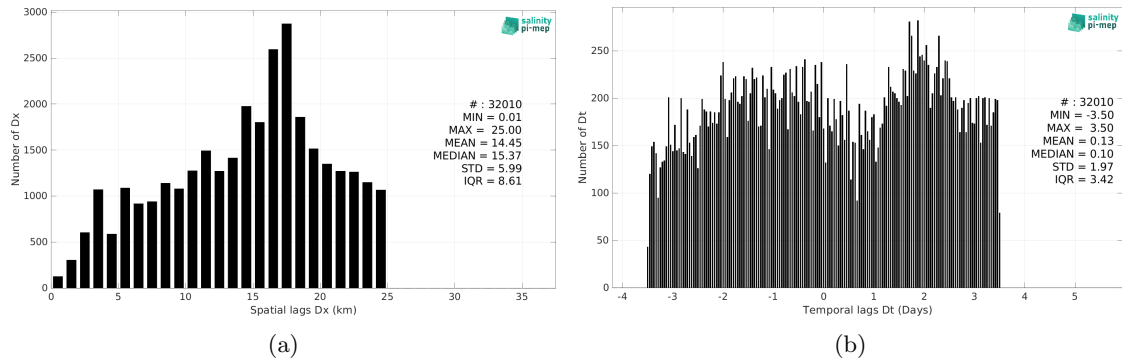
Figure 6: Histograms of the spatial (a) and temporal (b) lags between the location/time of the TSG (GOSUD-Research-vessel) measurement and the date of the corresponding Aquarius SSS L4 OI v5 - Weekly (IPRC) SSS pixel.
