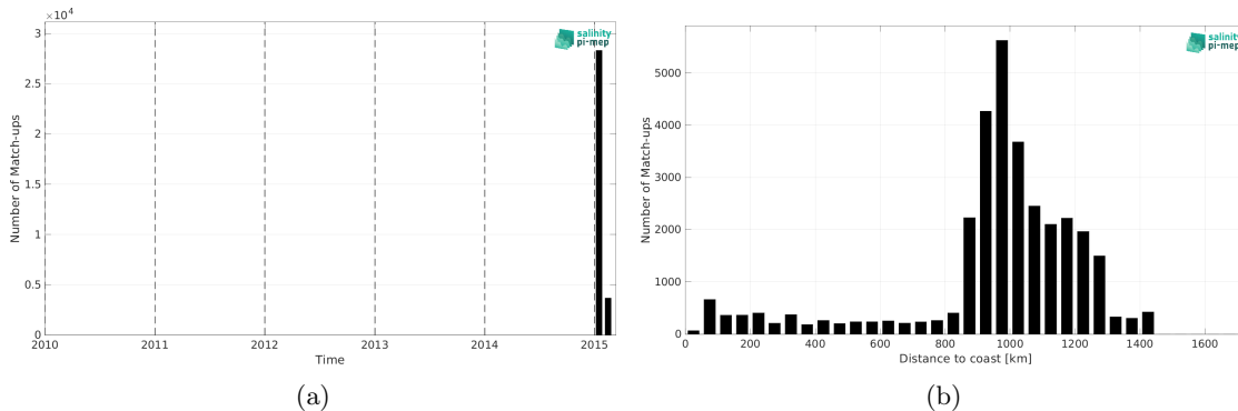
Figure 2: Number of match-ups between TSG (GOSUD-Research-vessel) and Aquarius SSS L4 OI v5 - Weekly (IPRC) SSS as a function of time (a) and as function of the distance to coast (b) over the Roaring Forties and Furious Fifties Pi-MEP region and for the full satellite product period.
