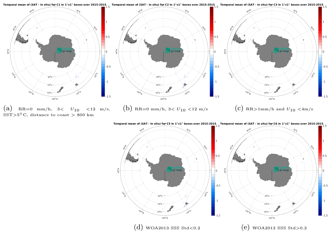
Figure 14: Temporal mean gridded over spatial boxes of size 1^\circ \times 1^\circ of \Delta SSS (Aquarius SSS L4 OI v5 - Weekly (IPRC) - TSG (GOSUD-Research-vessel)) for 5 different subdatasets corresponding to:RR=0 mm/h, 3 < U_{10} < 12 m/s, SST >5^\circ C, distance to coast > 800 km (a), RR=0 mm/h, 3 < U_{10} < 12 m/s (b), RR >1 mm/h and U_{10} < 4 m/s (c), WOA2013 SSS Std <0.2 (d), WOA2013 SSS Std >0.2 (e).
