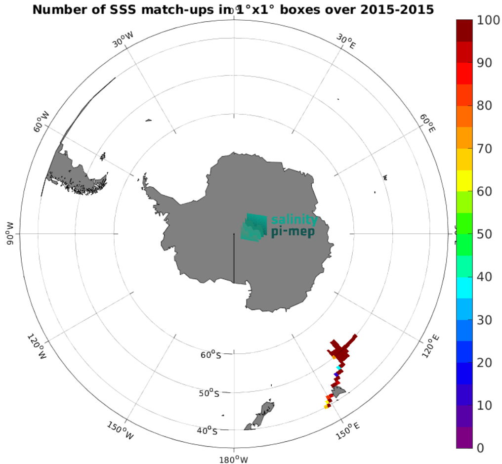
Figure 5: Number of SSS match-ups between TSG (GOSUD-Research-vessel) SSS and the Aquarius SSS L4 OI v5 - Weekly (IPRC) SSS product for the Roaring Forties and Furious Fifties Pi-MEP region over 1^\circ \times 1^\circ boxes and for the full satellite product period.
