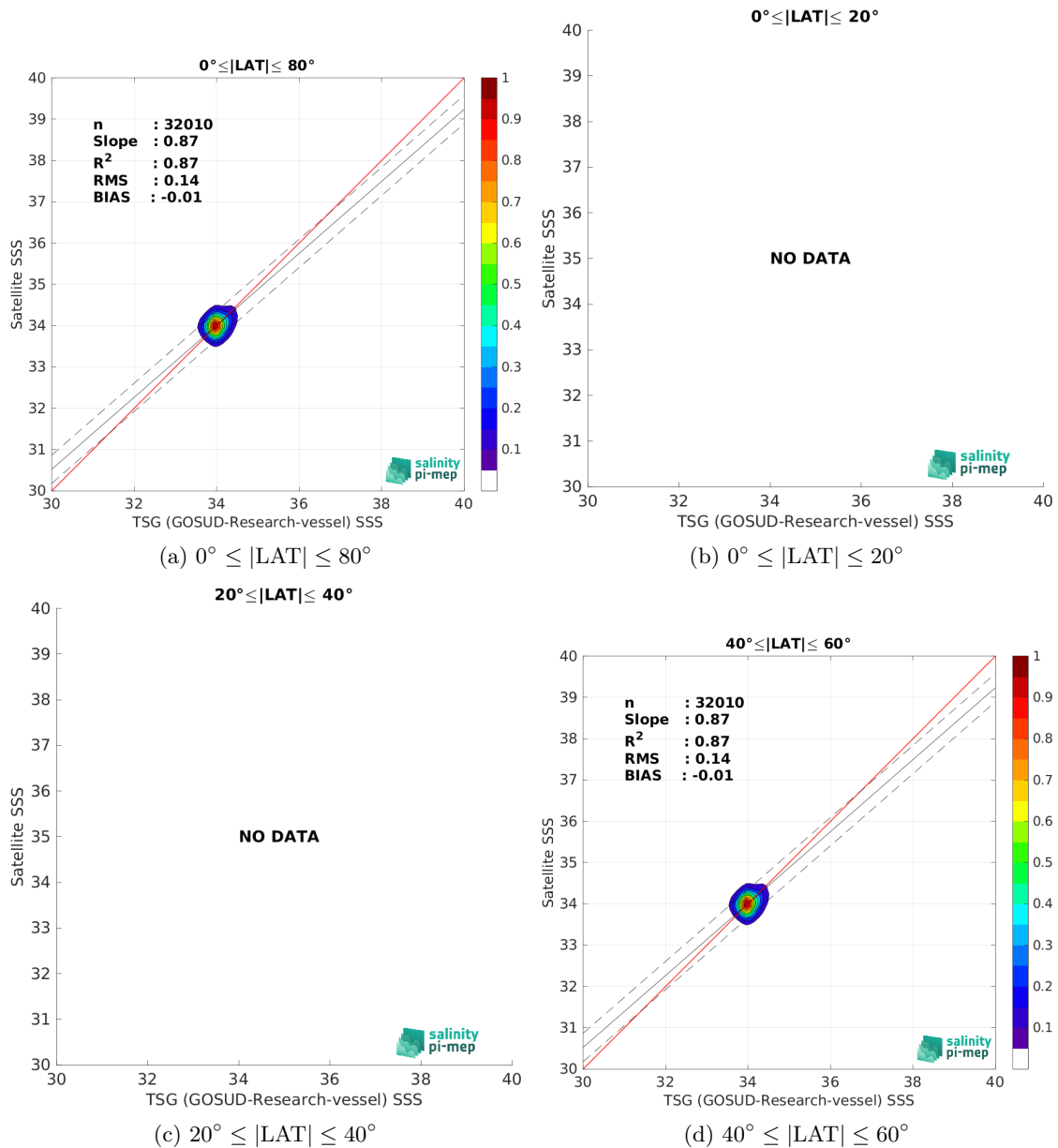
Figure 10: Contour maps of the concentration of Aquarius SSS L4 OI v5 - Weekly (IPRC) SSS (y-axis) versus TSG (GOSUD-Research-vessel) SSS (x-axis) at match-up pairs for different latitude bands. For each plot, the red line shows x=y . The black thin and dashed lines indicate a linear fit through the data cloud and the \pm 95\% confidence levels, respectively. The number match-up pairs n , the slope and R^2 coefficient of the linear fit, the root mean square (RMS) and the mean bias between satellite and in situ data are indicated for each latitude band in each plots.
