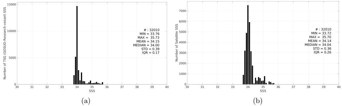
Figure 3: Histograms of SSS from TSG (GOSUD-Research-vessel) (a) and Aquarius SSS L4 OI v5 - Weekly (IPRC) (b) considering all match-up pairs per bins of 0.1 over the Roaring Forties and Furious Fifties Pi-MEP region and for the full satellite product period.
