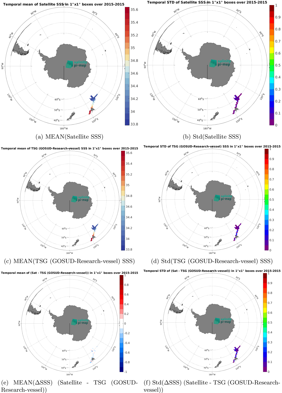
Figure 7: Temporal mean (left) and Std (right) of SSS from Aquarius SSS L4 OI v5 - Weekly (IPRC) (top), TSG (GOSUD-Research-vessel) (middle), and of \Delta SSS (Satellite - TSG (GOSUD-Research-vessel)). Only match-up pairs are used to generate these maps.
