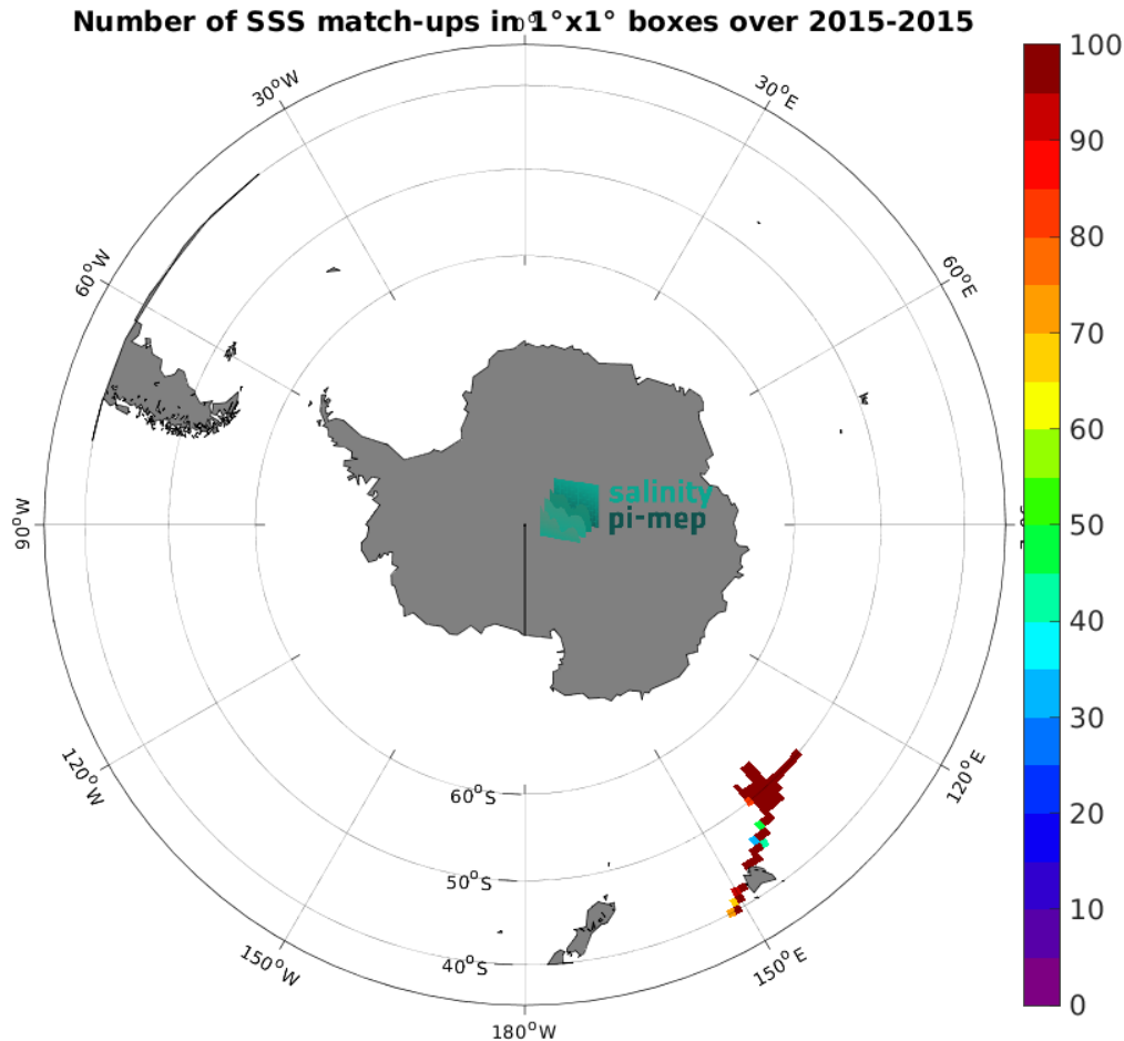
Figure 4: Number of SSS match-ups between TSG (GOSUD-Research-vessel) SSS and the Aquarius SSS L4 OI v5 - Weekly (IPRC) SSS product for the Roaring Forties and Furious Fifties Pi-MEP region over 1^\circ \times 1^\circ boxes and for the full satellite product period.
