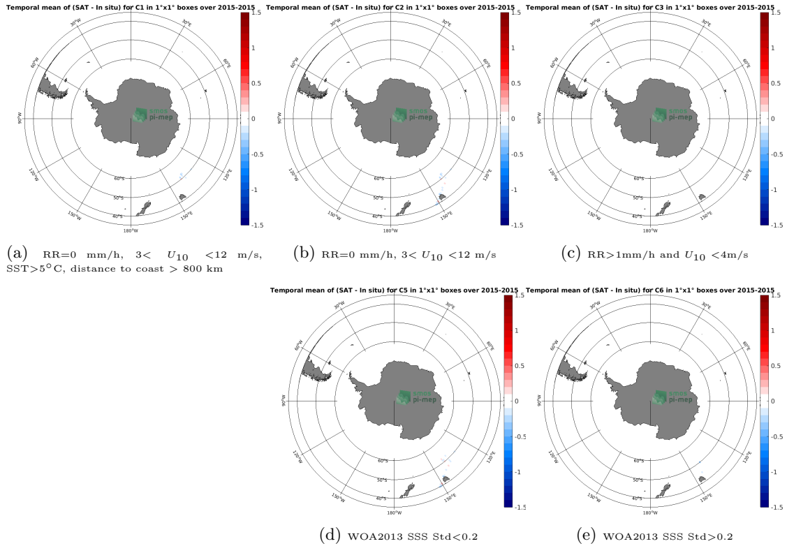
Figure 12: Temporal mean gridded over spatial boxes of size 1°x1° of \Delta SSS (Aquarius SSS L4 OI v5 - Weekly (IPRC) - TSG (GOSUD-Research-vessel)) for 5 different subdatasets corresponding to:RR=0 mm/h, 3 < U_{10} < 12 m/s, SST>5°C, distance to coast > 800 km (a), RR=0 mm/h, 3 < U_{10} < 12 m/s (b), RR>1mm/h and U_{10} < 4 m/s (c), WOA2013 SSS Std<0.2 (d), WOA2013 SSS Std>0.2 (e).
