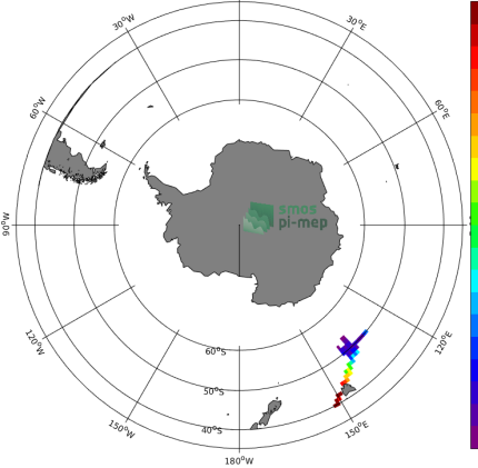
(c) MEAN(TSG-GOSUD-Research-vessel SSS)
