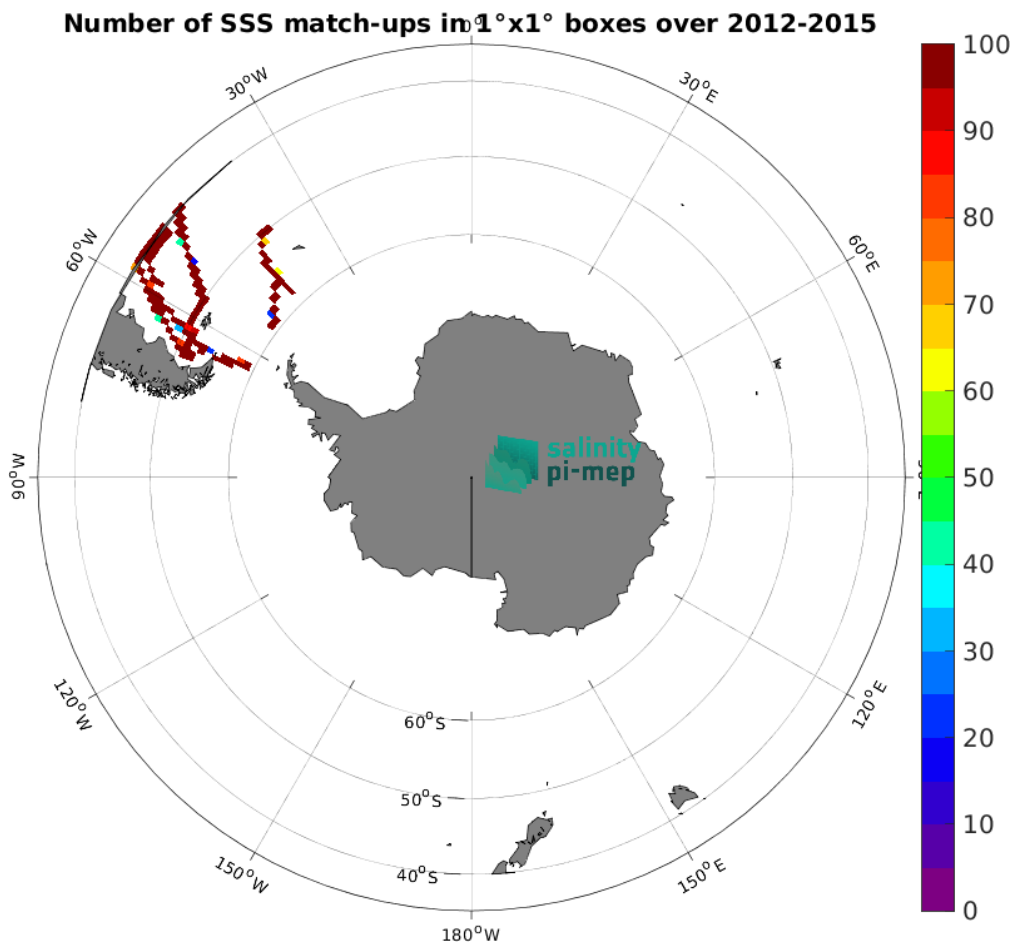
Figure 5: Number of SSS match-ups between TSG (CSIC-UTM) SSS and the Aquarius SSS L4 OI v5 - Weekly (IPRC) SSS product for the Roaring Forties and Furious Fifties Pi-MEP region over 1^{\circ} \times 1^{\circ} boxes and for the full satellite product period.
