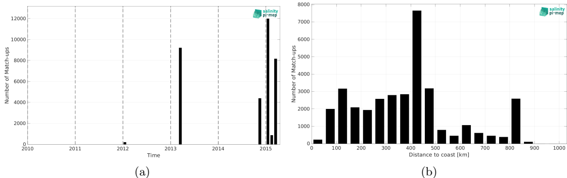
Figure 2: Number of match-ups between TSG (CSIC-UTM) and Aquarius SSS L4 OI v5 - Weekly (IPRC) SSS as a function of time (a) and as function of the distance to coast (b) over the Roaring Forties and Furious Fifties Pi-MEP region and for the full satellite product period.
