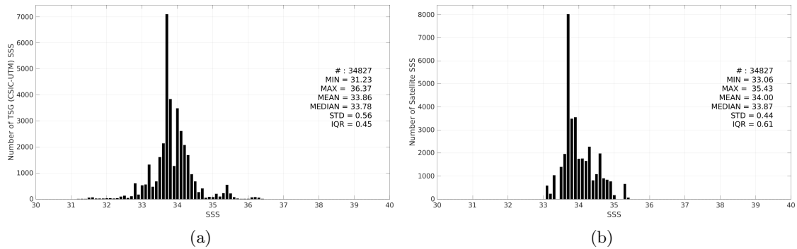
Figure 3: Histograms of SSS from TSG (CSIC-UTM) (a) and Aquarius SSS L4 OI v5 - Weekly (IPRC) (b) considering all match-up pairs per bins of 0.1 over the Roaring Forties and Furious Fifties Pi-MEP region and for the full satellite product period.
