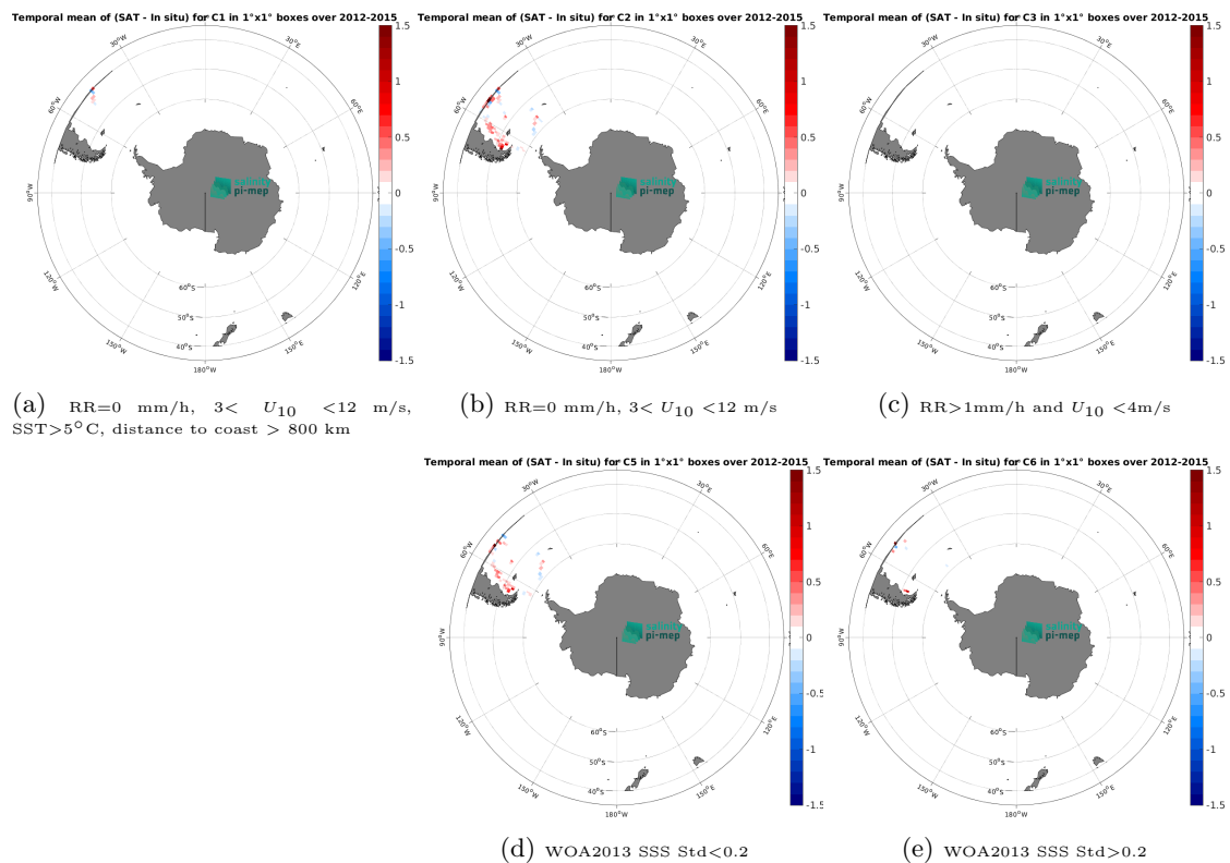
Figure 14: Temporal mean gridded over spatial boxes of size 1^\circ \times 1^\circ of \Delta\text{SSS} (Aquarius SSS L4 OI v5 - Weekly (IPRC) - TSG (CSIC-UTM)) for 5 different subdatasets corresponding to:RR=0 mm/h, 3 < U_{10} < 12 m/s, SST>5°C, distance to coast > 800 km (a), RR=0 mm/h, 3 < U_{10} < 12 m/s (b), RR>1mm/h and U_{10} < 4 m/s (c), WOA2013 SSS Std<0.2 (d), WOA2013 SSS Std>0.2 (e).
