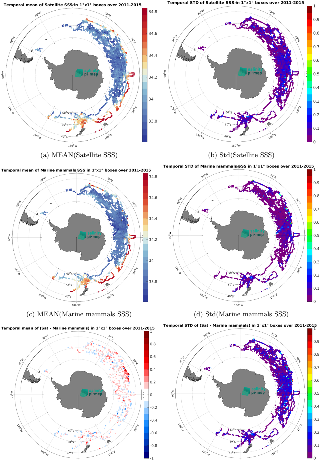
(e) MEAN( \Delta SSS) (Satellite - Marine mammals) 16 (f) Std( \Delta SSS) (Satellite - Marine mammals) Figure 7: Temporal mean (left) and Std (right) of SSS from Aquarius SSS L4 OI v5 - Weekly (IPRC) (top), Marine mammals (middle), and of \Delta SSS (Satellite - Marine mammals). Only match-up pairs are used to generate these maps.
