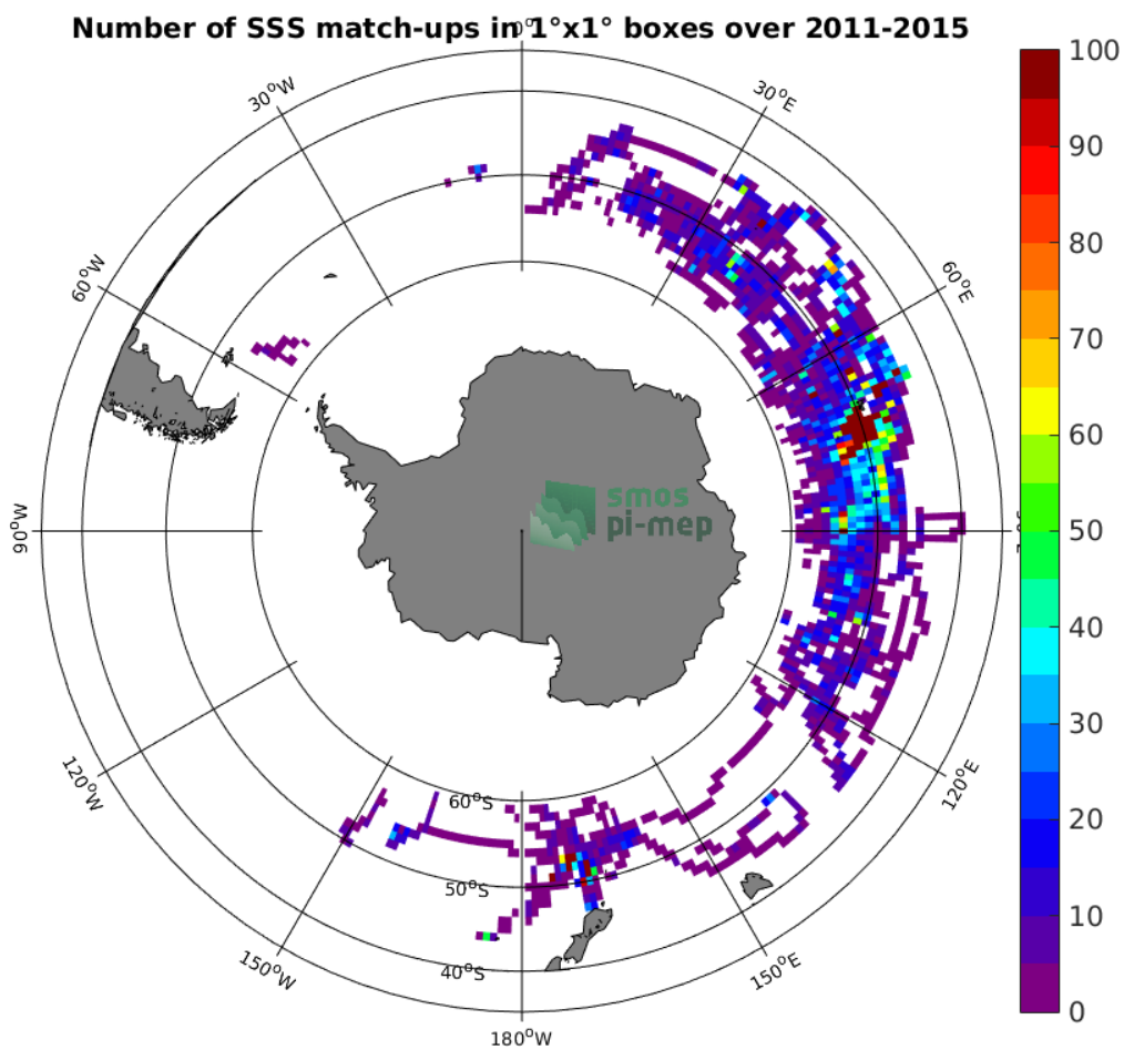
Figure 4: Number of SSS match-ups between Sea mammals SSS and the Aquarius-L4-IPRC-V5-WEEKLY SSS product for the Roaring Forties and Furious Fifties Pi-MEP region over 1^\circ \times 1^\circ boxes and for the full satellite product period.
