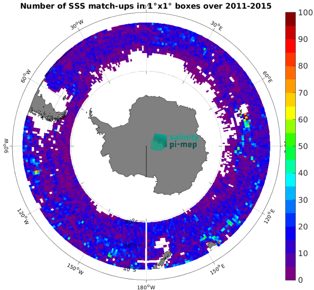
Figure 5: Number of SSS match-ups between Argo SSS and the Aquarius SSS L4 OI v5 - Weekly (IPRC) SSS product for the Roaring Forties and Furious Fifties Pi-MEP region over 1^\circ \times 1^\circ boxes and for the full satellite product period.
