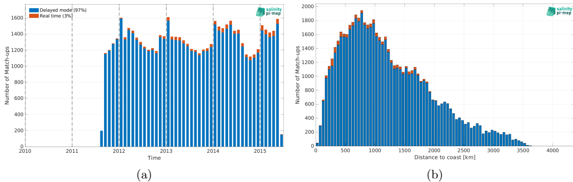
Figure 2: Number of match-ups between Argo and Aquarius SSS L4 OI v5 - Weekly (IPRC) SSS as a function of time (a) and as function of the distance to coast (b) over the Roaring Forties and Furious Fifties Pi-MEP region and for the full satellite product period.
