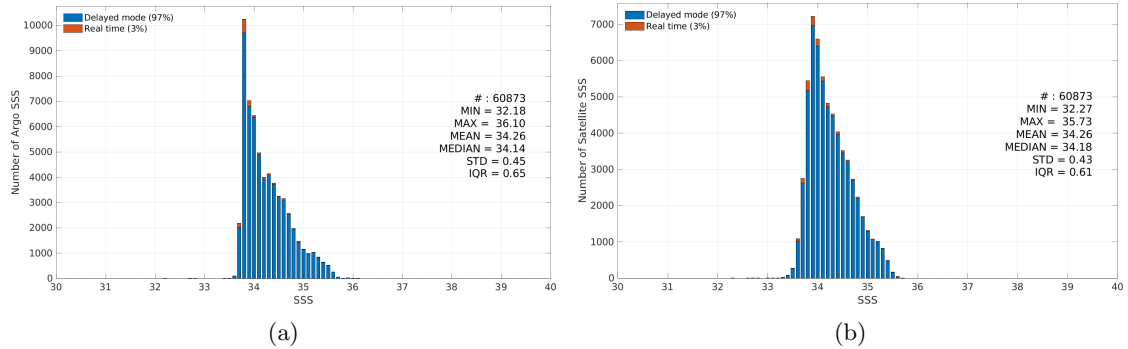
Figure 3: Histograms of SSS from Argo (a) and Aquarius SSS L4 OI v5 - Weekly (IPRC) (b) considering all match-up pairs per bins of 0.1 over the Roaring Forties and Furious Fifties Pi-MEP region and for the full satellite product period.
