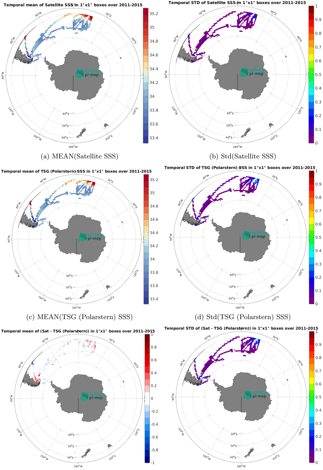
Figure 6: Temporal mean (left) and Std (right) of SSS from Aquarius SSS L4 OI v5 - Monthly (IPRC) (top), TSG (Polarstern) (middle), and of \Delta SSS (Satellite - TSG (Polarstern)). Only match-up pairs are used to generate these maps.
