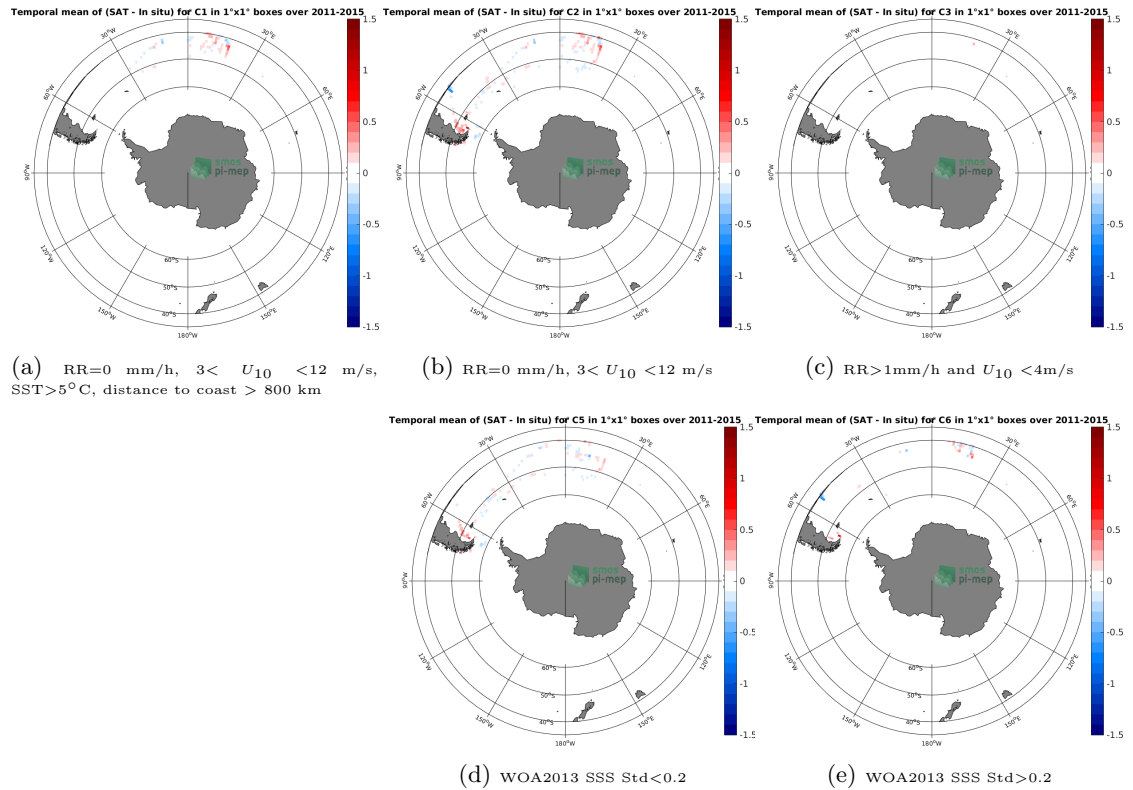
Figure 12: Temporal mean gridded over spatial boxes of size 1^{\circ}\times 1^{\circ} of \Delta\text{SSS} (Aquarius-L4-IPRC-V5-MONTHLY - TSG-POLARSTERN) for 5 different subdatasets corresponding to:RR=0 mm/h, 3 < U_{10} < 12 m/s, \text{SST}>5^{\circ}\text{C} , distance to coast > 800 km (a), RR=0 mm/h, 3 < U_{10} < 12 m/s (b), RR >1 mm/h and U_{10} < 4 m/s (c), WOA2013 SSS Std <0.2 (d), WOA2013 SSS Std >0.2 (e).
