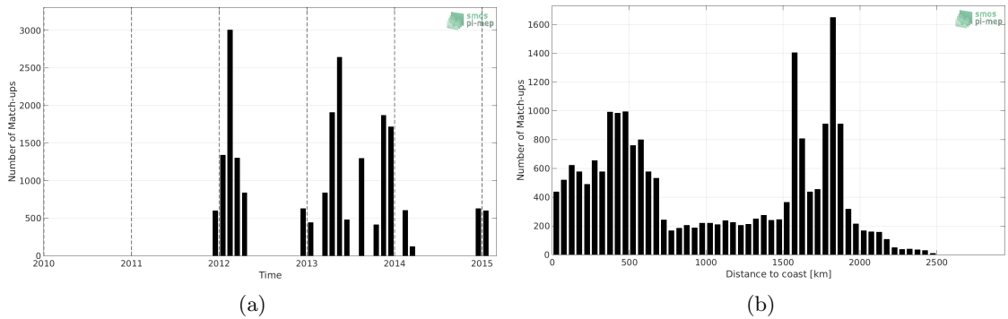
Figure 1: Number of match-ups between TSG-POLARSTERN and Aquarius-L4-IPRC-V5-MONTHLY SSS as a function of time (a) and as function of the distance to coast (b) over the Roaring Forties and Furious Fifties Pi-MEP region and for the full satellite product period.
