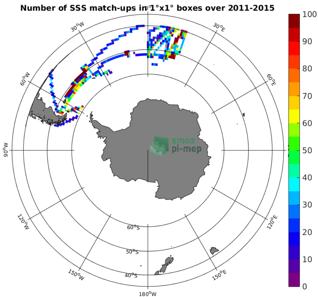
Figure 4: Number of SSS match-ups between TSG-POLARSTERN SSS and the Aquarius-L4-IPRC-V5-MONTHLY SSS product for the Roaring Forties and Furious Fifties Pi-MEP region over 1^\circ \times 1^\circ boxes and for the full satellite product period.
