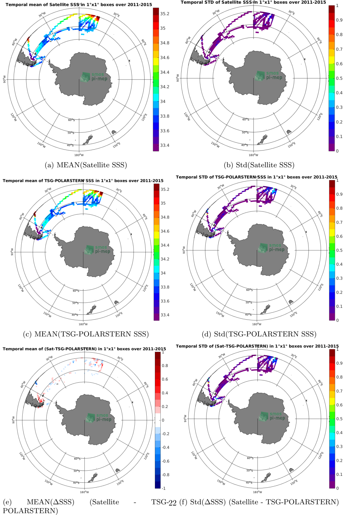
Figure 6: Temporal mean (left) and Std (right) of SSS from Aquarius-L4-IPRC-V5-MONTHLY (top), TSG-POLARSTERN (middle), and of \Delta SSS (Satellite - TSG-POLARSTERN). Only match-up pairs are used to generate these maps.
