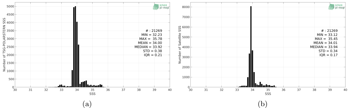
Figure 2: Histograms of SSS from TSG-POLARSTERN (a) and Aquarius-L4-IPRC-V5-MONTHLY (b) considering all match-up pairs per bins of 0.1 over the Roaring Forties and Furious Fifties Pi-MEP region and for the full satellite product period.
