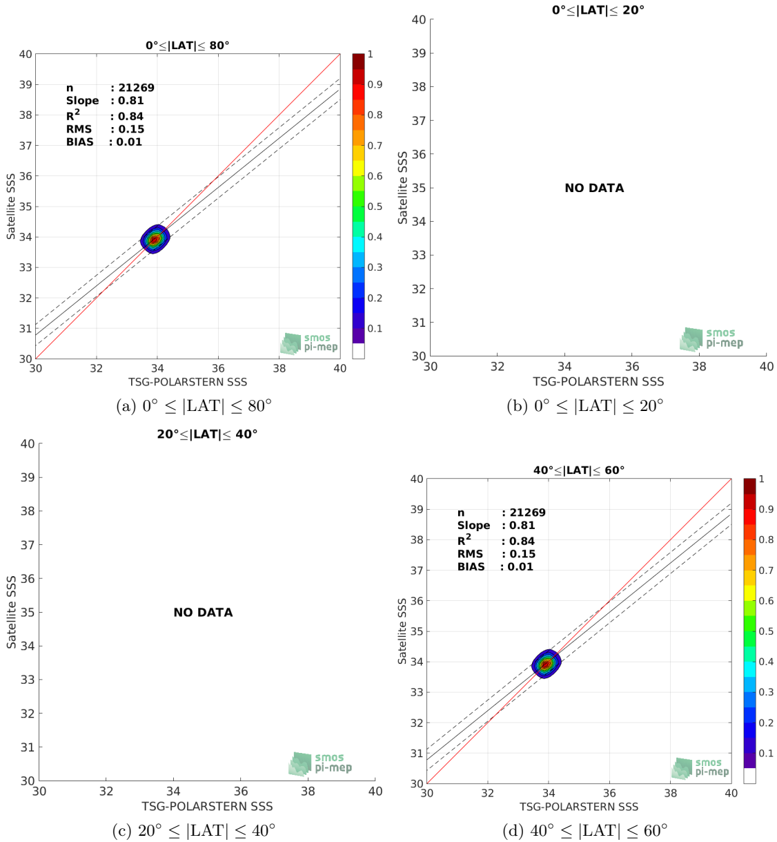
Figure 9: Contour maps of the concentration of Aquarius-L4-IPRC-V5-MONTHLY SSS (y-axis) versus TSG-POLARSTERN SSS (x-axis) at match-up pairs for different latitude bands. For each plot, the red line shows x=y . The black thin and dashed lines indicate a linear fit through the data cloud and the \pm 95\% confidence levels, respectively. The number match-up pairs n , the slope and R^2 coefficient of the linear fit, the root mean square (RMS) and the mean bias between satellite and in situ data are indicated for each latitude band in each plots.
