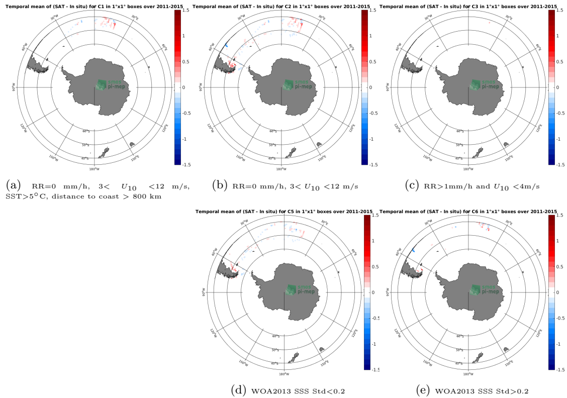
Figure 12: Temporal mean gridded over spatial boxes of size 1^\circ \times 1^\circ of \Delta SSS (Aquarius-L4-IPRC-V5-MONTHLY - TSG-POLARSTERN) for 5 different subdatasets corresponding to:RR=0 mm/h, 3 < U_{10} < 12 m/s, SST >5^\circ C, distance to coast > 800 km (a), RR=0 mm/h, 3 < U_{10} < 12 m/s (b), RR >1 mm/h and U_{10} < 4 m/s (c), WOA2013 SSS Std <0.2 (d), WOA2013 SSS Std >0.2 (e).
