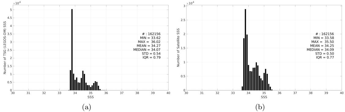
Figure 3: Histograms of SSS from TSG (LEGOS-DM) (a) and Aquarius SSS L4 OI v5 - Monthly (IPRC) (b) considering all match-up pairs per bins of 0.1 over the Roaring Forties and Furious Fifties Pi-MEP region and for the full satellite product period.
