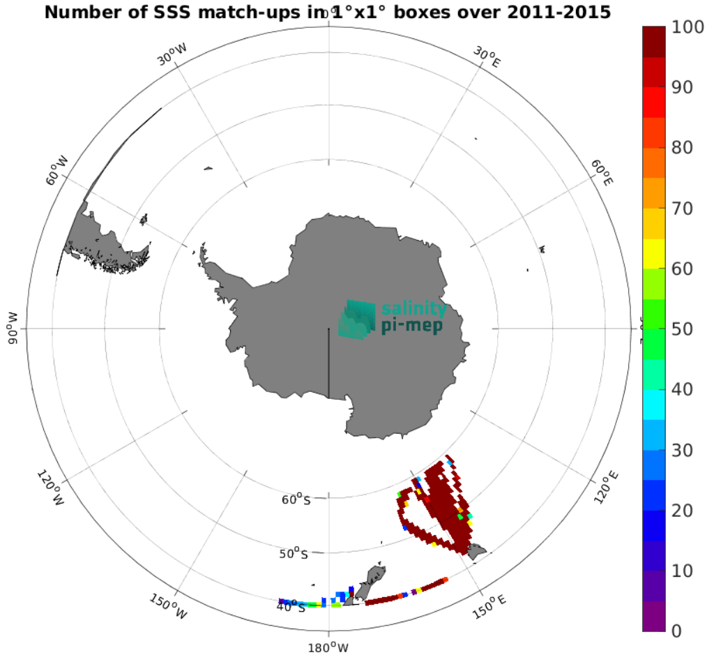
Figure 5: Number of SSS match-ups between TSG (LEGOS-DM) SSS and the Aquarius SSS L4 OI v5 - Monthly (IPRC) SSS product for the Roaring Forties and Furious Fifties Pi-MEP region over 1^\circ \times 1^\circ boxes and for the full satellite product period.
