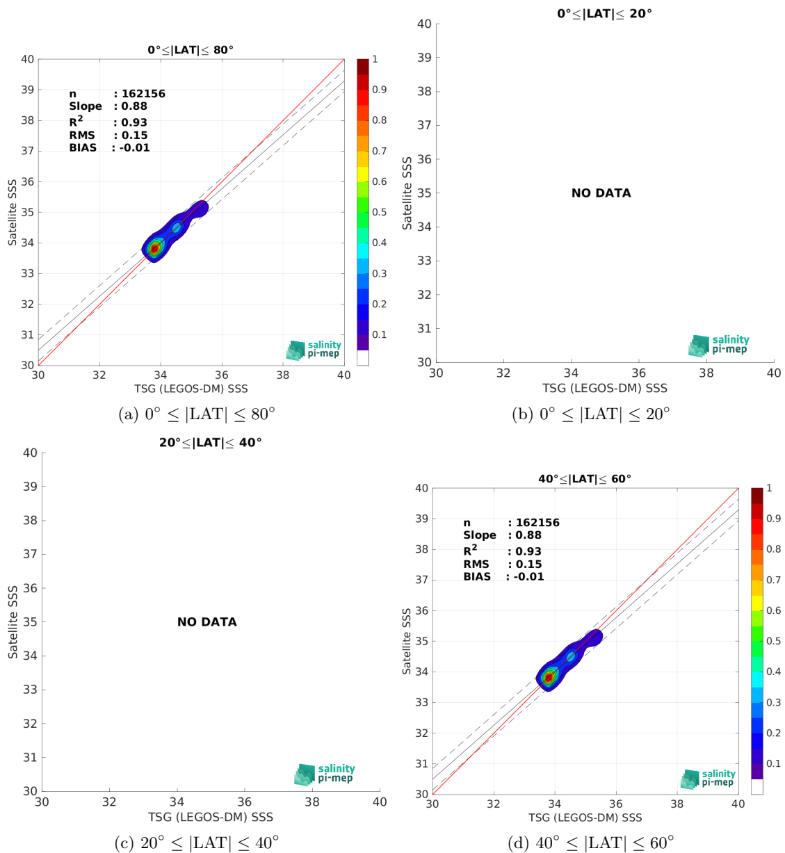
Figure 10: Contour maps of the concentration of Aquarius SSS L4 OI v5 - Monthly (IPRC) SSS (y-axis) versus TSG (LEGOS-DM) SSS (x-axis) at match-up pairs for different latitude bands. For each plot, the red line shows x=y . The black thin and dashed lines indicate a linear fit through the data cloud and the \pm 95\% confidence levels, respectively. The number match-up pairs n , the slope and R^2 coefficient of the linear fit, the root mean square (RMS) and the mean bias between satellite and in situ data are indicated for each latitude band in each plots.
