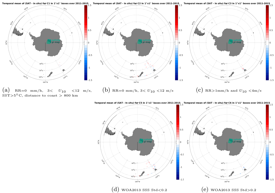
Figure 14: Temporal mean gridded over spatial boxes of size 1^\circ \times 1^\circ of \Delta SSS (Aquarius SSS L4 OI v5 - Monthly (IPRC) - TSG (LEGOS-DM)) for 5 different subdatasets corresponding to:RR=0 mm/h, 3 < U_{10} < 12 m/s, SST>5°C, distance to coast > 800 km (a), RR=0 mm/h, 3 < U_{10} < 12 m/s (b), RR>1mm/h and U_{10} < 4 m/s (c), WOA2013 SSS Std<0.2 (d), WOA2013 SSS Std>0.2 (e).
