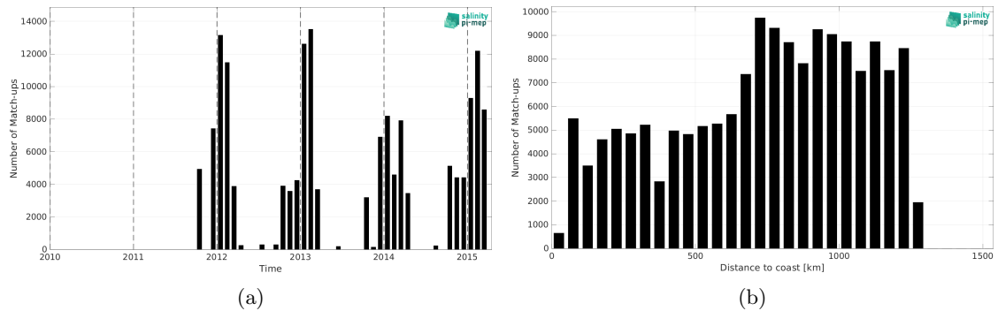
Figure 2: Number of match-ups between TSG (LEGOS-DM) and Aquarius SSS L4 OI v5 - Monthly (IPRC) SSS as a function of time (a) and as function of the distance to coast (b) over the Roaring Forties and Furious Fifties Pi-MEP region and for the full satellite product period.
