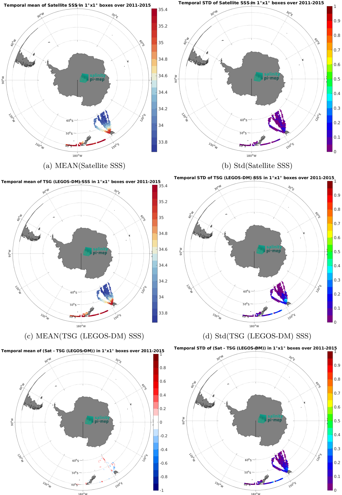
Figure 7: Temporal mean (left) and Std (right) of SSS from Aquarius SSS L4 OI v5 - Monthly (IPRC) (top), TSG (LEGOS-DM) (middle), and of \Delta SSS (Satellite - TSG (LEGOS-DM)). Only match-up pairs are used to generate these maps.
