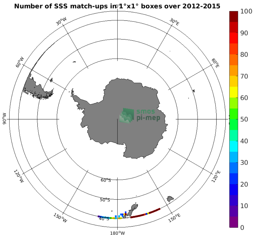
Figure 4: Number of SSS match-ups between TSG (LEGOS-DM) SSS and the Aquarius SSS L4 OI v5 - Monthly (IPRC) SSS product for the Roaring Forties and Furious Fifties Pi-MEP region over 1°x1° boxes and for the full satellite product period.
