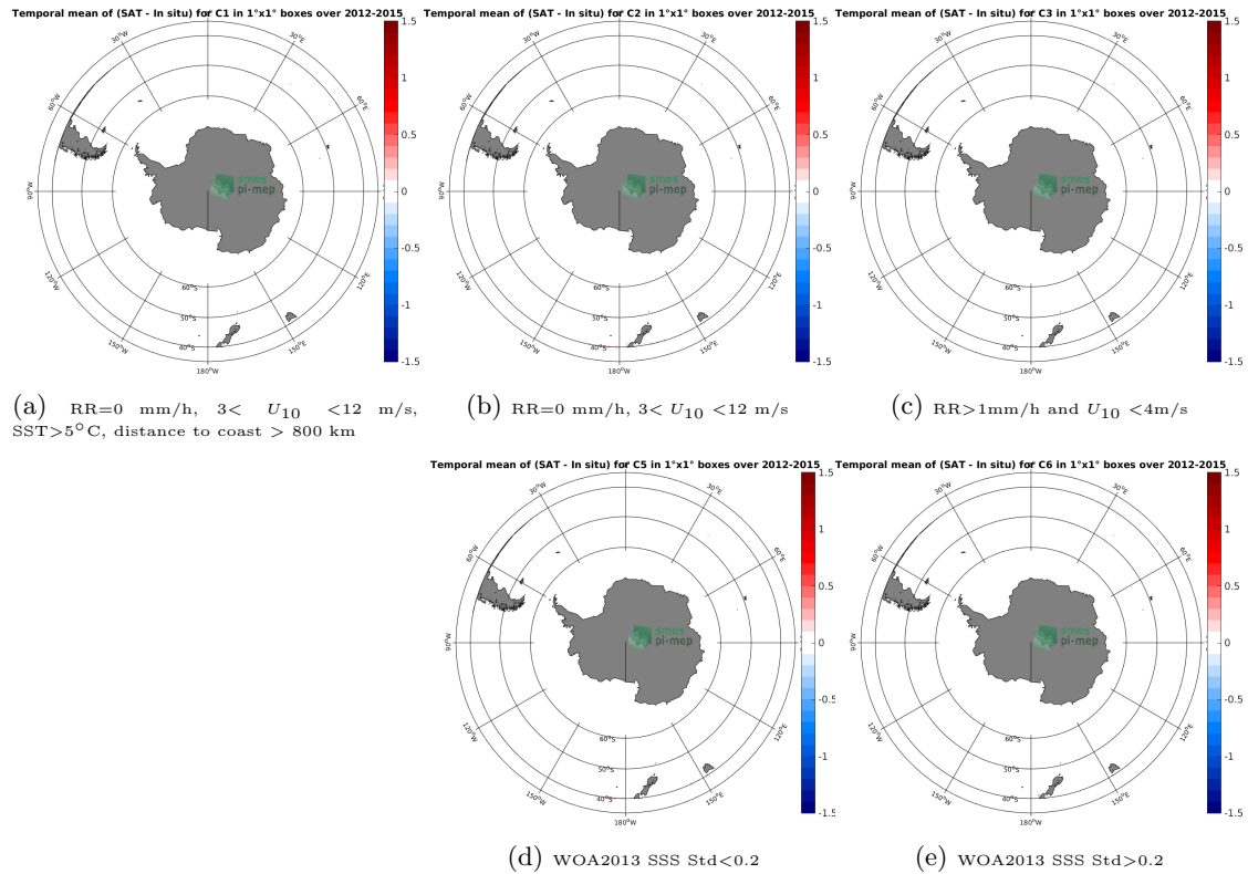
Figure 12: Temporal mean gridded over spatial boxes of size 1^{\circ}\times 1^{\circ} of \Delta\text{SSS} (Aquarius-L4-IPRC-V5-MONTHLY - TSG-LEGOS-DM) for 5 different subdatasets corresponding to:RR=0 mm/h, 3 < U_{10} < 12 m/s, SST > 5^{\circ}\text{C} , distance to coast > 800 km (a), RR=0 mm/h, 3 < U_{10} < 12 m/s (b), RR > 1 mm/h and U_{10} < 4 m/s (c), WOA2013 SSS Std < 0.2 (d), WOA2013 SSS Std > 0.2 (e).
