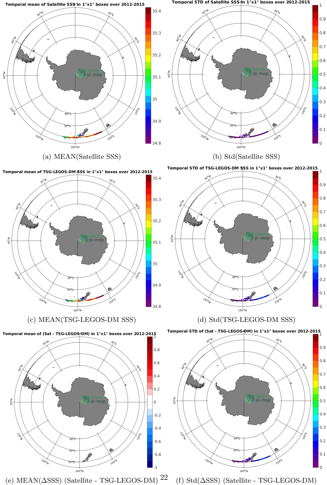
Figure 6: Temporal mean (left) and Std (right) of SSS from Aquarius-L4-IPRC-V5-MONTHLY (top), TSG-LEGOS-DM (middle), and of \Delta SSS (Satellite - TSG-LEGOS-DM). Only match-up pairs are used to generate these maps.
