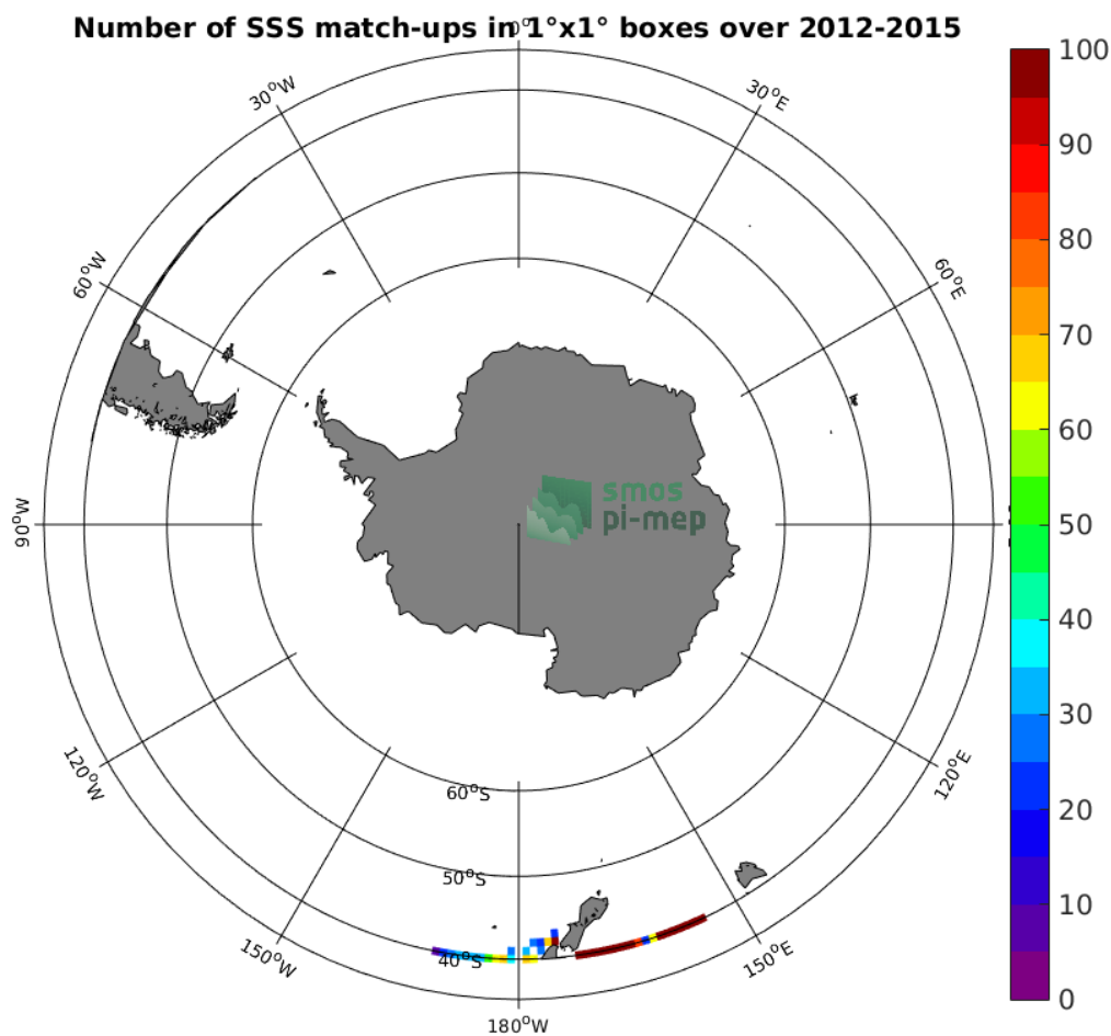
Figure 4: Number of SSS match-ups between TSG-LEGOS-DM SSS and the Aquarius-L4-IPRC-V5-MONTHLY SSS product for the Roaring Forties and Furious Fifties Pi-MEP region over 1°x1° boxes and for the full satellite product period.
