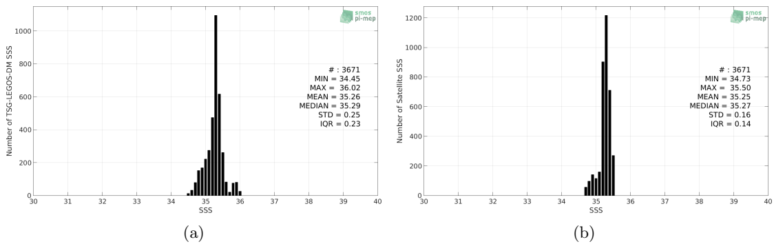
Figure 2: Histograms of SSS from TSG-LEGOS-DM (a) and Aquarius-L4-IPRC-V5-MONTHLY (b) considering all match-up pairs per bins of 0.1 over the Roaring Forties and Furious Fifties Pi-MEP region and for the full satellite product period.
