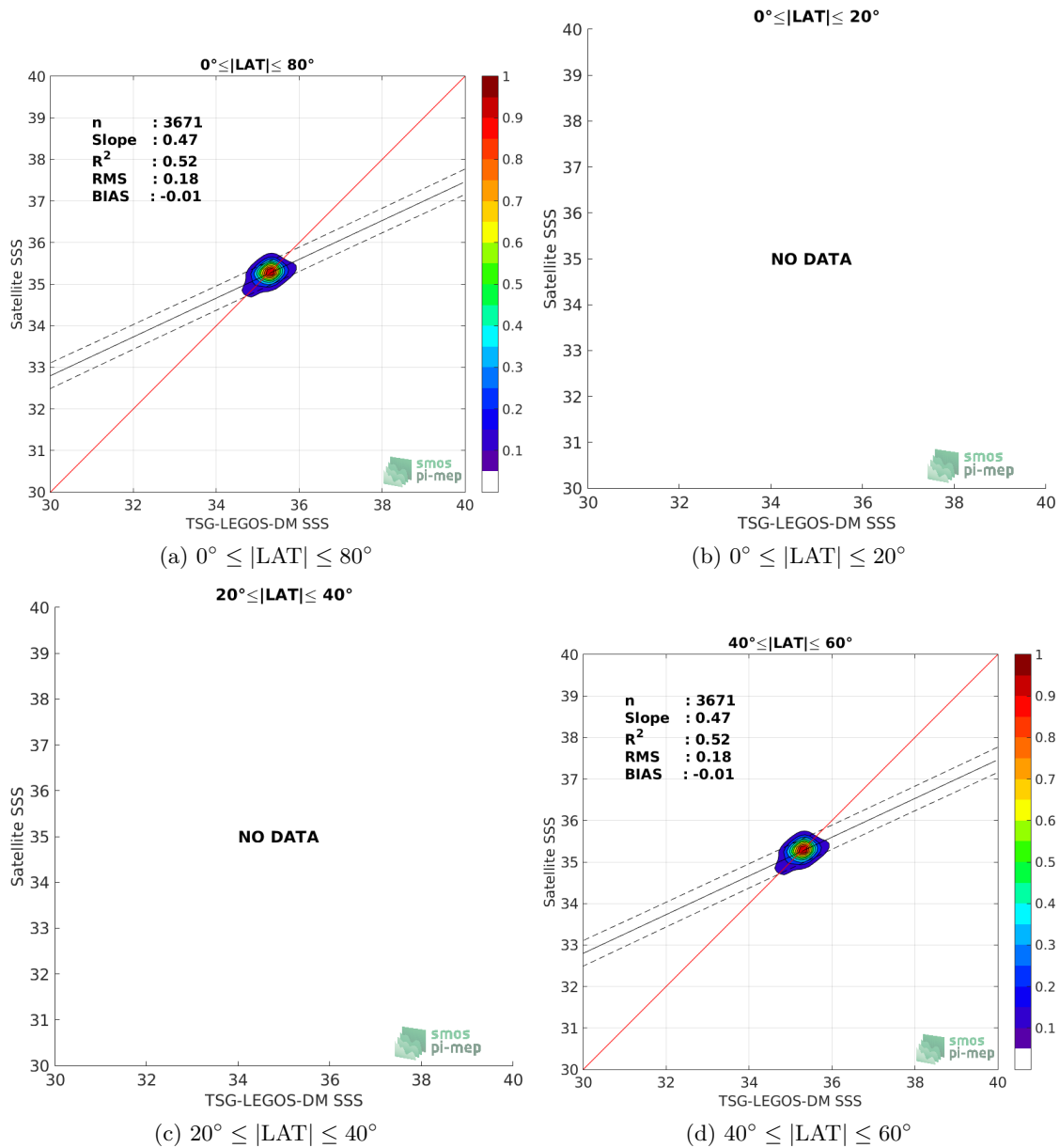
Figure 9: Contour maps of the concentration of Aquarius-L4-IPRC-V5-MONTHLY SSS (y-axis) versus TSG-LEGOS-DM SSS (x-axis) at match-up pairs for different latitude bands. For each plot, the red line shows x=y . The black thin and dashed lines indicate a linear fit through the data cloud and the \pm 95\% confidence levels, respectively. The number match-up pairs n , the slope and R^2 coefficient of the linear fit, the root mean square (RMS) and the mean bias between satellite and in situ data are indicated for each latitude band in each plots.
