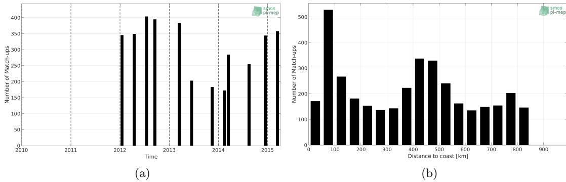
Figure 1: Number of match-ups between TSG-LEGOS-DM and Aquarius-L4-IPRC-V5-MONTHLY SSS as a function of time (a) and as function of the distance to coast (b) over the Roaring Forties and Furious Fifties Pi-MEP region and for the full satellite product period.
