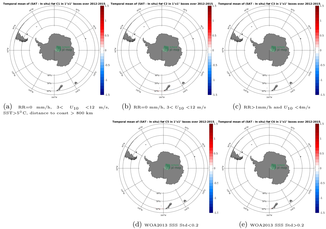
Figure 12: Temporal mean gridded over spatial boxes of size 1^\circ \times 1^\circ of \Delta SSS (Aquarius-L4-IPRC-V5-MONTHLY - TSG-LEGOS-DM) for 5 different subdatasets corresponding to:RR=0 mm/h, 3 < U_{10} < 12 m/s, SST > 5^\circ\text{C} , distance to coast > 800 km (a), RR=0 mm/h, 3 < U_{10} < 12 m/s (b), RR > 1 mm/h and U_{10} < 4 m/s (c), WOA2013 SSS Std < 0.2 (d), WOA2013 SSS Std > 0.2 (e).
