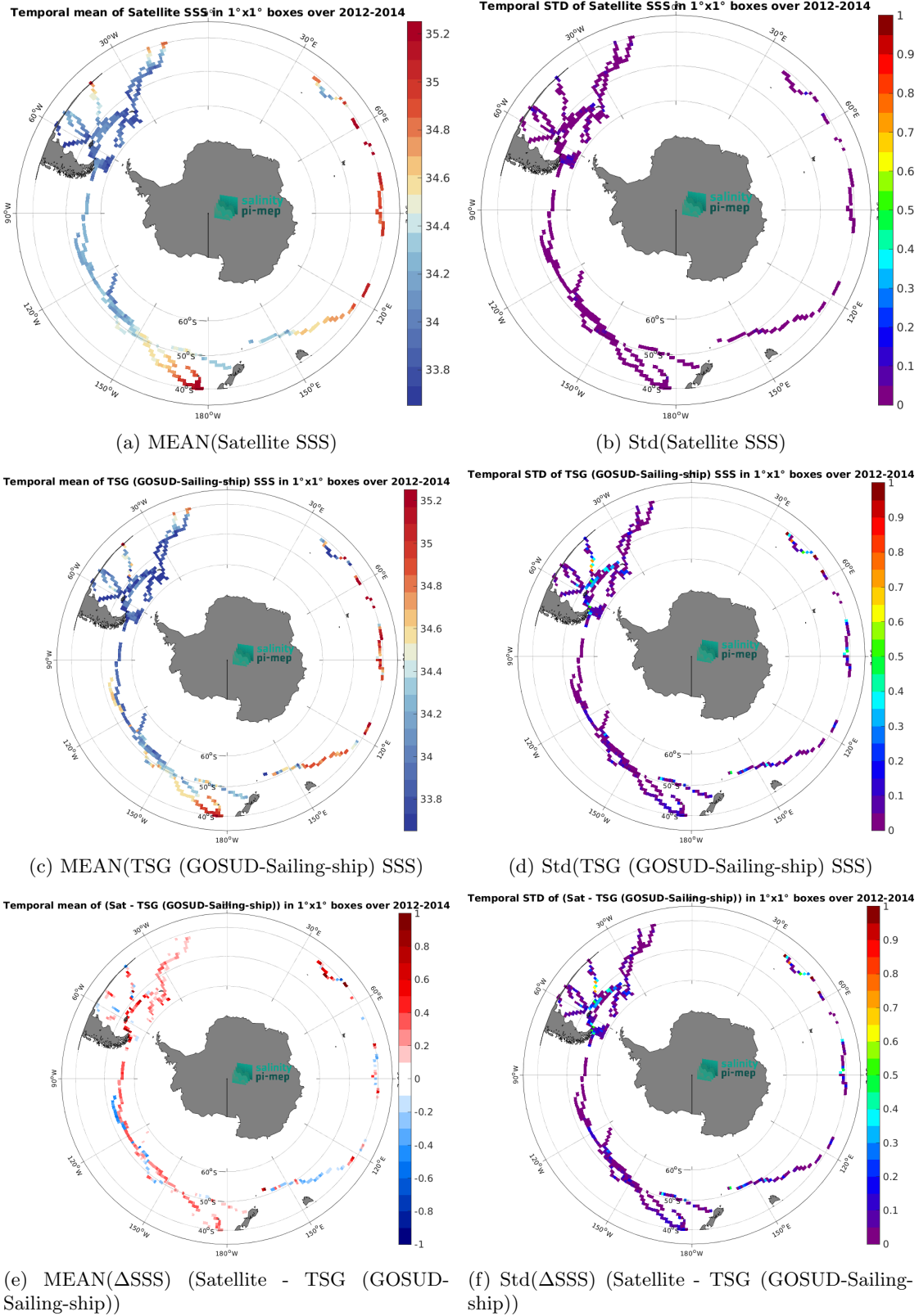
Figure 7: Temporal mean (left) and Std (right) of SSS from Aquarius SSS L4 OI v5 - Monthly (IPRC) (top), TSG (GOSUD-Sailing-ship) (middle), and of \Delta SSS (Satellite - TSG (GOSUD-Sailing-ship)). Only match-up pairs are used to generate these maps.
