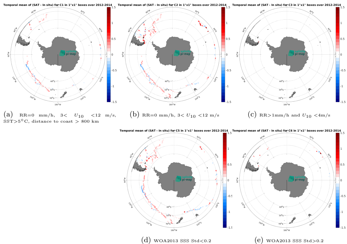
Figure 14: Temporal mean gridded over spatial boxes of size 1^\circ \times 1^\circ of \Delta SSS (Aquarius SSS L4 OI v5 - Monthly (IPRC) - TSG (GOSUD-Sailing-ship)) for 5 different subdatasets corresponding to: RR=0 mm/h, 3 < U_{10} < 12 m/s, SST > 5^\circ\text{C} , distance to coast > 800 km (a), RR=0 mm/h, 3 < U_{10} < 12 m/s (b), RR > 1 mm/h and U_{10} < 4 m/s (c), WOA2013 SSS Std < 0.2 (d), WOA2013 SSS Std > 0.2 (e).
