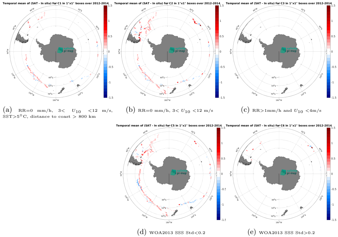
Figure 12: Temporal mean gridded over spatial boxes of size 1^{\circ} \times 1^{\circ} of \Delta SSS (Aquarius SSS L4 OI v5 - Monthly (IPRC) - TSG (GOSUD-Sailing-ship)) for 5 different subdatasets corresponding to: RR=0 mm/h, 3 < U_{10} < 12 m/s, SST > 5^{\circ}C , distance to coast > 800 km (a), RR=0 mm/h, 3 < U_{10} < 12 m/s (b), RR > 1 mm/h and U_{10} < 4 m/s (c), WOA2013 SSS Std < 0.2 (d), WOA2013 SSS Std > 0.2 (e).
