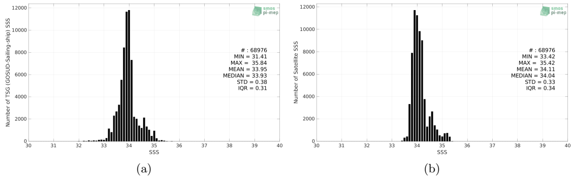
Figure 2: Histograms of SSS from TSG (GOSUD-Sailing-ship) (a) and Aquarius SSS L4 OI v5 - Monthly (IPRC) (b) considering all match-up pairs per bins of 0.1 over the Roaring Forties and Furious Fifties Pi-MEP region and for the full satellite product period.
