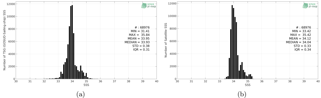
Figure 2: Histograms of SSS from TSG (GOSUD-Sailing-ship) (a) and Aquarius SSS L4 OI v5 - Monthly (IPRC) (b) considering all match-up pairs per bins of 0.1 over the Roaring Forties and Furious Fifties Pi-MEP region and for the full satellite product period.
