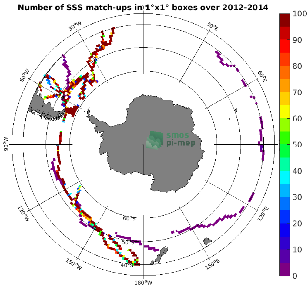
Figure 4: Number of SSS match-ups between TSG (GOSUD-Sailing-ship) SSS and the Aquarius SSS L4 OI v5 - Monthly (IPRC) SSS product for the Roaring Forties and Furious Fifties Pi-MEP region over 1^\circ \times 1^\circ boxes and for the full satellite product period.
