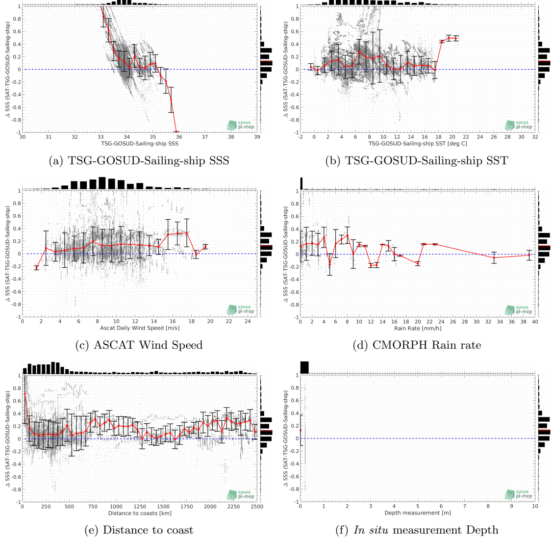
Figure 11: \Delta SSS (Satellite - TSG-GOSUD-Sailing-ship) sorted as function of TSG-GOSUD-Sailing-ship SSS values a), TSG-GOSUD-Sailing-ship SST b), ASCAT Wind speed c), CMORPH rain rate d), distance to coast (e) and in situ measurement depth (f). In all plots the median and Std of \Delta SSS for each bin is indicated by the red curves and black vertical thick bars ( \pm 1 Std)
