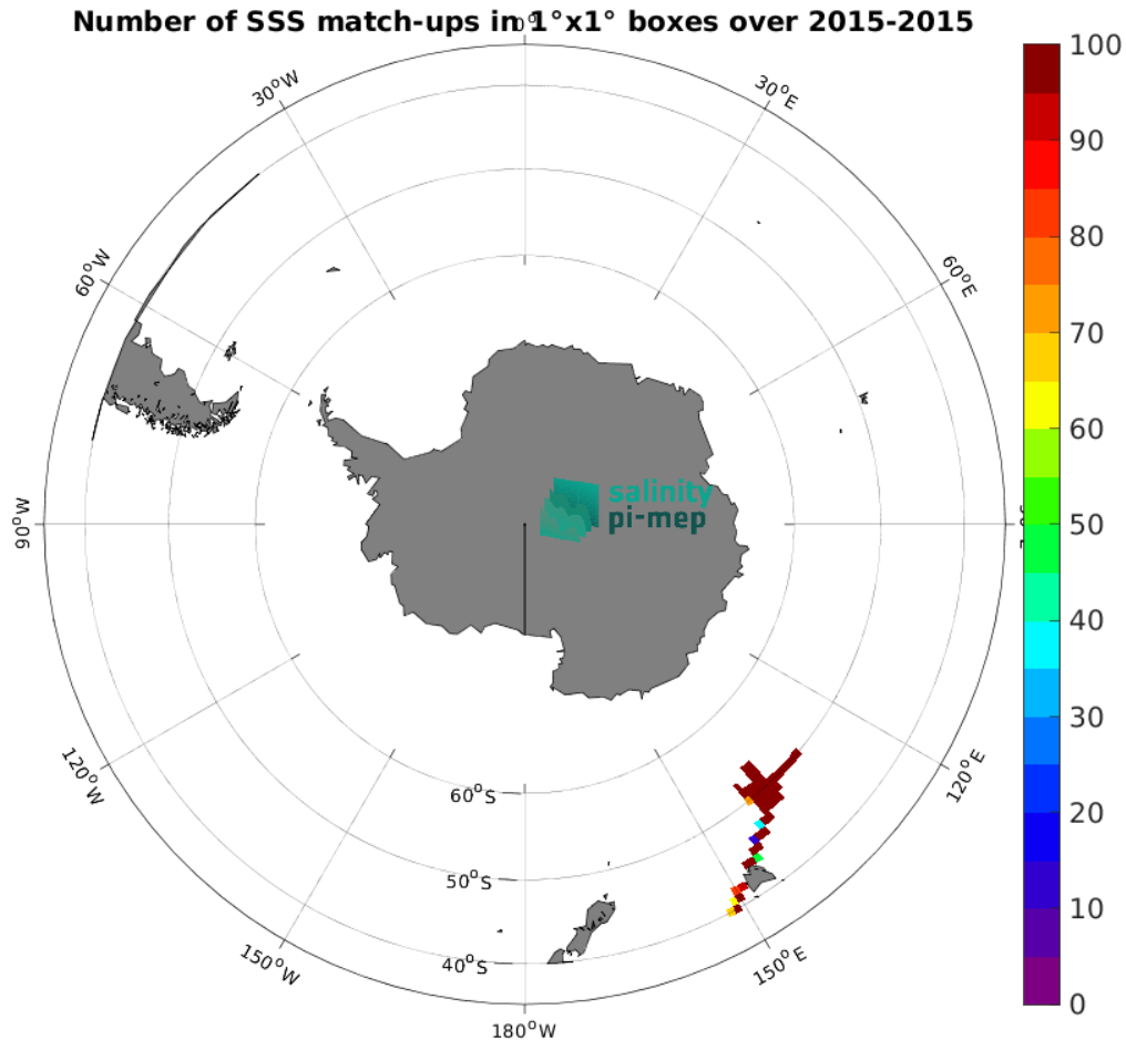
Figure 5: Number of SSS match-ups between TSG (GOSUD-Research-vessel) SSS and the Aquarius SSS L4 OI v5 - Monthly (IPRC) SSS product for the Roaring Forties and Furious Fifties Pi-MEP region over 1^\circ \times 1^\circ boxes and for the full satellite product period.
