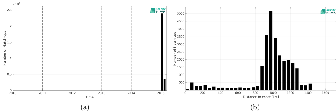
Figure 2: Number of match-ups between TSG (GOSUD-Research-vessel) and Aquarius SSS L4 OI v5 - Monthly (IPRC) SSS as a function of time (a) and as function of the distance to coast (b) over the Roaring Forties and Furious Fifties Pi-MEP region and for the full satellite product period.
