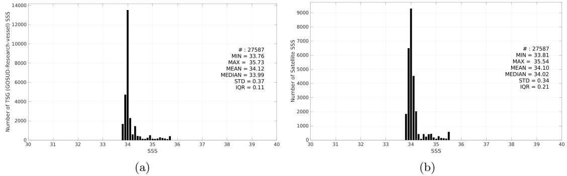
Figure 3: Histograms of SSS from TSG (GOSUD-Research-vessel) (a) and Aquarius SSS L4 OI v5 - Monthly (IPRC) (b) considering all match-up pairs per bins of 0.1 over the Roaring Forties and Furious Fifties Pi-MEP region and for the full satellite product period.
