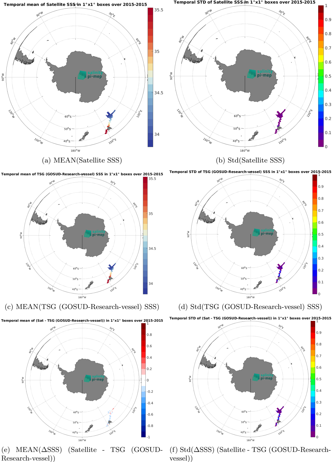
Figure 7: Temporal mean (left) and Std (right) of SSS from Aquarius SSS L4 OI v5 - Monthly (IPRC) (top), TSG (GOSUD-Research-vessel) (middle), and of \Delta SSS (Satellite - TSG (GOSUD-Research-vessel)). Only match-up pairs are used to generate these maps.
