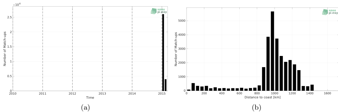
Figure 1: Number of match-ups between TSG (GOSUD-Research-vessel) and Aquarius SSS L4 OI v5 - Monthly (IPRC) SSS as a function of time (a) and as function of the distance to coast (b) over the Roaring Forties and Furious Fifties Pi-MEP region and for the full satellite product period.
