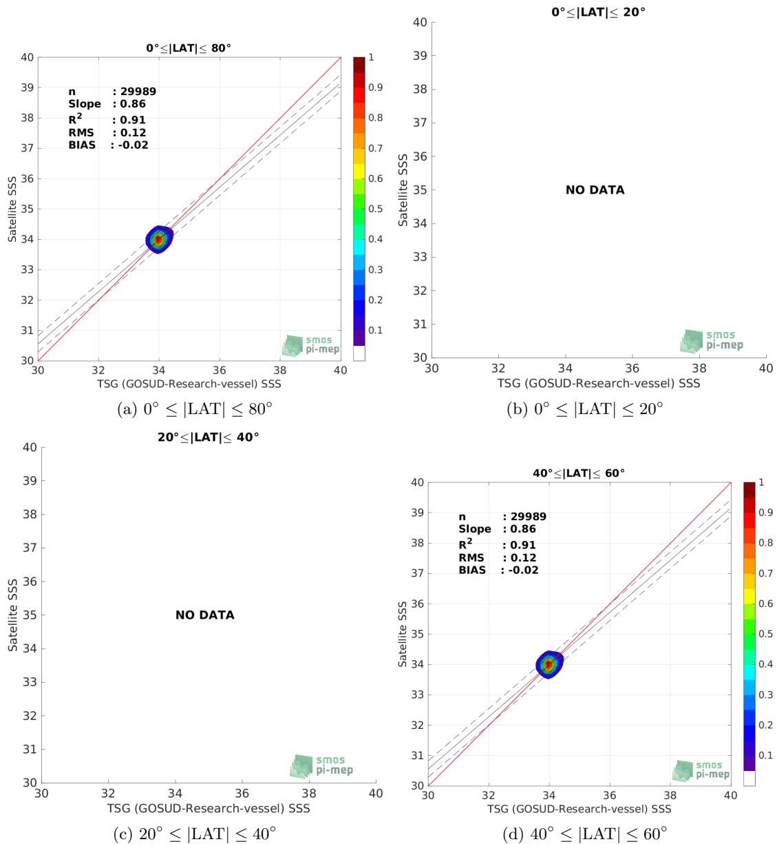
Figure 9: Contour maps of the concentration of Aquarius SSS L4 OI v5 - Monthly (IPRC) SSS (y-axis) versus TSG (GOSUD-Research-vessel) SSS (x-axis) at match-up pairs for different latitude bands. For each plot, the red line shows x=y . The black thin and dashed lines indicate a linear fit through the data cloud and the \pm 95\% confidence levels, respectively. The number match-up pairs n , the slope and R^2 coefficient of the linear fit, the root mean square (RMS) and the mean bias between satellite and in situ data are indicated for each latitude band in each plots.
