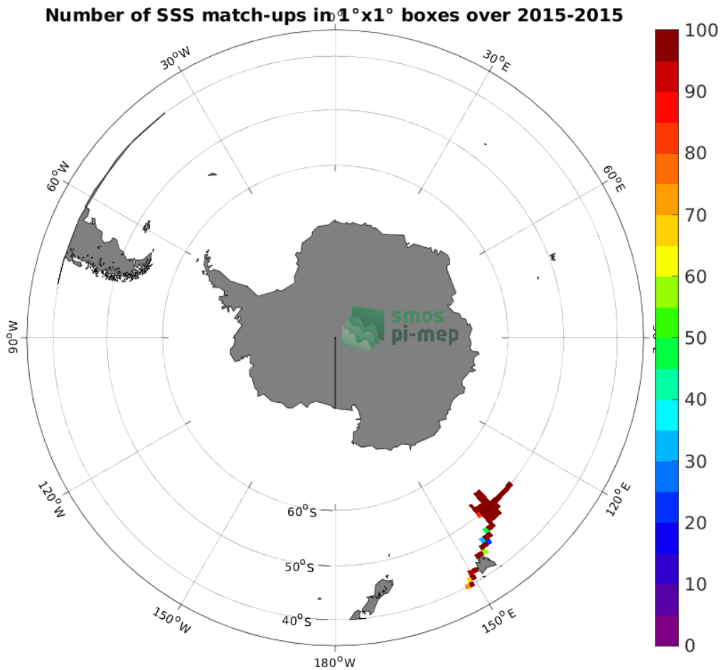
Figure 4: Number of SSS match-ups between TSG (GOSUD-Research-vessel) SSS and the Aquarius SSS L4 OI v5 - Monthly (IPRC) SSS product for the Roaring Forties and Furious Fifties Pi-MEP region over 1^\circ \times 1^\circ boxes and for the full satellite product period.
