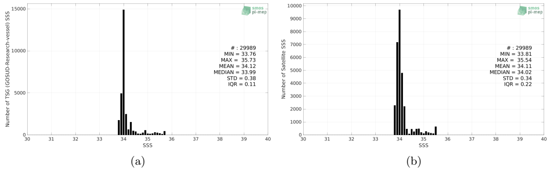
Figure 2: Histograms of SSS from TSG (GOSUD-Research-vessel) (a) and Aquarius SSS L4 OI v5 - Monthly (IPRC) (b) considering all match-up pairs per bins of 0.1 over the Roaring Forties and Furious Fifties Pi-MEP region and for the full satellite product period.
