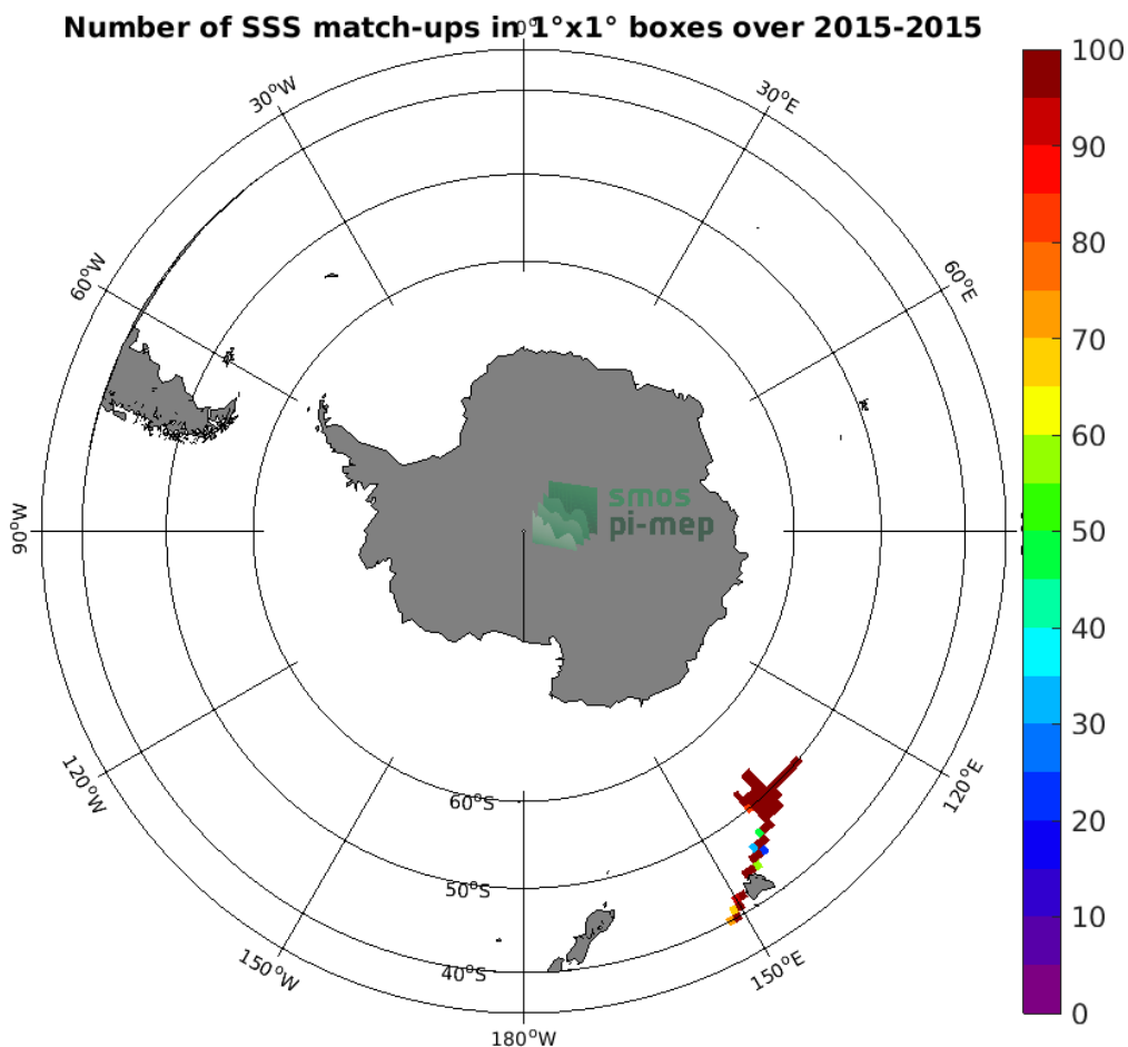
Figure 4: Number of SSS match-ups between TSG (GOSUD-Research-vessel) SSS and the Aquarius SSS L4 OI v5 - Monthly (IPRC) SSS product for the Roaring Forties and Furious Fifties Pi-MEP region over 1°x1° boxes and for the full satellite product period.
