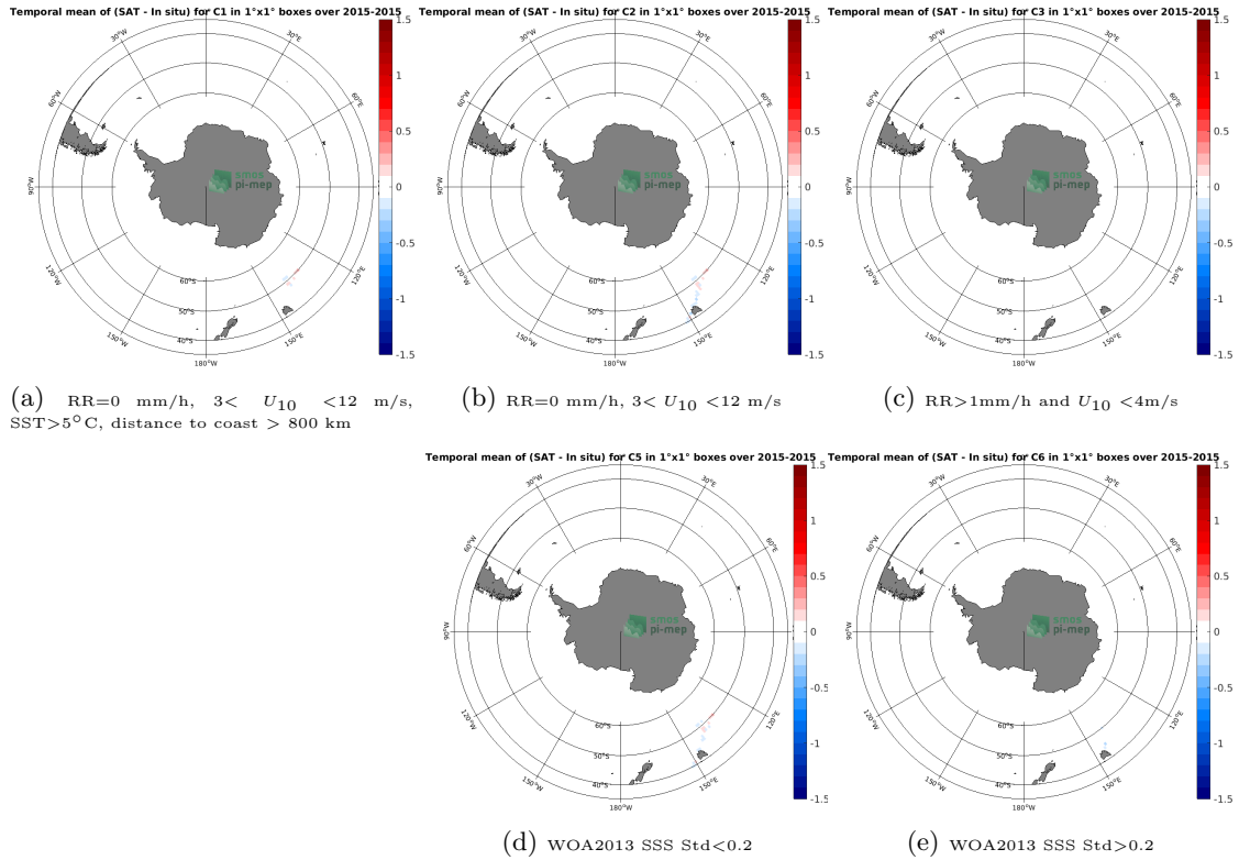
Figure 12: Temporal mean gridded over spatial boxes of size 1°x1° of \Delta SSS (Aquarius SSS L4 OI v5 - Monthly (IPRC) - TSG (GOSUD-Research-vessel)) for 5 different subdatasets corresponding to:RR=0 mm/h, 3 < U_{10} < 12 m/s, SST>5°C, distance to coast > 800 km (a), RR=0 mm/h, 3 < U_{10} < 12 m/s (b), RR>1mm/h and U_{10} < 4 m/s (c), WOA2013 SSS Std<0.2 (d), WOA2013 SSS Std>0.2 (e).
