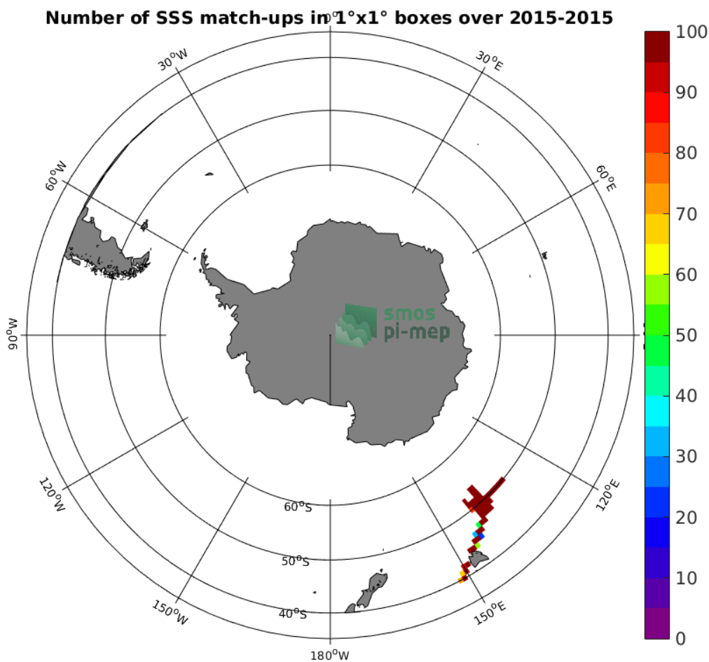
Figure 4: Number of SSS match-ups between TSG-GOSUD-Research-vessel SSS and the Aquarius-L4-IPRC-V5-MONTHLY SSS product for the Roaring Forties and Furious Fifties Pi-MEP region over 1°x1° boxes and for the full satellite product period.
